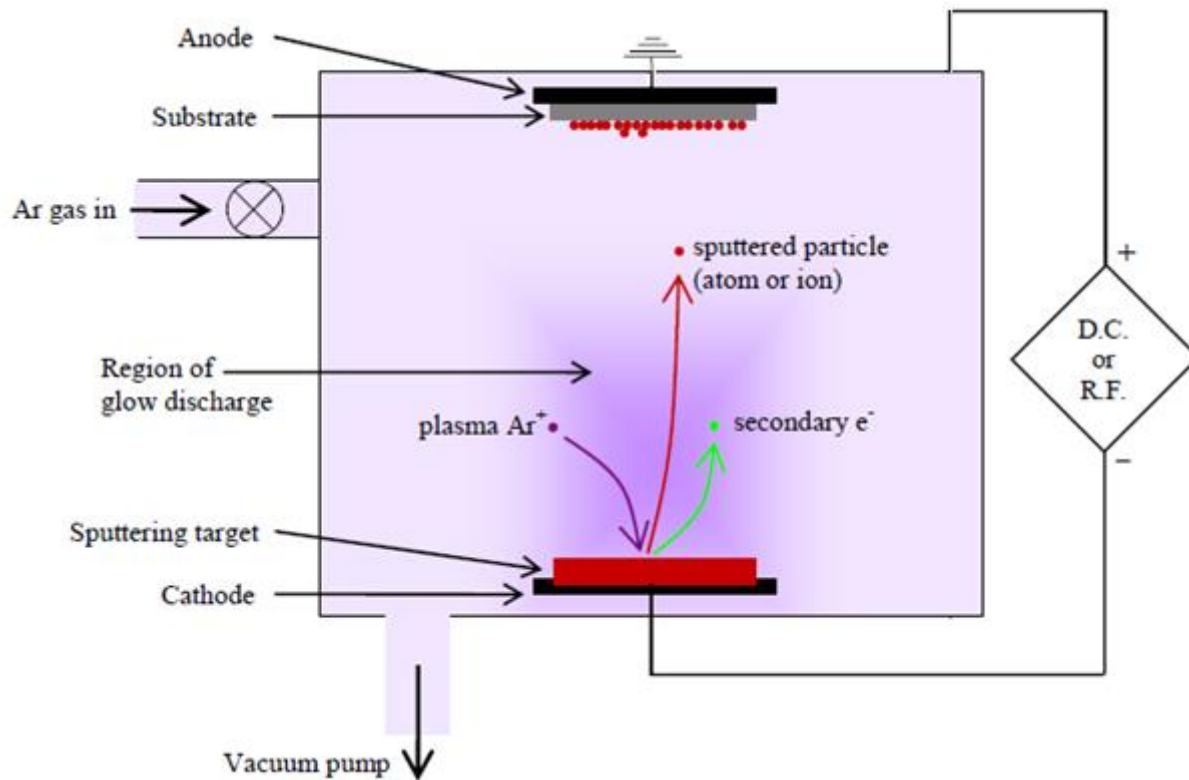
Figure 2.11: Schematic of the process of sputter deposition with Ar gas in a UHV chamber illustrating the glow discharge [32].
