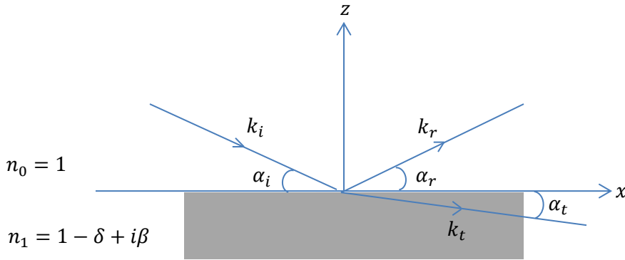
Figure 2.16: Schematic diagram showing the path of incident X-ray beam on a sample. X-rays are totally externally reflected when the angle of incidence is less than the critical angle. It is assumed that they undergo elastic scattering.
