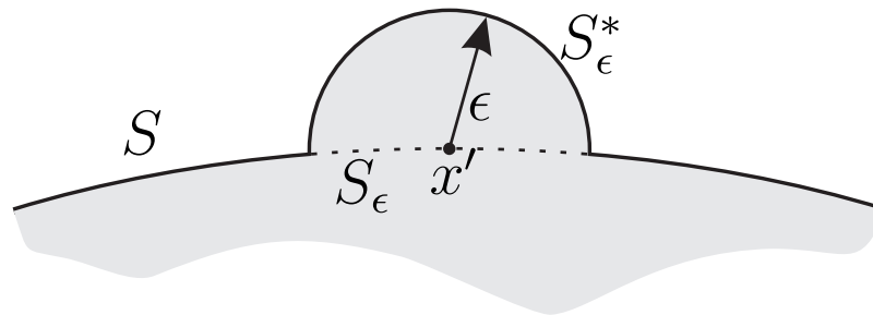
Figure 4.3: Semi-circular added domain on the boundary
