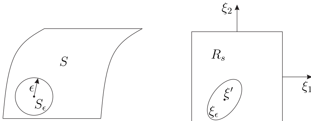
Figure 4.12: limiting procedure for three-dimensional problems
