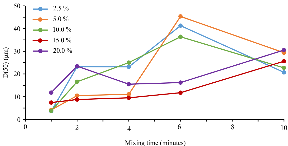
FIGURE 6.15: Graph showing the median granule size, D(50), as a function of granulation time for granules comprising spherical ATO nanoparticles and 2.5 %, 5.0 %, 10.0 %, 15.0 % and 20.0 % silicone binder.
