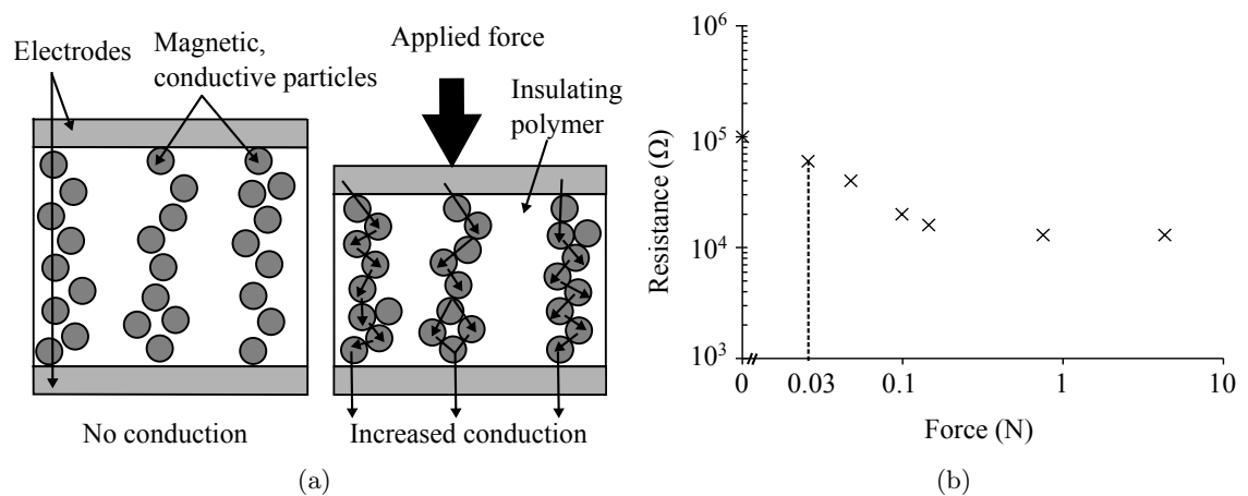
FIGURE 2.7: (a) Schematic of conducting polymer composite layer comprising columns of conductive, magnetic particles aligned through the application of an external magnetic field. Under applied force the composite compresses and the number of conductive pathways through the columns increase and field-assisted quantum tunnelling between particles may occur, causing a decrease in resistance through the composite. (b) Force-resistance response of a pressure-sensitive resistive touchscreen, demonstrated by Goncalves et al. , redrawn from data provided in the patent application [76]. The resistance through the composite decreases by a factor of 10 for applied forces up to 1 N, beyond which the resistance remains almost constant. The activation force of 0.03 N is shown by the dashed line.
