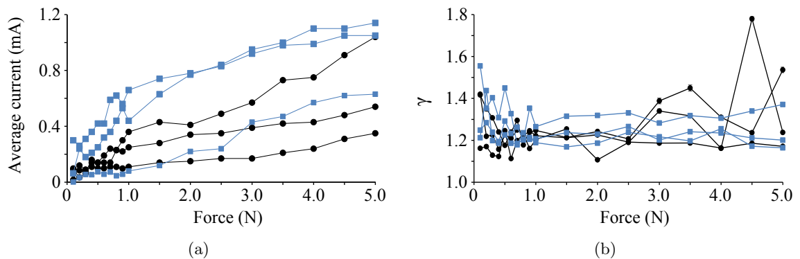
FIGURE 12.20: Graphs showing (a) the average current flow through each sensor and (b) the calculated \gamma value for each sensor, as a function of applied force. The black circles represent G3 sensors and the blue squares represent G4 sensors. Lines are drawn between data points as a guide to the eye.
