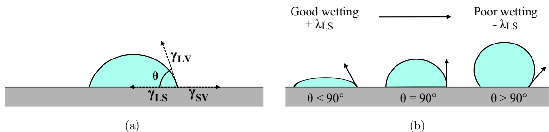
FIGURE 3.1: (a) Schematic showing a liquid droplet incident on a smooth, non-porous solid surface with a contact angle, \theta , between the solid and liquid phase. The surface free energy between the phases is given by \gamma , where the subscripts L , S and V denote the liquid, solid and vapour phases respectively (b) Good wetting occurs for \theta < 90^\circ and leads to a positive spreading coefficient, \lambda_{LS} , between liquid and solid. Poor wetting occurs for \theta > 90^\circ and this leads to a negative \lambda_{LS} .
