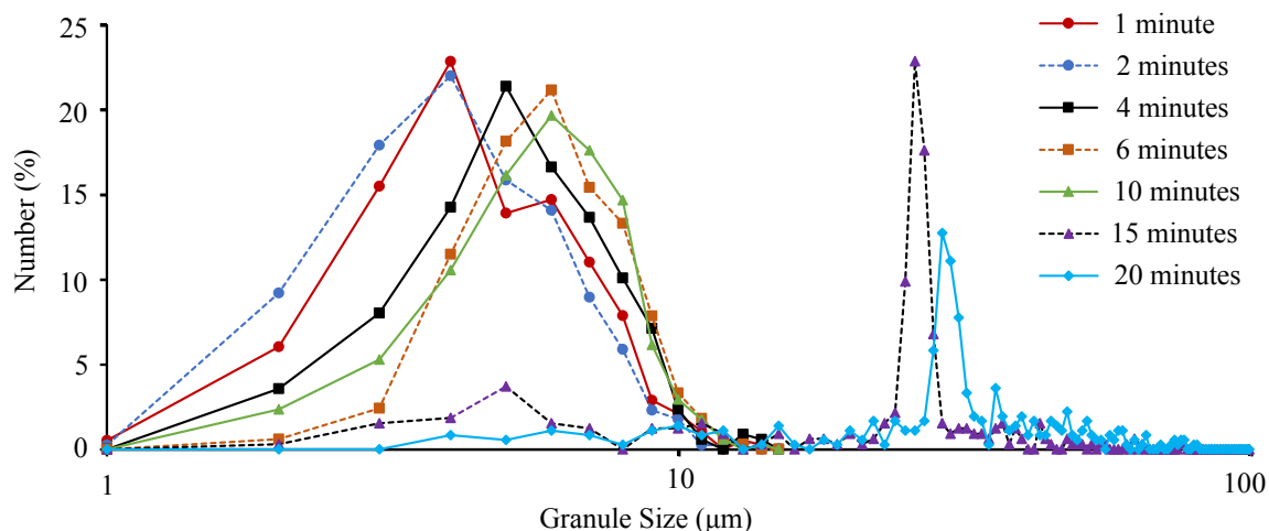
FIGURE 6.2: Graphs showing GSD for granules comprising spherical ATO particles and 10 % silicone binder, granulated at a speed of 2000 rpm for 1 to 20 minutes. Lines between data points are drawn as a guide to the eye.
