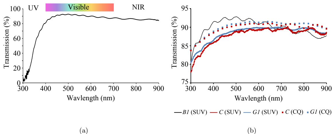
FIGURE 10.4: Graphs showing the transmission spectra for (a) substrate B1 over ultraviolet/visible/near infra-red wavelengths from 300–900 nm measured using the SUV spectrophotometer and (b) samples G1 and C measured using both CQ and SUV spectrophotometers, compared against substrate B1 measured using the SUV spectrophotometer.
