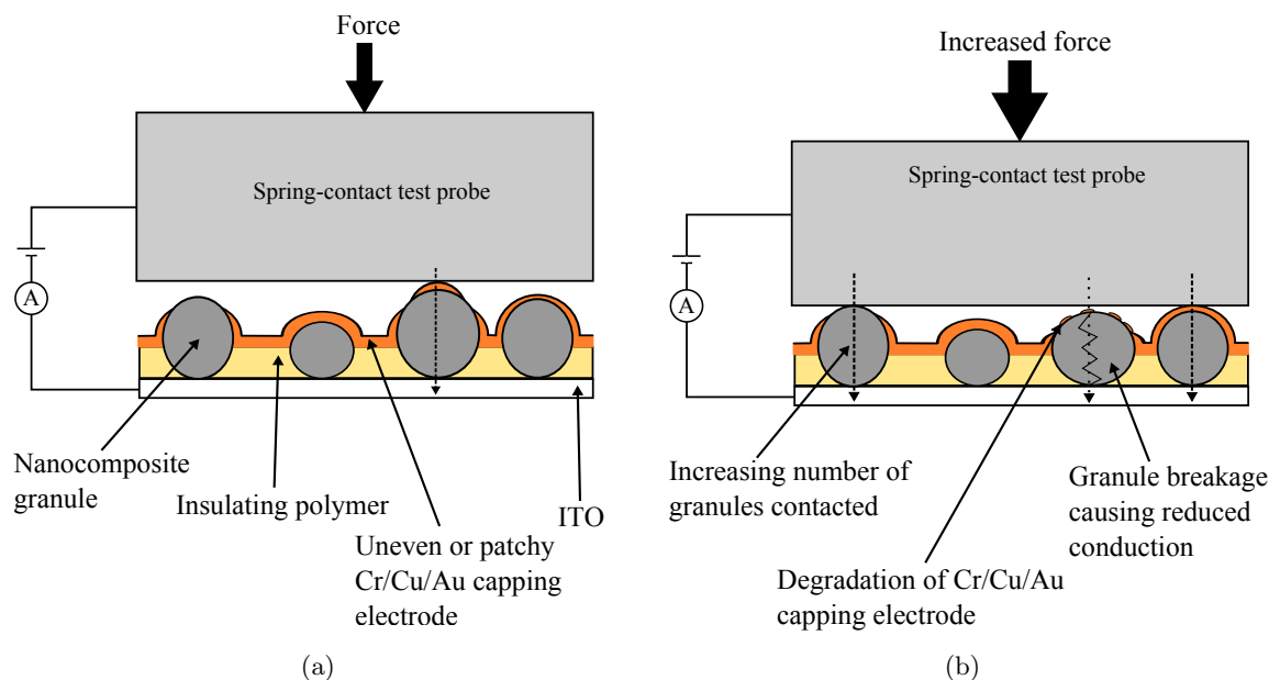
FIGURE 12.6: Schematics showing the complex interaction between the granules within the PS layer and the SCTP. In (a) initial contact is first created between the largest granule and the SCTP, and this granule is compressed first. The capping electrode may be uneven across the curved granule topography. In (b) increasing force increases the number of granules contacted and subsequently compressed by the SCTP, and may also cause degradation of the capping electrode.
