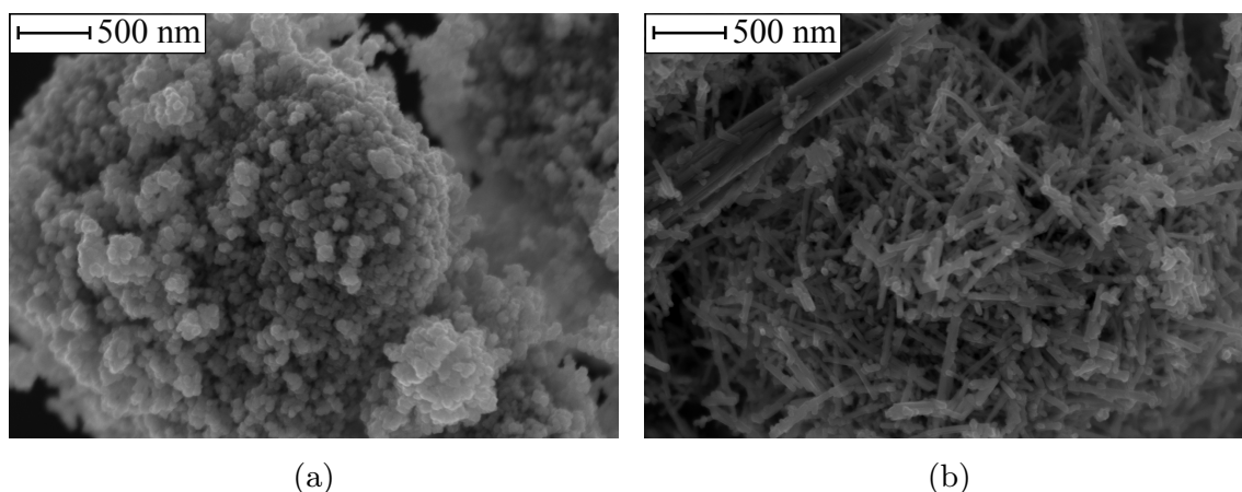
FIGURE 4.1: SEM images of (a) agglomerated spherical ATO nanoparticles of diameter 10–30 nm (b) acicular ATO nanoparticles of diameter 10–20 nm and length 0.2–2 \mu\text{m} .
