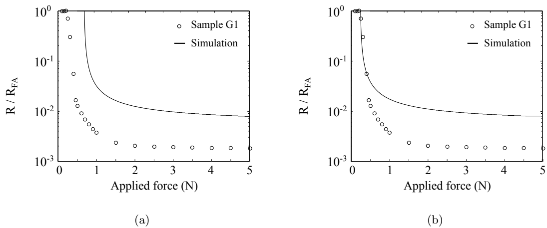
FIGURE 11.5: Graphs showing (a) the simulated force-resistance response for a PS layer with a granule concentration of 54 \text{ mm}^{-2} , where each granule has an arbitrarily assigned resistance of 1 \text{ M}\Omega (black line), compared against the F - R response of sample G1 (open circles) where the (normalised) resistance is expressed as a fraction of the resistance at the activation force. In (b), the simulation is adjusted to match the activation force F_A observed in sample G1 .
