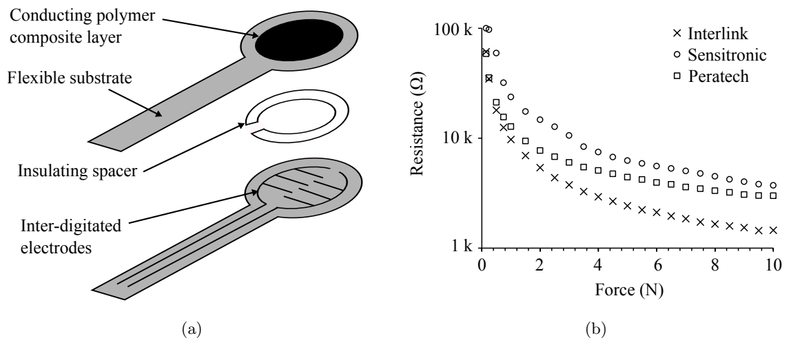
FIGURE 2.10: (a) Schematic of a Force Sensitive Resistor (FSR) comprising a conducting polymer composite layer printed onto a flexible substrate, separated from a set of interdigitated electrodes by an insulating spacer ring. When pressed, contact is made between the CPC layer and the electrodes. (b) Graph showing the force-resistance profile of three commercial FSR sensors sourced from Interlink Electronics, Sensitronic LLC and Peratech Holdco Ltd. For each FSR, the resistance decreases by over three orders of magnitude for up to 10 N applied force.
