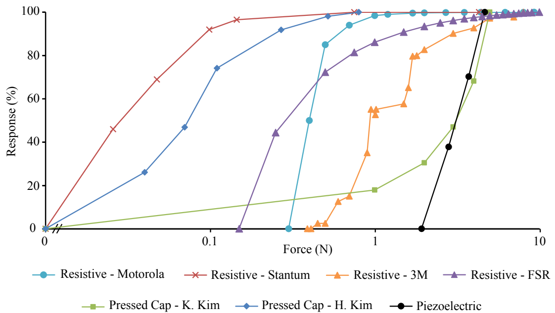
FIGURE 2.11: Force-sensitive response for all touch interfaces discussed in this chapter, including the piezoelectric sensor developed by Rendl et al. [46], the pressed capacitive sensors demonstrated by K. Kim et al. and H. Kim et al. [48, 50], the transparent resistive touchscreens patented by Motorola, Inc., Stantum and 3M Innovative Properties Company [75, 76, 81] and a force sensitive resistor commercialised by Interlink Electronics. Data points are connected by straight lines as a guide to the eye.
