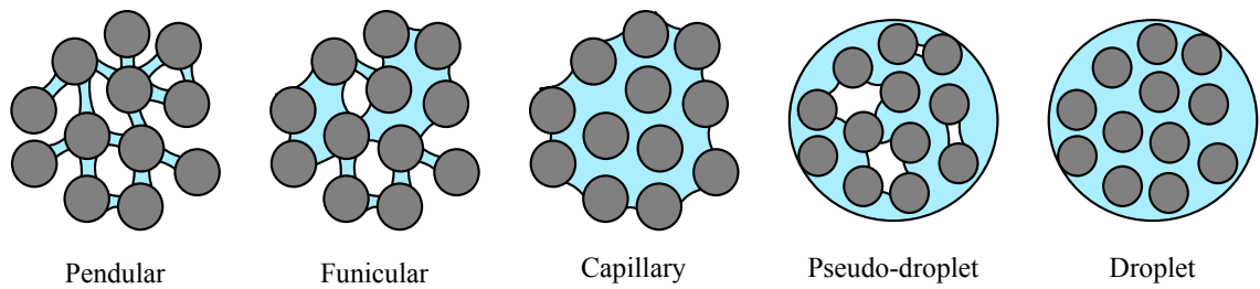
FIGURE 3.3: Schematic illustrations of the various states of liquid saturation within a granule as described by Newitt and Conway-Jones [108]
