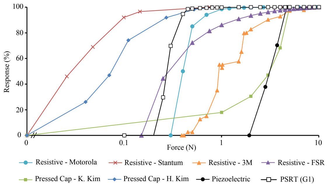
FIGURE 10.16: Graph showing the force sensitive response of the PSRT device comprising the PS layer G1 , compared against the response of other force sensing technologies described in chapter 2 of this thesis, including a piezoelectric sensor developed by PyzoFlex, pressed capacitive sensors developed by H. Kim and K. Kim, piezoresistive conducting polymer composites developed by Motorola, Stantum and 3M and force sensitive resistors developed by Interlink Electronics.
