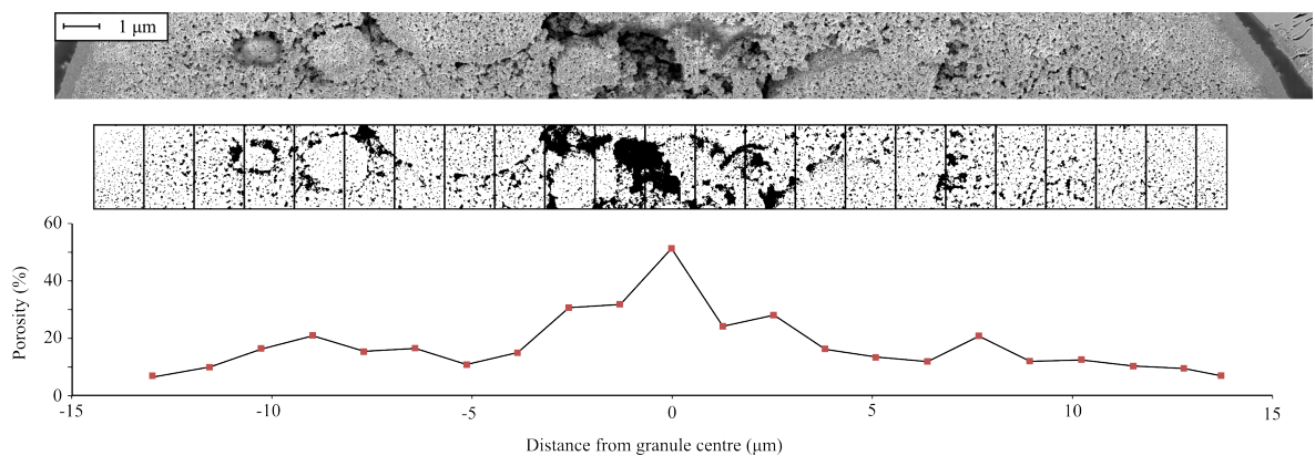
FIGURE 7.8: Porosity profile of a granule of Feret diameter 34 µm produced after 10 minutes, comprising a core of coalesced nuclei, areas of high binder content and large internal voids. The porosity reaches a peak value of 51.3 % at the granule centre, caused by a large internal void.
