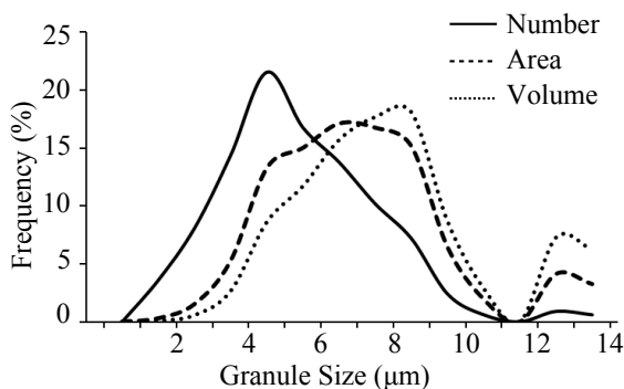
FIGURE 3.9: Granule size distributions calculated for same set of granules, where the frequency weighting by number, area and volume are compared. Area and volume weighting are biased towards larger granules compared to number weighting. For ease of comparison the lines show the envelope of the measured GSDs.
