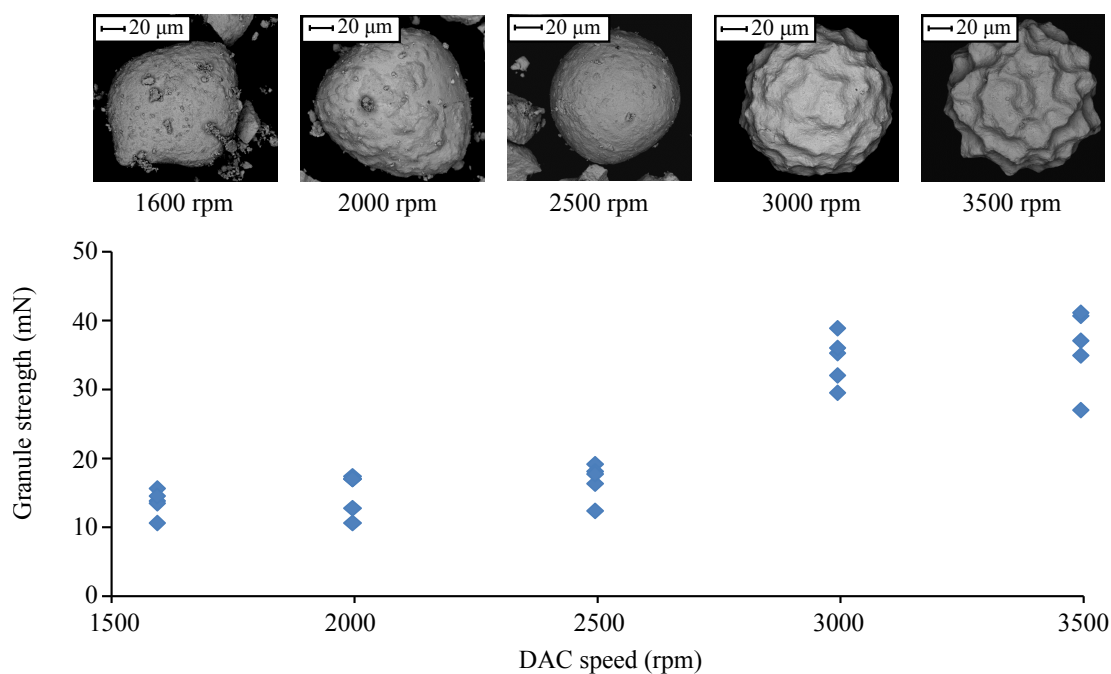
FIGURE 7.16: Graph showing the effect of DAC rotational speed on the fracture strength of granules in the size range 75–100 μm produced after 10 minutes. The insets show SEM images of representative granules produced at each speed.
