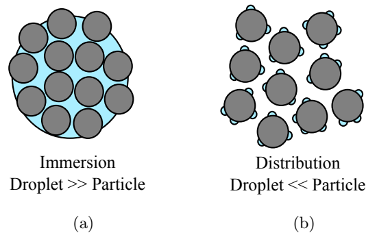
FIGURE 3.2: Schematic showing the immersion and distribution nucleation mechanisms first proposed by Schæfer and Mathieson [106]. (a) If the binder droplet size is much larger than the particle size then particles become immersed within the binder droplet. (b) If the binder droplet size is much smaller than the particle size then the droplets are distributed amongst the particles and adhere to the particle surfaces.
