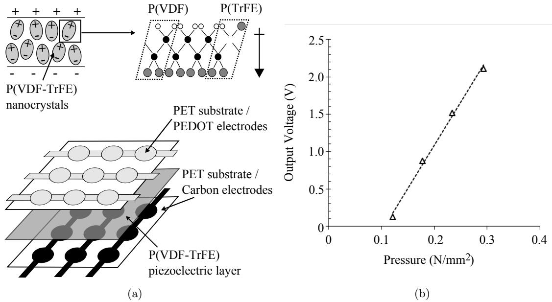
FIGURE 2.1: (a) Schematic of piezoelectric touch interface, comprising a piezoelectric layer containing P(VDF-TrFE) nanocrystals located between two electrode arrays. The left hand inset shows the alignment of nanocrystals within the film achieved through a poling process. The right hand inset shows the atomic arrangement within a nanocrystal, where the arrangement of carbon (black circles), fluorine (grey circles) and hydrogen (white circles) atoms creates a permanent dipole moment. (b) Graph showing the output voltage as a function of applied pressure for a piezoelectric sensor array, reproduced from data provided by Rendl et al. [46]. The output voltage is linearly dependent on the applied pressure in the range 0.12–0.29 N mm -2 .
