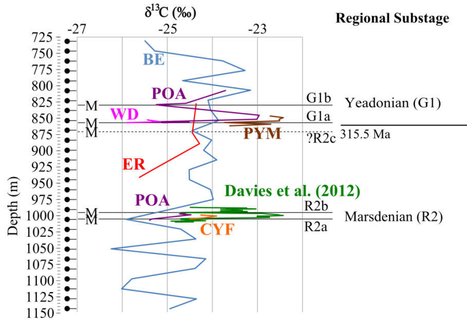
Figure 6-12: \delta^{13}\text{C} variations with depth and time. Depth is based on the Blacon East borehole (BE -blue line) which is the most continuous record of carbon isotope values available. Marine bands from the Holywell Shale allow correlation with other boreholes (Point of Ayr - purple and Erbistock - red) as well as outcrop locations from northeast Wales (Pen-Y-Maes = PYM - brown, Warren Dingle = WD - pink and Coed-Y-Felin = CYF - orange) and Yorkshire (Pule Hill; Davies et al., 2012).
