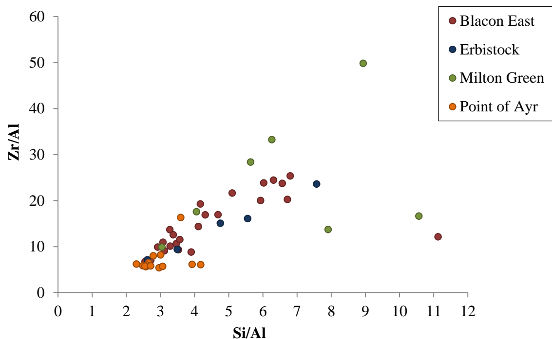
Figure 5-12: Silica and zirconium to aluminium ratios plotted to distinguish between biogenic and terrestrially sourced silica. Low Zr/Al indicates low terrestrial input, combined with high Si/Al indicates a biogenic source for the silica present.
