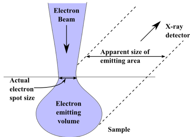
Figure 3-5: Interaction volume of the surface of a sample comparing electron beam spot size and the size of the area of emitted X-rays.
