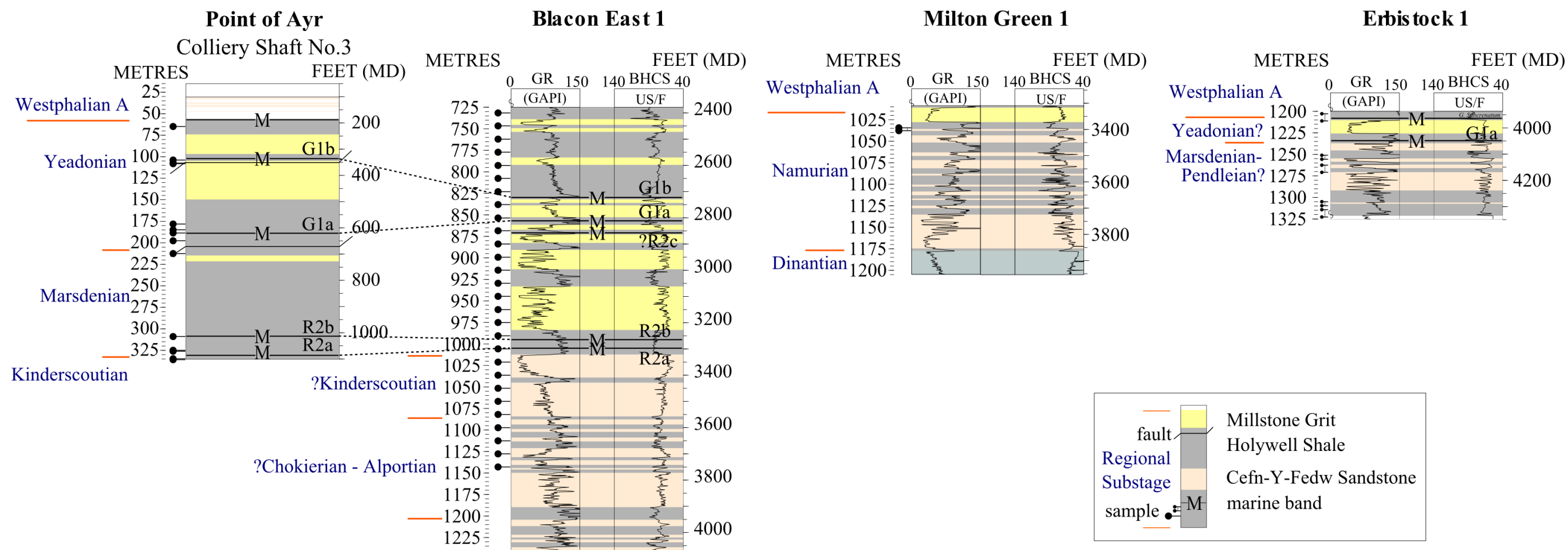
Figure 5-3: Log representation of all the boreholes used in this study across northeast Wales (Point of Ayr, Blacon East, Milton Green and Erbistock). Where possible, identified marine bands are labelled and correlated between Point of Ayr and Blacon East (dotted lines).
