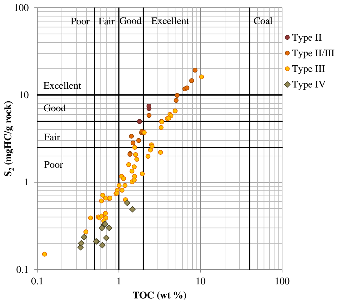
Figure 6-17: TOC versus S_2 (hydrocarbons formed from thermal decomposition of kerogen; from RockEval™). The higher the S_2 values the greater the potential for hydrocarbon generation. Samples are separated according to kerogen type (taken from Figure 6-16).
