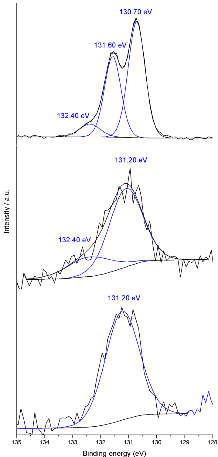
Figure 4.39: XPS spectra of the P(2p) region of i) [100] as a powder (top); ii) [100]-SAM (middle), still showing the characteristic P(2p) energy band of PPh 3 at 132.40 eV (FWHM values for the two bands at 131.20 and 132.40 eV are comparable), and iii) after annealing [100]-SAM for two hours at 150 °C (bottom), where the P(2p) energy band of PPh 3 could not be calculated.
