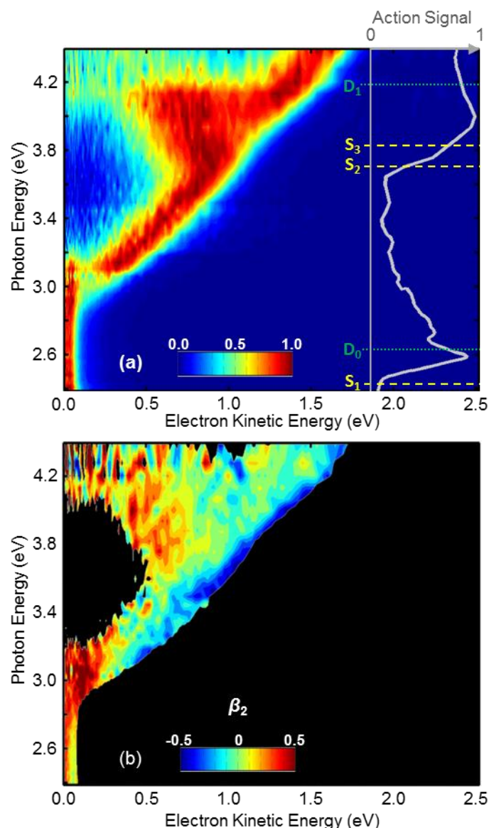
Figure 4.3 Frequency- and angle-resolved PE spectra of HBD \Gamma . The complete set of peak-normalised PE spectra is shown in (a), together with the action spectrum and calculated energies, taken from reference 34 . The PE anisotropy parameters are shown in (b).
