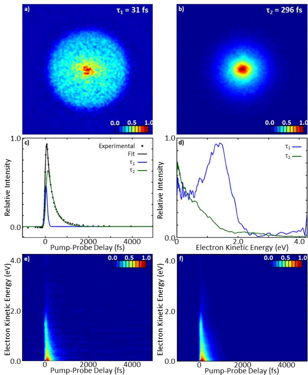
Figure 3.2 The results of the global kinetic fit of the time-resolved image series of dAMP^- assuming sequential dynamics. a-b) The normalised images associated with the decay lifetimes \tau_1 = 31 fs and \tau_2 = 296 fs respectively. c) The integrated time-resolved PE signal (black dots), the fit to the experimental data (black line) and the relative contributions from the decay lifetimes, S_i(eKE, t) . d) The decay associated spectra obtained from POP analysis of the decay associated images. e-f) The background subtracted and normalised time-resolved PE spectrum and the obtained fit to the spectrum respectively.
