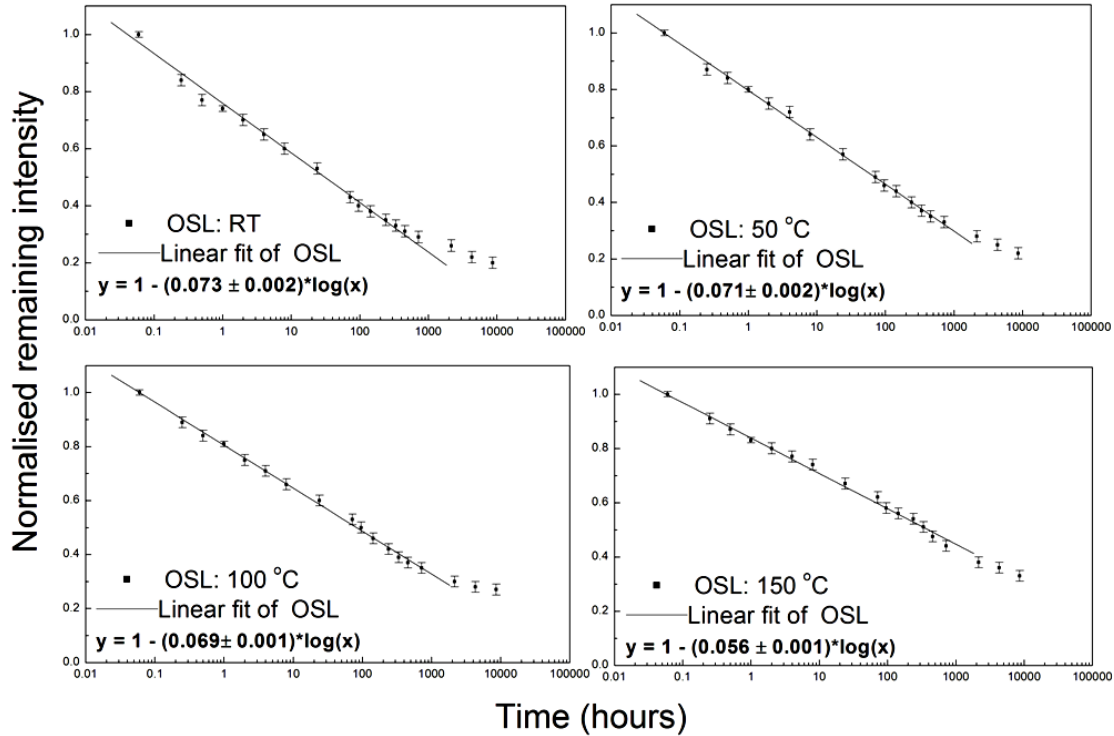
Figure 10.6: Comparison of fading curves of OSL at several sample measurement temperatures following irradiation with 3 Gy and preheat to 120 °C (10 s). The data points from t = t_0 ( t_0 \approx 1 -3 minutes) to t \approx 3 months were fitted with the equation describing the quantum mechanical tunnelling fading mechanism. Note that the rate of fading expressed by the constant b decreases with increasing sample temperature.
