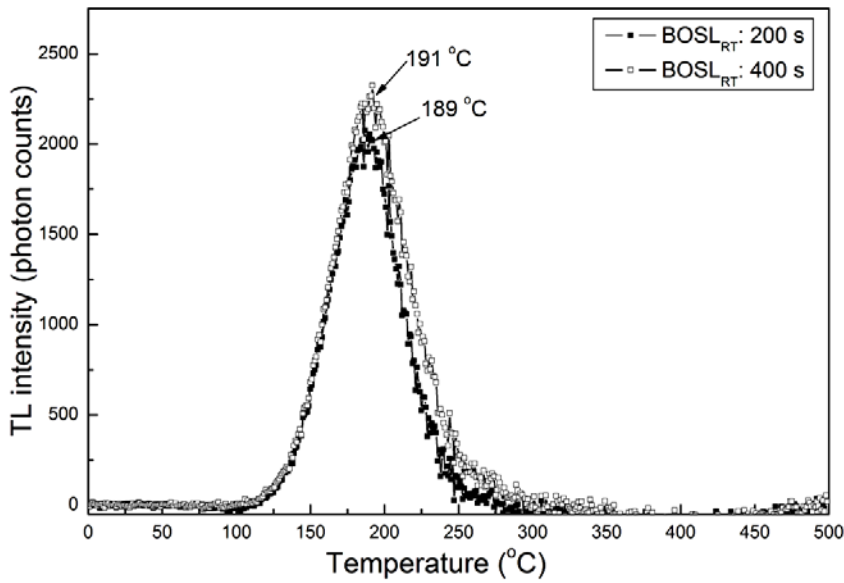
Figure 9.8: Lost TL glow curves following annealing to 120 °C and bleaching with blue light at RT for 200 and 400 s. The position of the maximum of each lost glow peak is also indicated in the figure. The glow curves are representative of a sample consisting of ~ 20 type ‘0402’ SMRs irradiated with ~ 10 Gy.
