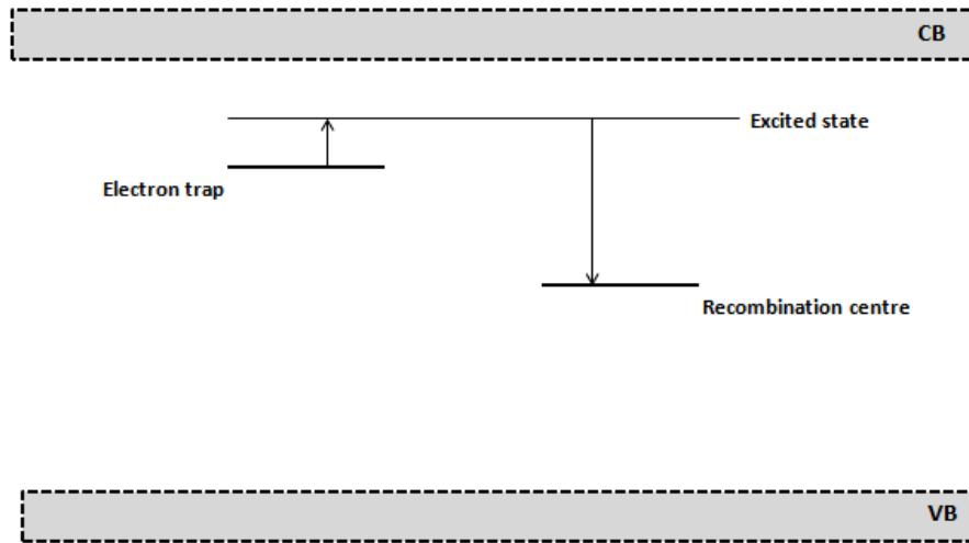
Figure 2.11: Localised transition model of anomalous fading. The electron trap and the recombination centre have a common excited state through which phonon-assisted excited electrons reach the ground state of the recombination centre.
