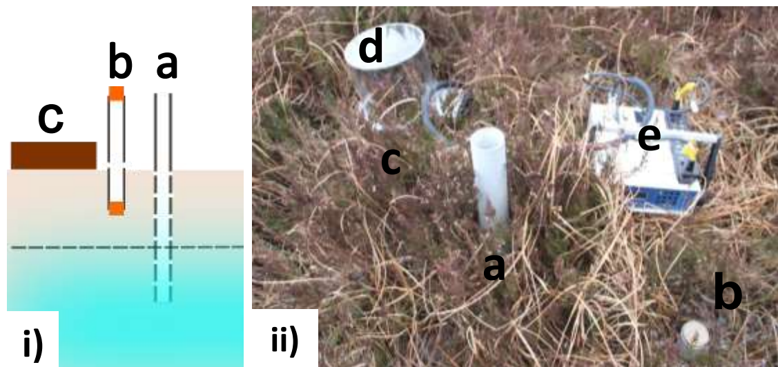
Figure 2.6: i) cross section diagram of sets of equipment displaying instrumentation relative to the peat surface and the water table. ii) Example an experimental plot. The Lettering on both i) and ii) represent the following: a) dipwell b) runoff trap (present at the Goyt Valley study sites) c) gas collar d) gas chamber e) Infra-red gas analyser (IRGA).
