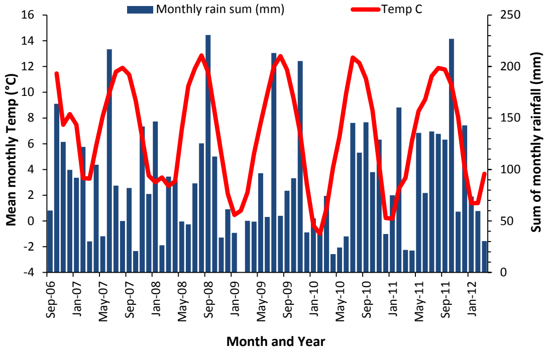
Figure 3.3: Monthly sum rainfall (mm) and mean daily temperature (°C) (2006 – 2012). Precipitation data are derived from both the MU AWS and the Defra UK-AIR data.
