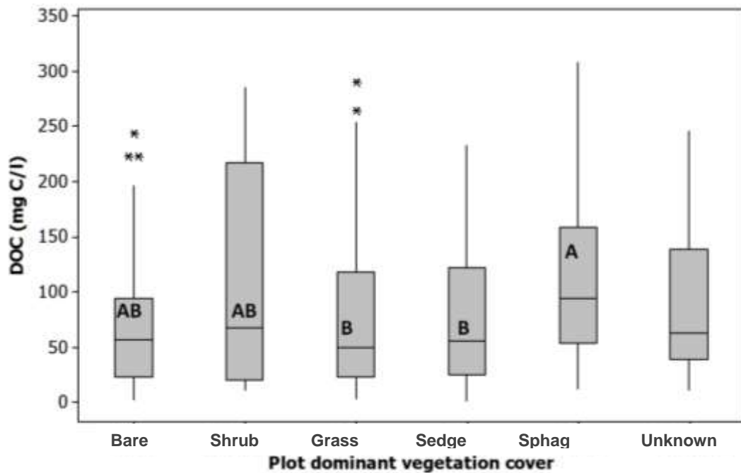
Figure 3.14: Box plot of DOC (2008) by most dominant vegetation cover. The ANCOVA includes: factors (site and month) and covariate air mean temperature of month prior to sampling. The letters signify post hoc tukey test results, whereby the means that do not share a letter are significantly different.
