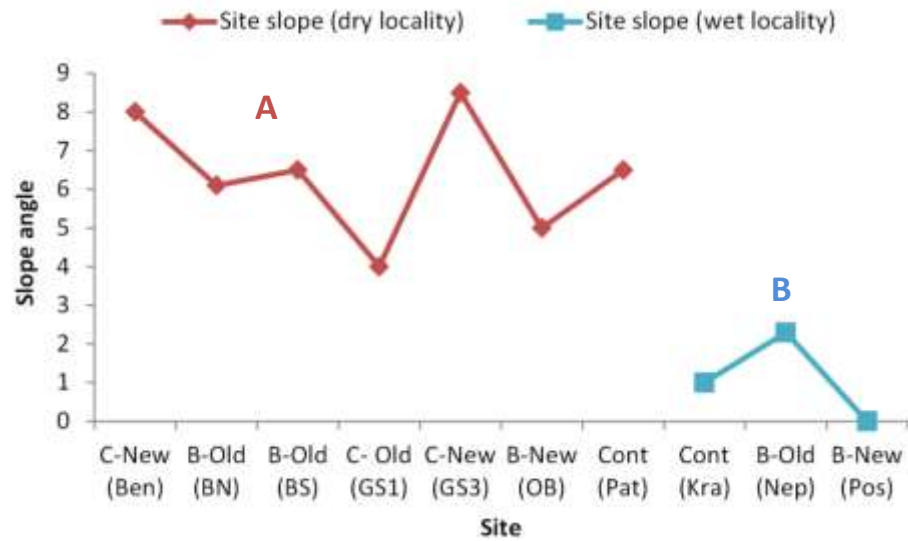
Figure 5.5: Goyt sites slope angle (red, dry locality, blue, wet locality). There are no error bars as no replicate measures were taken. The letters represent the results of an ANOVA tukey post hoc test; they indicate the significant difference between the locality levels (wet and dry).
