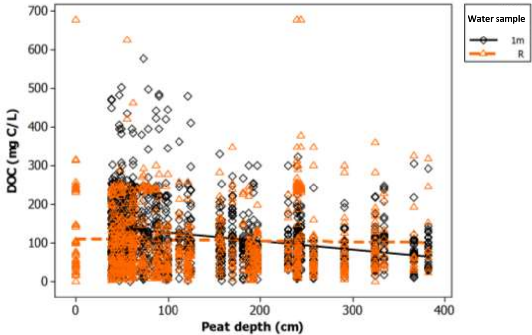
Figure 5.17: Goyt Valley runoff (R, brown triangles) and soil pore water (1m, black diamonds) sample DOC concentration plotted against site peat depth (May 2008 – April 2013).
