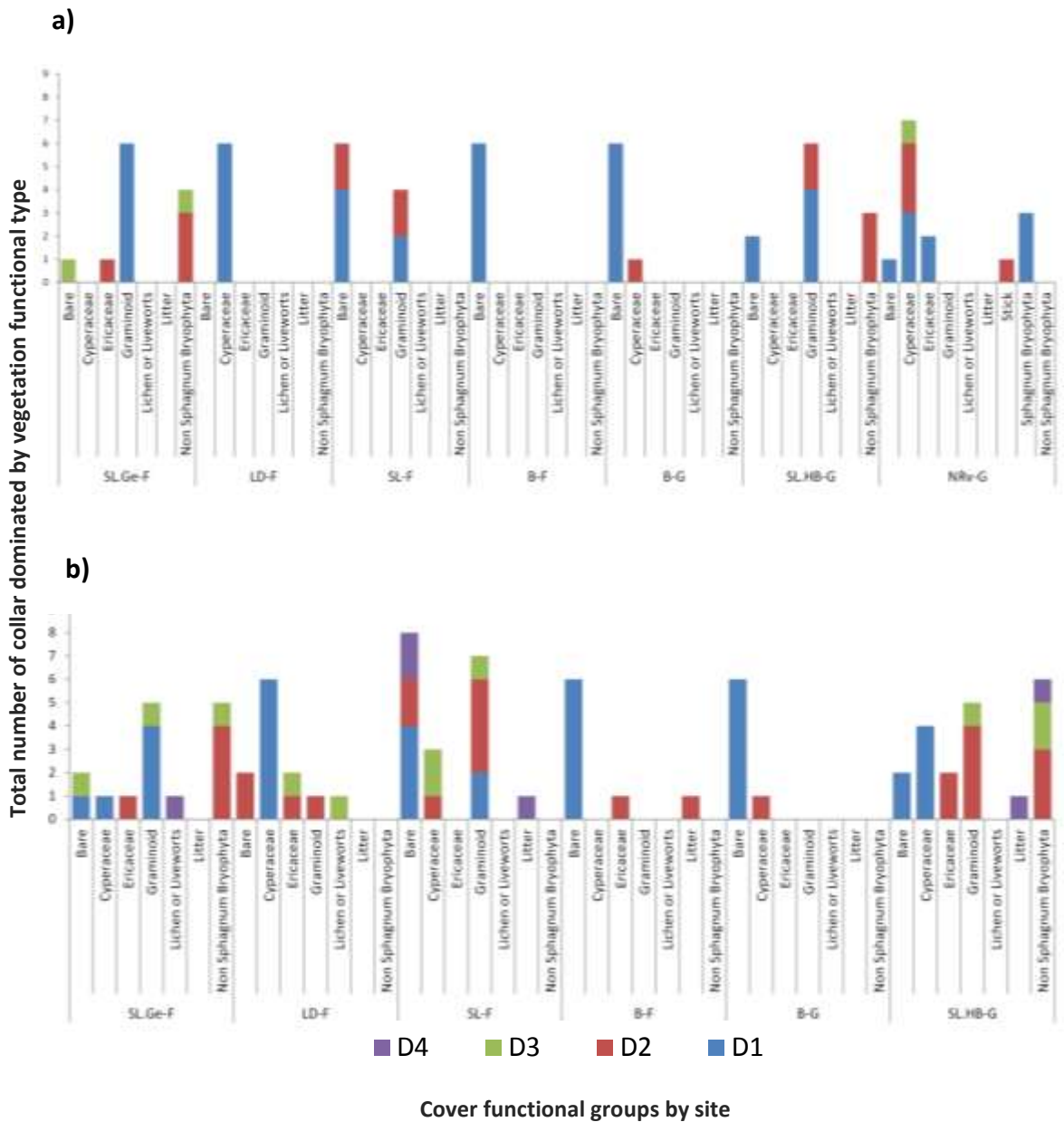
Figure 3.6: Bar chart of total plots vegetation dominance, by site and functional group (Bare, sedge, shrub, grass, other, Litter, Non Sphagnum moss and Sphagnum spp.) along the y-axis a) In 2009 and b) In 2011. The bars display present plot vegetation cover, in terms of 4 levels dominance levels, most dominant (D1) to least dominant (D4). The vegetation dominance at each site is not an accumulative value. Note: the only site with Sphagnum spp. was NRv-G. Refer to Table 3.1 for detail on site names.
