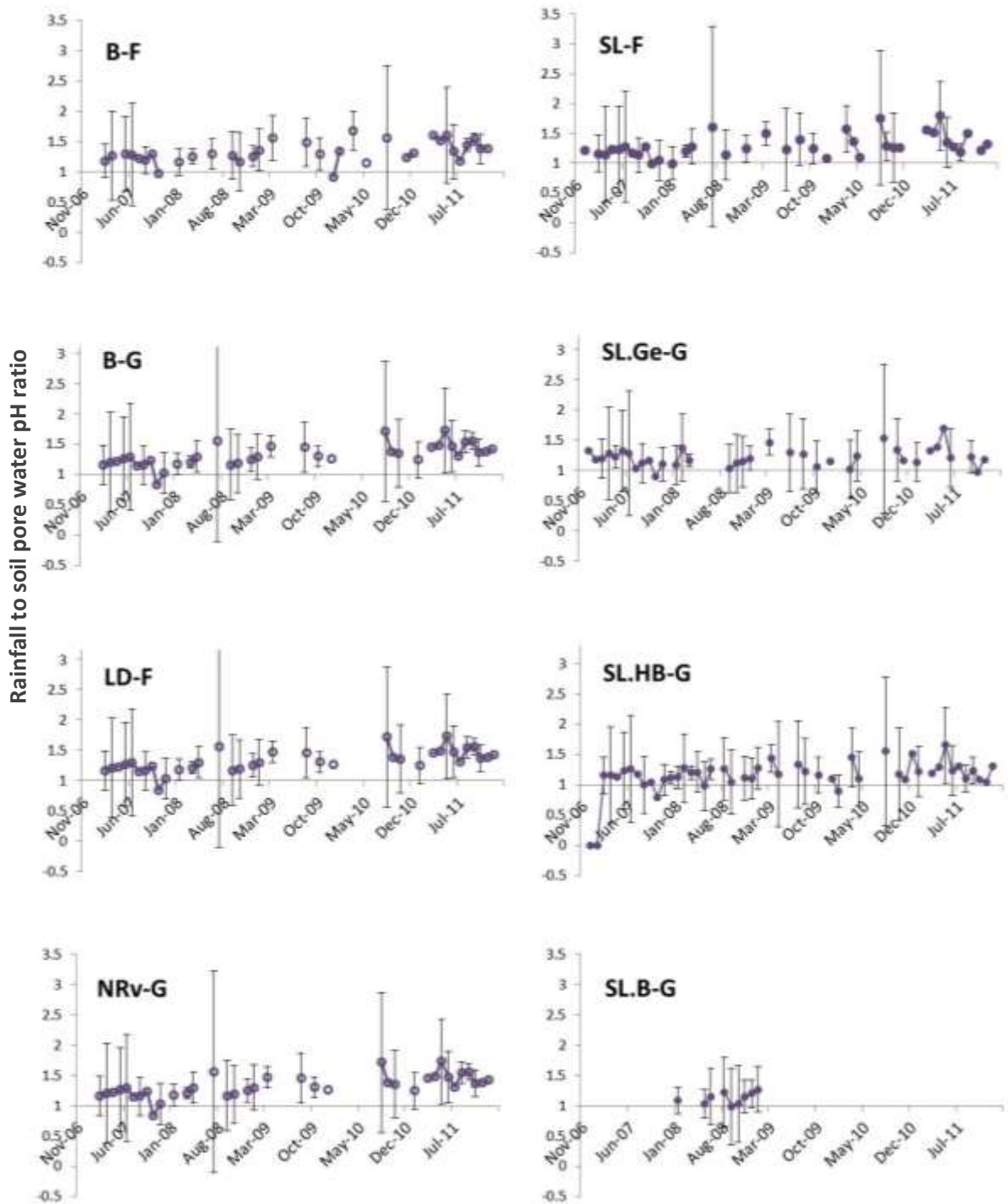
Figure 3.24: The ratio of rainfall to soil pore water pH (November 2006 – January 2012). Each data-points represents the monthly rainfall pH divided by site mean pH of the plot replicates on each site with error bars defining the standard error of the mean. The hollow purple circles signify site controls and the filled in purple circles represent sample pH measured at site with treatment. Point >1 signify that the mean rainfall pH was greater than the mean soil pore water during that month.
