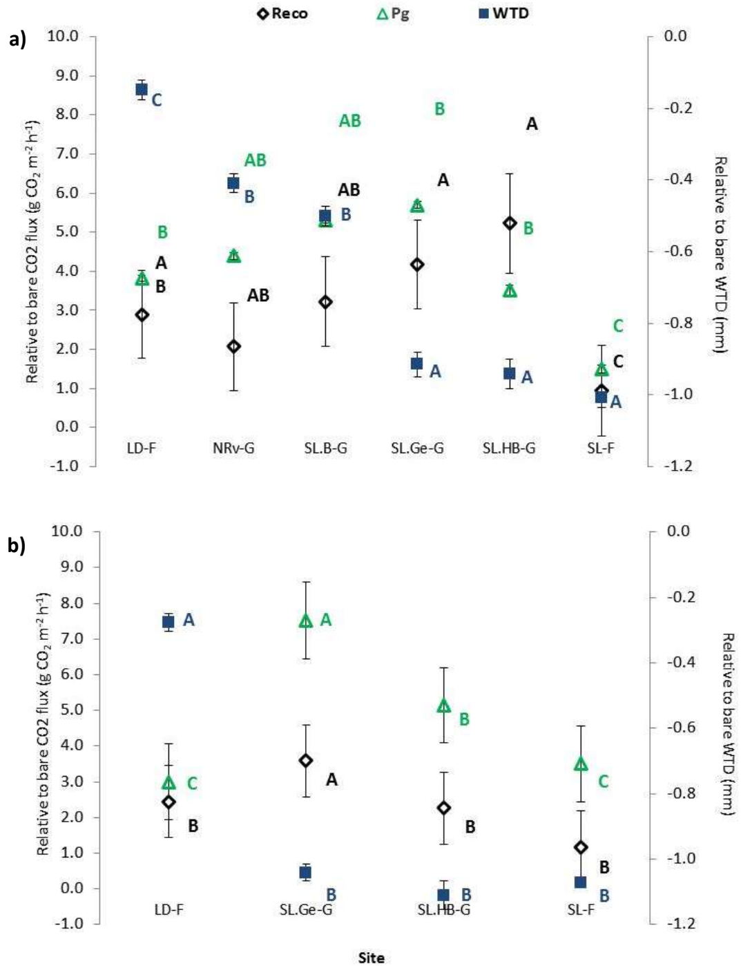
Figure 4.8: Main effects plots of relative to bare control (mean bare flat and bare gully): CO 2 fluxes (Left axis) - R_{eco} (black diamonds and letters) and P_g (green triangles and letters), and water table depth (blue boxes and letters- right axis) by site. a) At one year duration (2008), b) full five year study (2007-2011). Relative flux values >1 indicate site values were greater than bare control; <1 indicate site values were smaller than the bare control. WTD is a negative value, therefore relative values closer to >-1 are WTDs nearer the surface and most different to the bare control. Error bars denote SE error mean. The capital letters represent the significant differences between factor levels determined by post-hoc tests. The post hoc results are specific to each data set (e.g. R_{eco} ).
