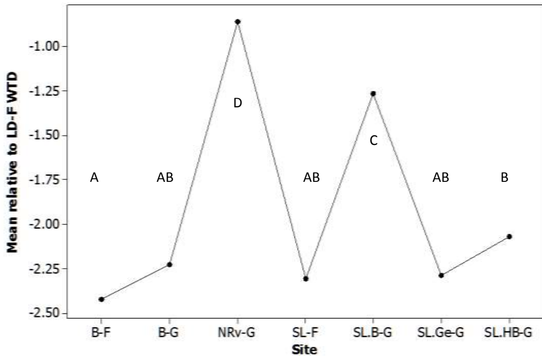
Figure 4.1: Relative to LD-F ( n = 314 ) water table depth ANOVA main effects plot by sites (2008). The letters on the plots represent the post hoc test results.
