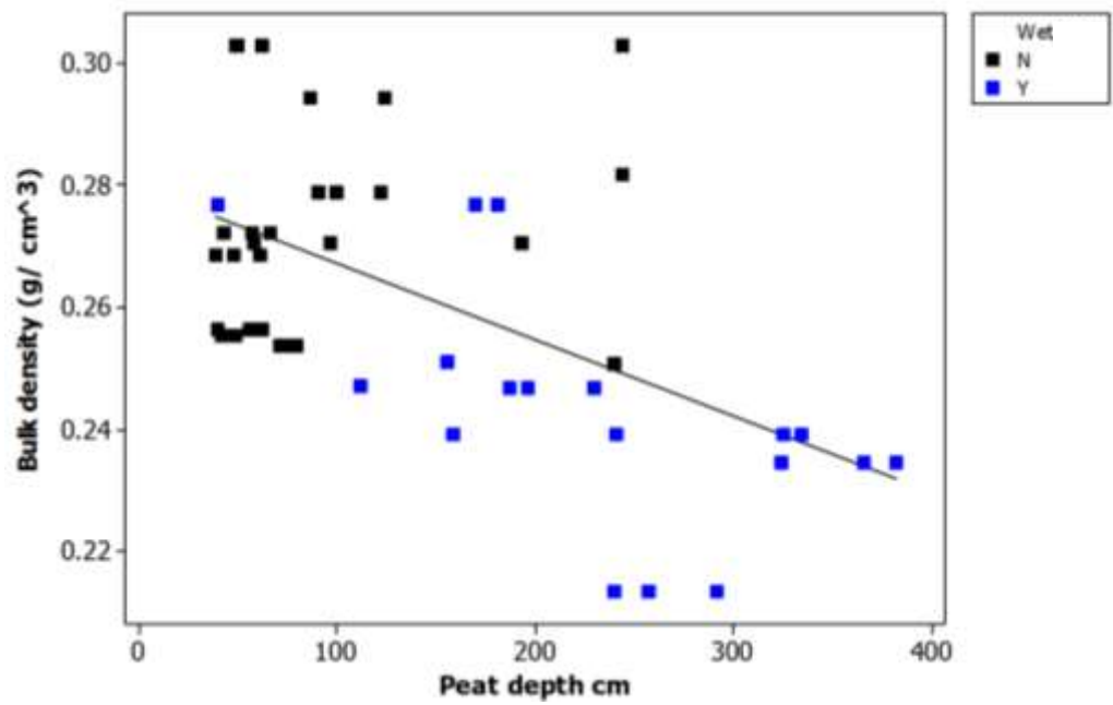
Figure 5.6: Regression plot of peat depth against bulk density, by site locality (wet vs. dry).
