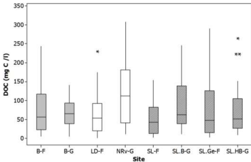
Figure 3.12: Box plot of site DOC (2008). The box plot colours represent the following: grey, bare soil controls; white, vegetated controls and grey striped, with restoration treatment.
