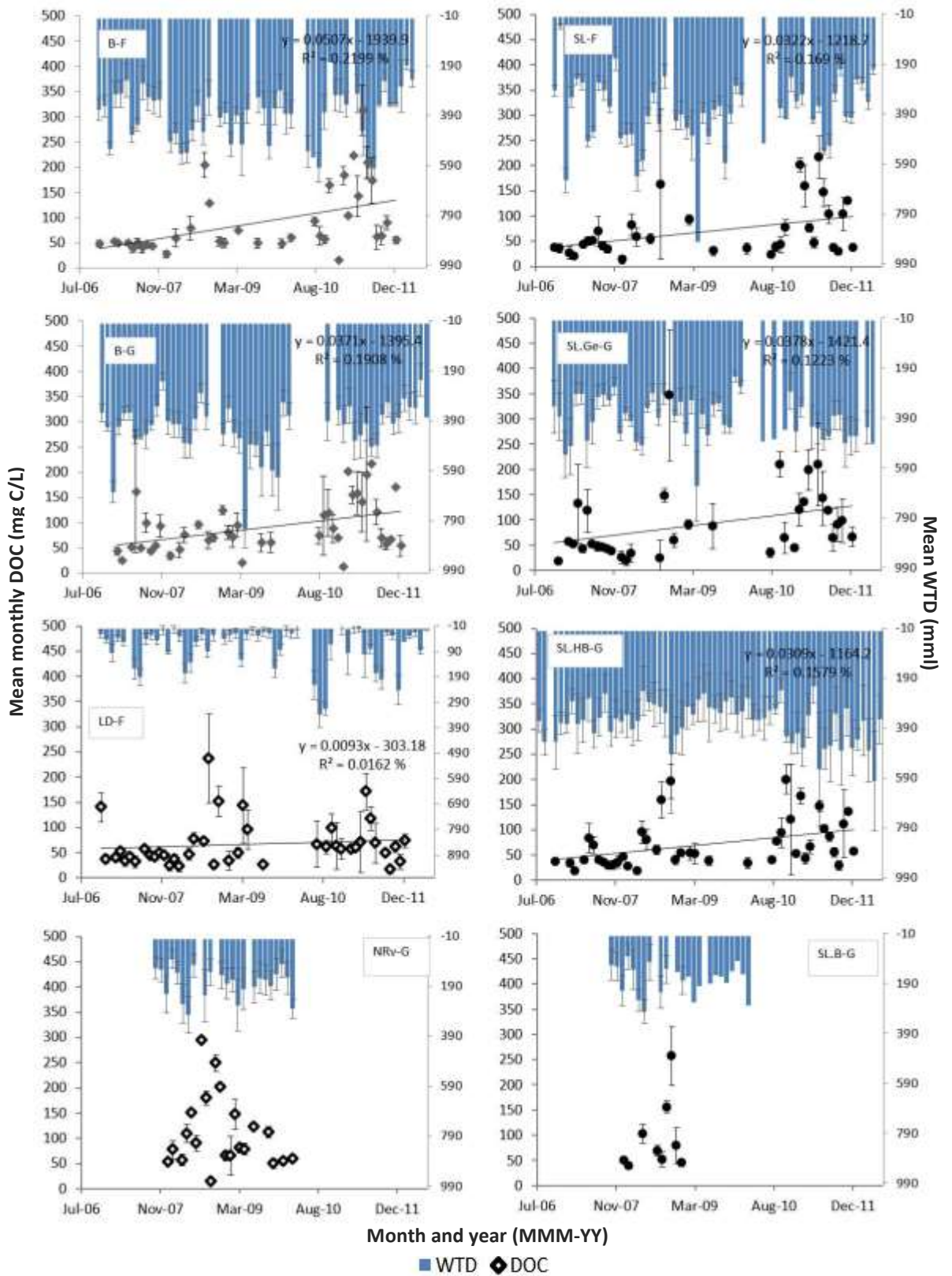
Figure 3.18: Bleaklow sites monthly mean soil pore water DOC conc. (left axes - mg C/L – diamonds: grey, bare untreated; black hollow, vegetated controls; black diamond, treated) and WTD (right axes - mm - blue bars) (2007 – 2011). The error bars represent the SE mean. A fitted trend line illustrates site long term DOC concentrations general trends.
