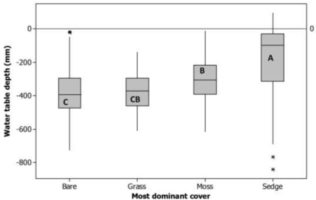
Figure 3.11: Box plot (five year study 2007-2011) of WTD plotted by 2011 primary site dominance. Letters on the plot are post hoc results of ANCOVA (Variables include: month and most dominant site cover, PAR, air temperature and total monthly rainfall).
