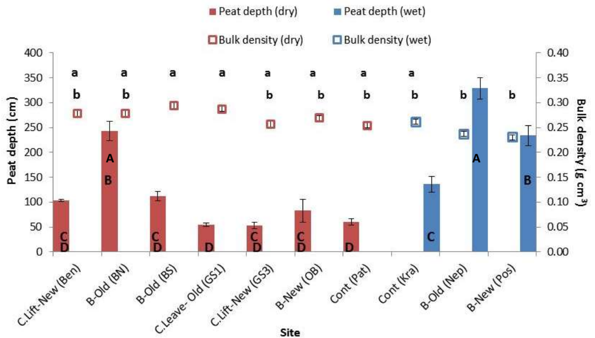
Figure 5.4: Goyt sites peat depth (bars: red, dry locality; blue wet locality) and bulk density (hollow blocks) raw data. The lettering represents post hoc analysis results. Lower case letter are the ANOVA post hoc results for bulk density ( n=32 ). The capital letters belong to the peat depth ANOVA post hoc test ( n=48 ). Site factor levels with shared letters indicate no significant difference; the opposite is true for different letters.
