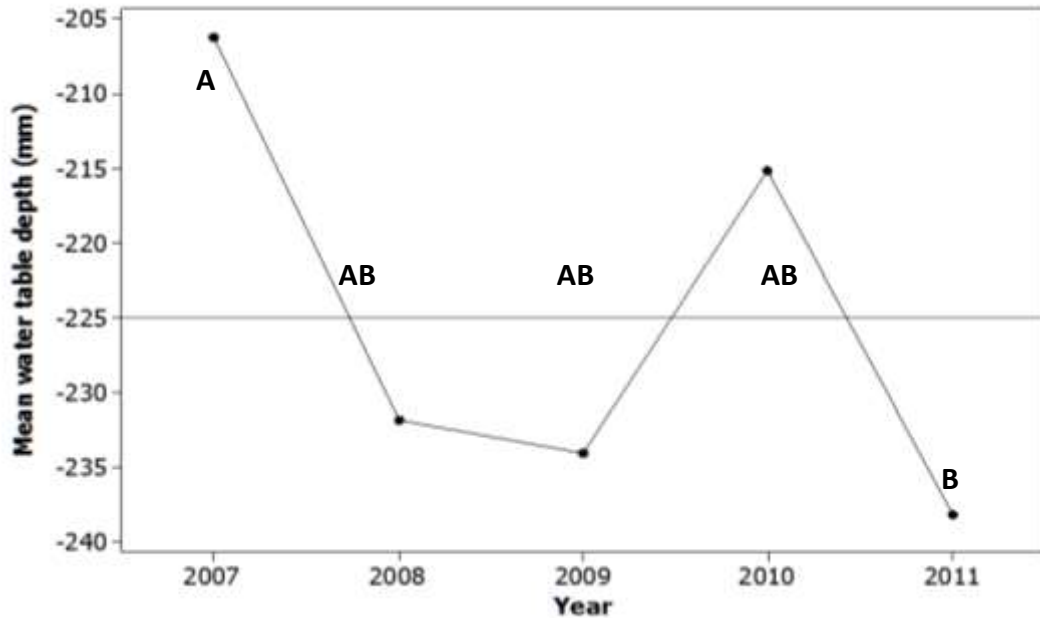
Figure 3.10: Water table depth ANCOVA main effects plot (2007 – 2011). Model inputs include: sites, plot nested within site, year, month nested within year. Covariates include: AT and PAR.
