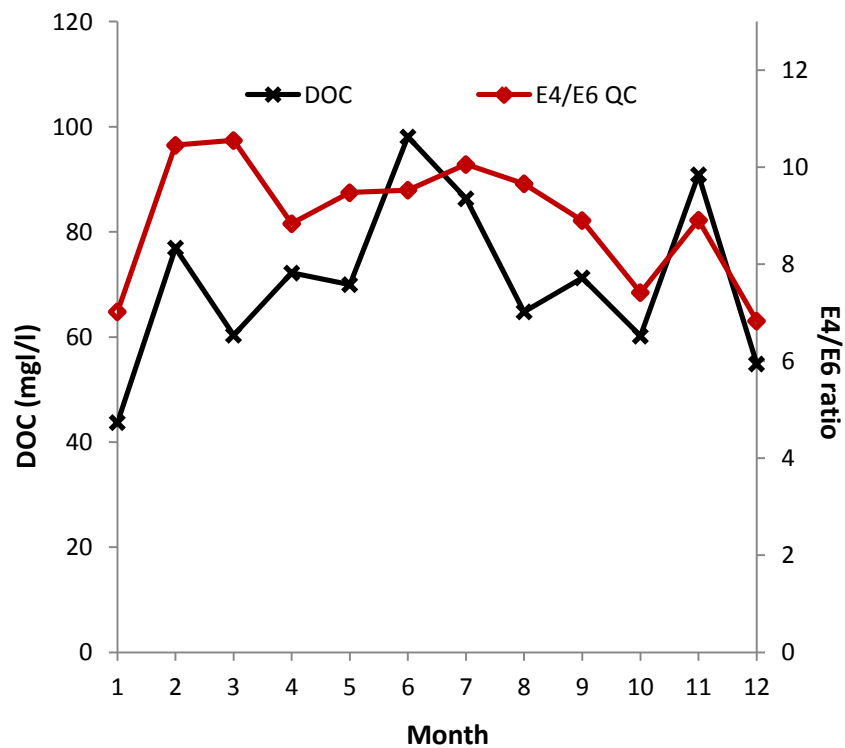
Figure 3.26: Mean monthly E_4/E_6 and DOC across all Bleaklow sites 2006-2011.
