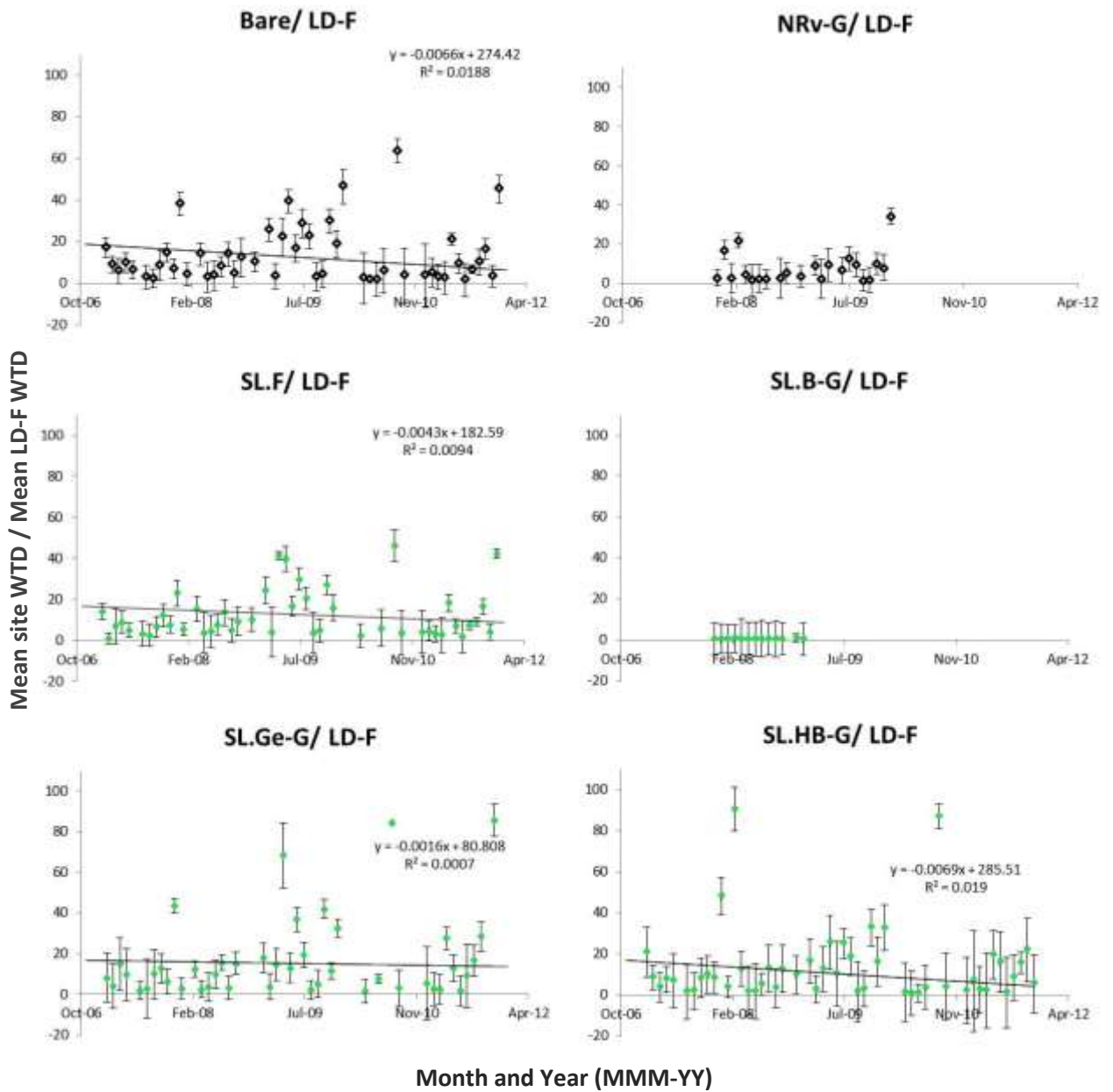
Figure 4.2: Six plots of site water table depth relative to the vegetated control (2006–2011). Bare signifies the average of B-F and B-G. The black-hollow diamonds represent untreated sites, and green diamonds represent treated sites. Values greater than one indicate site flux is greater than LD-F, values lower than one are smaller than LD-F. The error bars are the SE mean. A linear trend demonstrates the similarity between site and LD-F over time.
