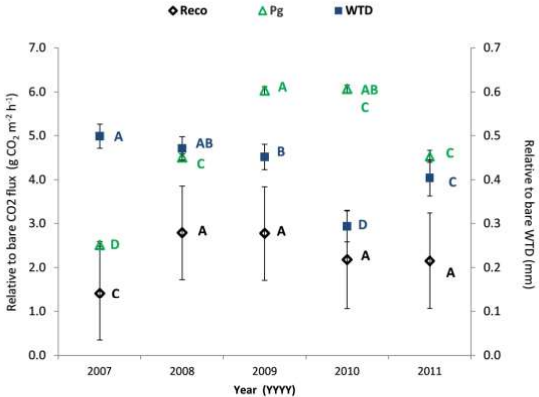
Figure 4.9: Main effect plot of pooled data (treatment sites and LD-F) relative to the bare controls: water table depth (Blue squares, Right hand axis) and relative to bare CO 2 R_{eco} (black-diamonds) and P_g (green triangles) fluxes (Left hand axis) by year (2007-2011) across the Bleaklow sites. Values closer to zero indicate the measure (relative to bare flux or WTD) were more similar to the bare site. Large relative values indicate the measure at a site was more different to the bare site control. Standard errors are denoted by error bars. The capital letters next are post-hoc tests results; the different letters represent significant differences between years (5 factor levels).
