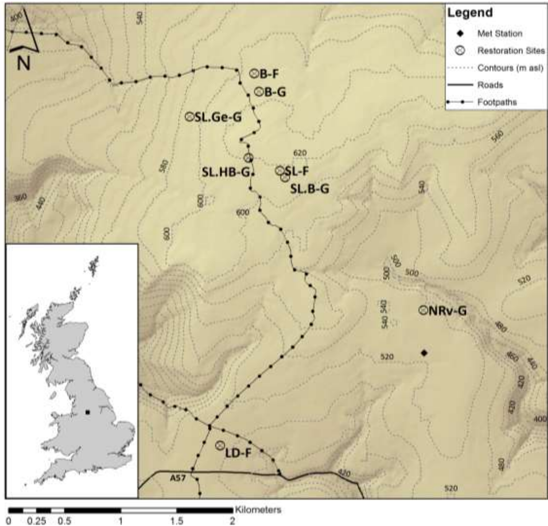
Figure 2.2: Location of study sites on the Bleaklow Plateau. For explanation of site codes see (Table 2.1). Bleaklow Plateau with field sites marked: Least disturbed flat (LD-F), naturally re-vegetated gully (NRv-G), seeded limed flat (SL-F), seeded limed gully blocked (SL.B-G), seeded limed heather brash gully (SL.HB-G), seeded limed geojute gully (SL.Ge-G), bare gully (B-G), bare flat (B-F) and met station. (Figure adapted from Dixon et al. 2014).
