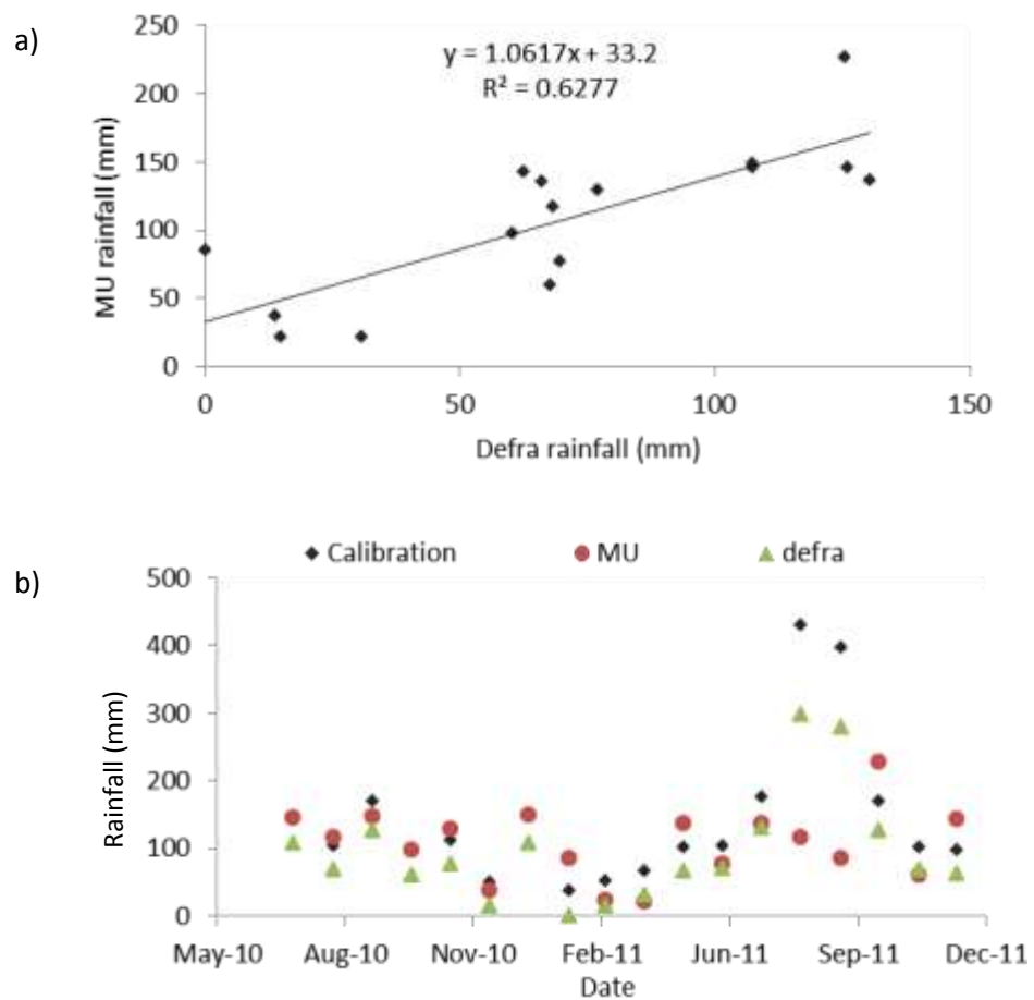
Figure 3.5: Rainfall data calibration a) Calibration of defra data to Bleaklow MU AWS. MU AWS Monthly rainfall is along the y-axis and Defra rainfall is along the x-axis.; b) monthly rainfall sum Defra data (green triangle), MU AWS data (red circle) (Jul 2010 – Dec 2011) and calibrated rainfall values using calibration in graph 3.5a (black diamonds).
