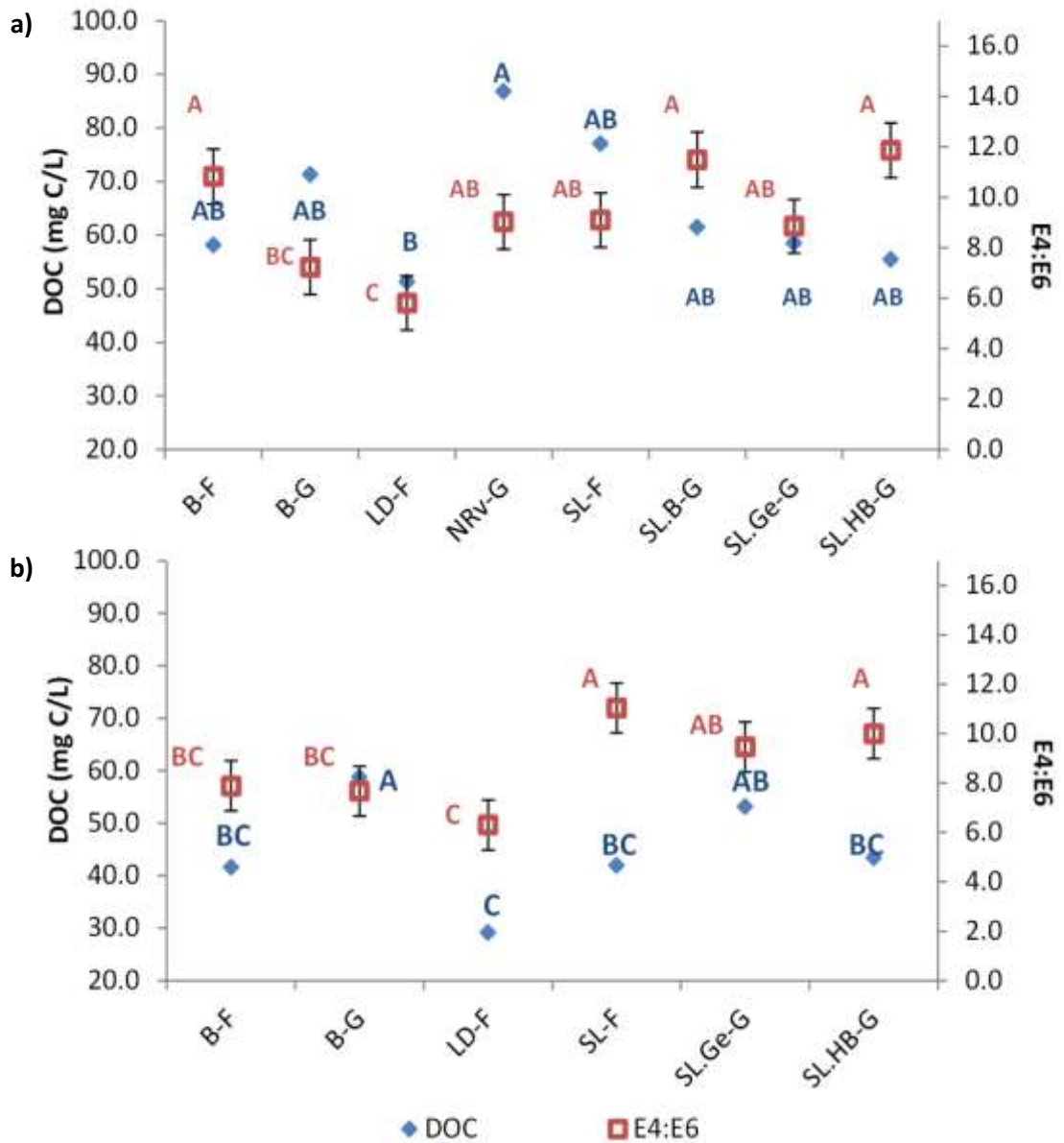
Figure 3.13: Main effects plot by site for DOC (normalised square root) in blue and E_4/E_6 (natural log) in red: a) 2008 data ANCOVA; b) 2007 – 2011 data ANCOVA. The ANCOVAs included the factors site and month. The Letters signify post hoc tukey test results whereby the means that do not share a letter are significantly different.
