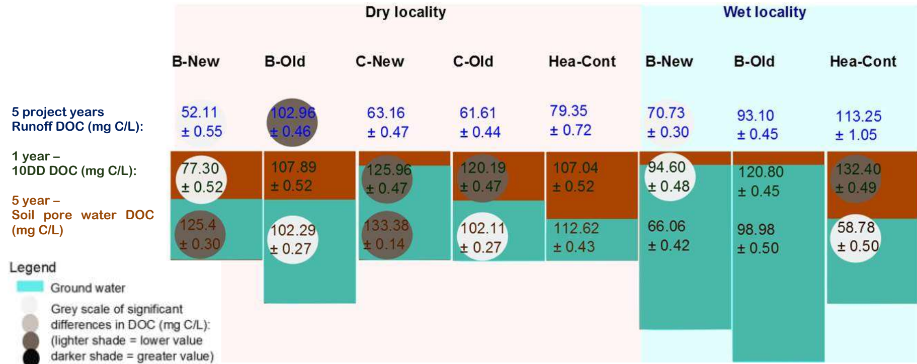
Figure 7.2: Conceptual diagram of the Goyt Valley heather management study (2008 – 2013) key result (ANCOVA and post hoc results). The figure includes eight schematics/ peat cross sections representing managed heather sites and controls at: a dry on the left (heather control, new burn, old burn, new cut, old cut) and wet locality on the right (heather control, new burn and old burn). Significant differences are read by locality and horizontally by sample type (not between water samples types). The figure includes: mean DOC concentration values; shaded circles, significant differences between the sites DOC (by sample type); blue unit, ground water and water table. Site details are available in thesis methodology (Chapter 2).
