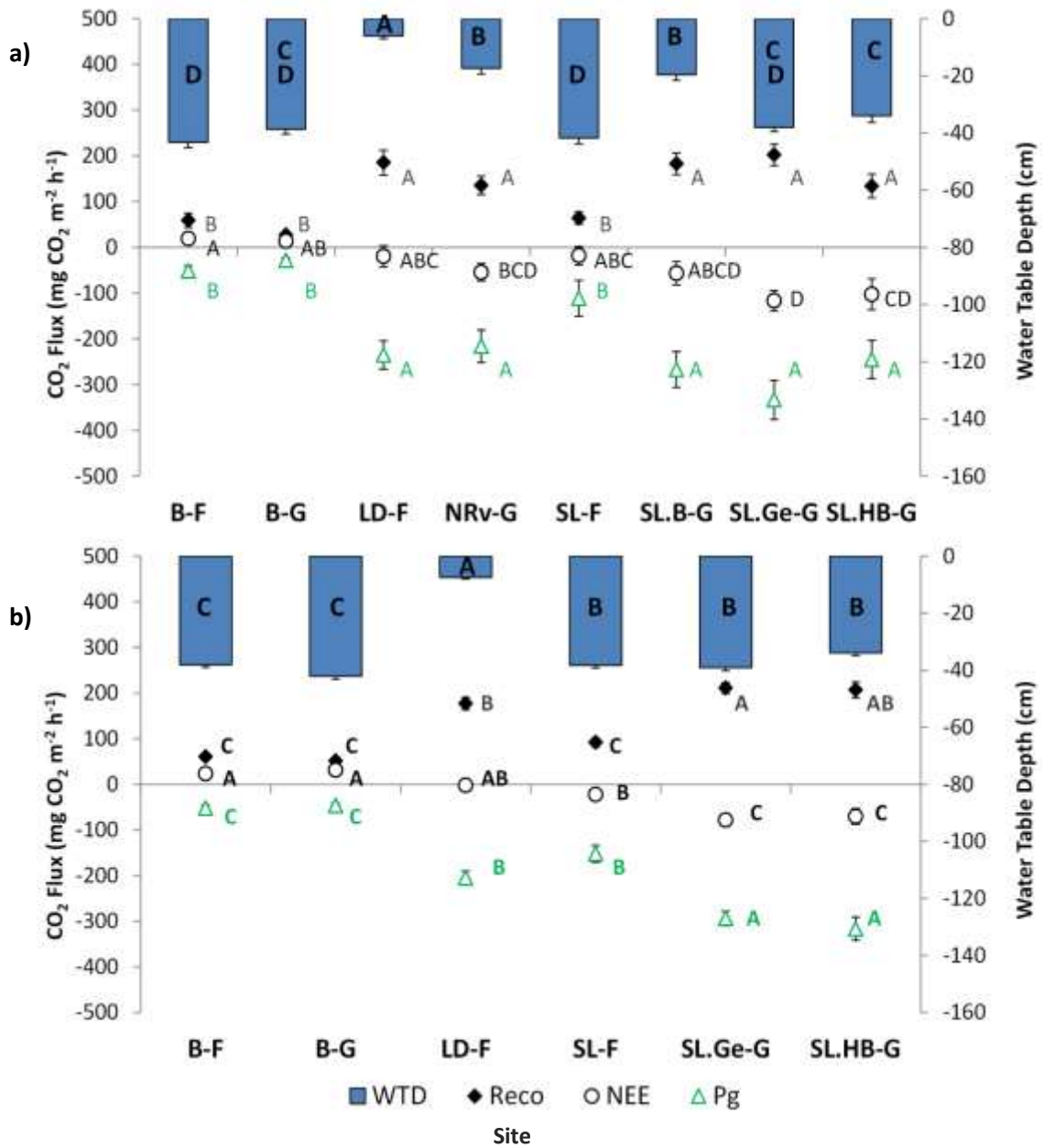
Figure 4.5: Mean water table depth (WTD – right y-axis) and CO 2 fluxes ( R_{eco} , NEE, P_g – left y-axis) a) by site for the one year dataset (2008); b) for the full five year dataset (2007 - 2011). Error bars denote SE mean, in some cases the errors are smaller than the data-points themselves. The letters within/next to each bar/data-point represent the post-hoc tests results. Sites with different letters for a given dataset (e.g. R_{eco} ) are significantly different in terms of the magnitude of that flux. Grey-drop-boxes denote water table depth, black-diamonds denote R_{eco} , white-circles denote NEE, and white-triangles denote P_g . (Figure adapted from Dixon et al. (2014)).
