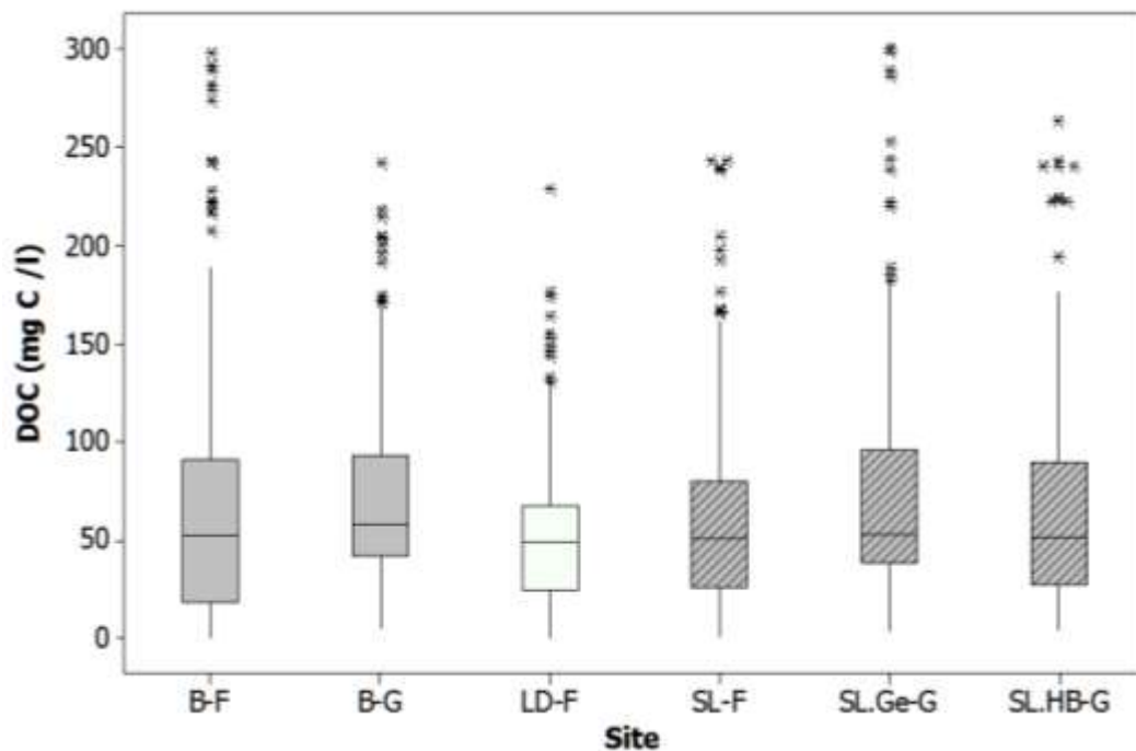
Figure 3.16: Box plots of soil pore water DOC concentrations (2007-2011) by site. The grey boxes are bare soil controls, white is least vegetated controls and grey striped are sites with restoration treatment.
