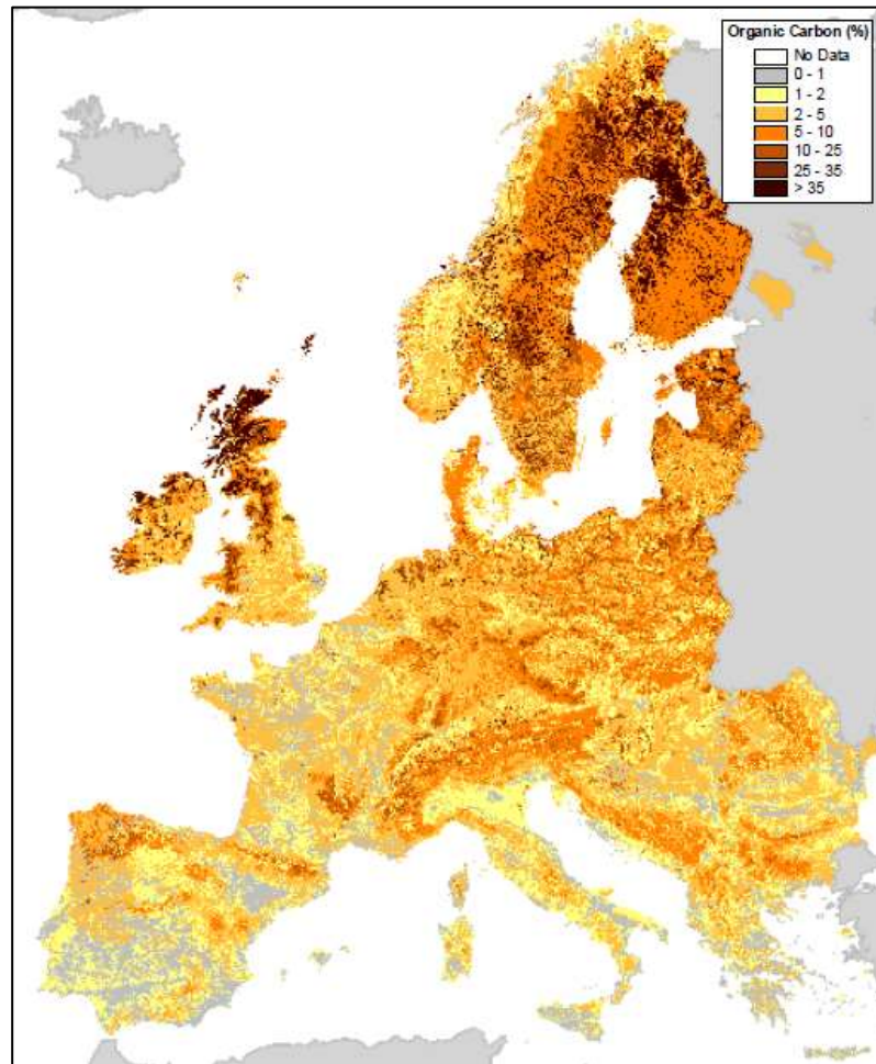
Figure 1.1: European topsoil organic carbon percentage. The ranges of organic carbon are greater at darker shades, which coincide with the presence of peat (Jones et al. 2005).
