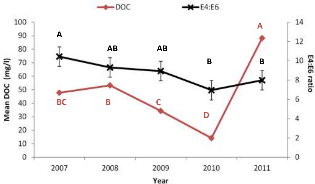
Figure 3.17: Main effects plot (2007 – 2011) of DOC (brown diamond) and E_4/E_6 (black cross), using natural log data valued in an ANCOVA. Model Inputs included site, year and month. Left axis is DOC (mg/L) and right axis is the E_4/E_6 ratio. The letters on the plot represent the tukey post hoc result. Shared letters represent no significant differences between year factor levels.
