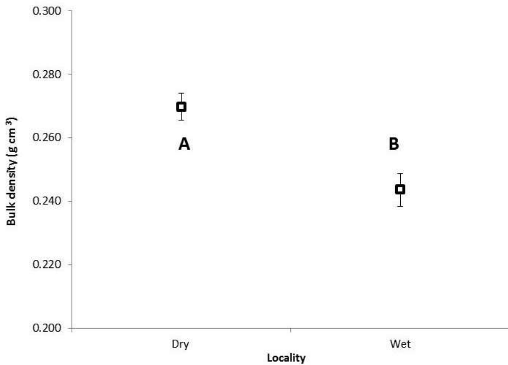
Figure 5.7: Main effects plot for bulk density (black hollow squares) by locality. Post hoc analysis results are displayed as letters. Different letters denote significant differences between localities.
