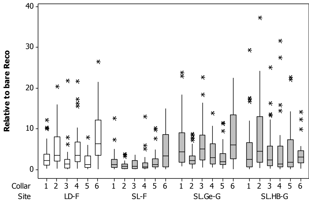
Figure 4.7: Box plot of relative to bare ecosystem respiration ( \text{g CO}_2 \text{ m}^{-2} \text{ h}^{-1} ) (2007–2011), by site and collar.
