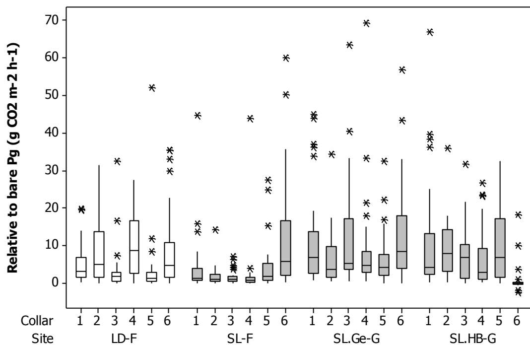
Figure 4.11: Box plot of relative to bare gross photosynthesis (2007–2011) by site and collar. The grey box plots represent collar within with treated sites, white box plots are collar within the untreated least disturbed vegetated control.
