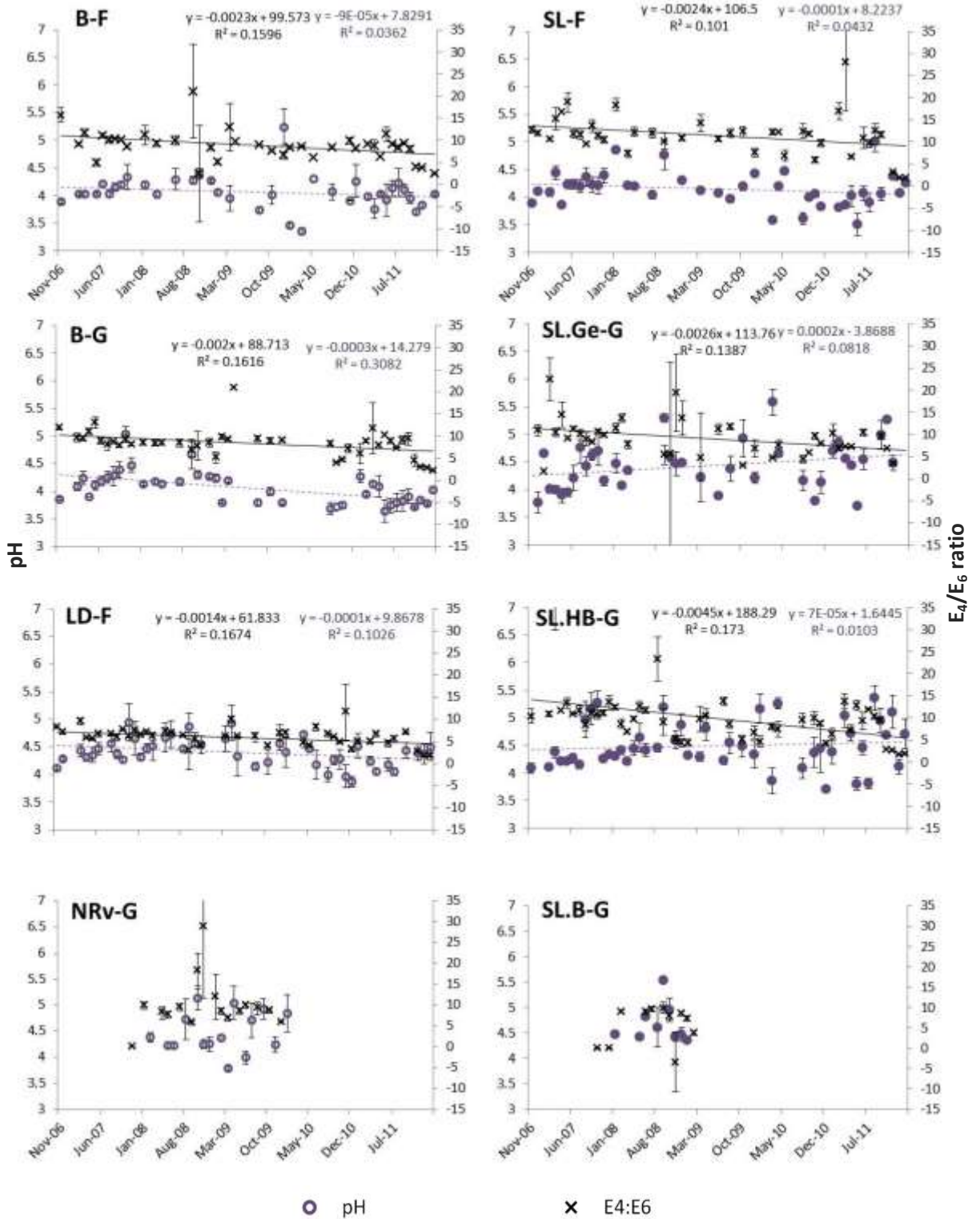
Figure 3.22: Bleaklow soil pore water monthly (x-axis, November 2006 – January 2012) mean pH (left y-axis) and E_4/E_6 (right y-axis). All data-points are mean monthly values with error bars defining the SE mean. The purple circles are pH (hollow circles signify controls). The E_4/E_6 ratios are represented by black crosses. Multiannual linear trends are displayed for both the pH (dash purple) and E_4/E_6 (black line).
