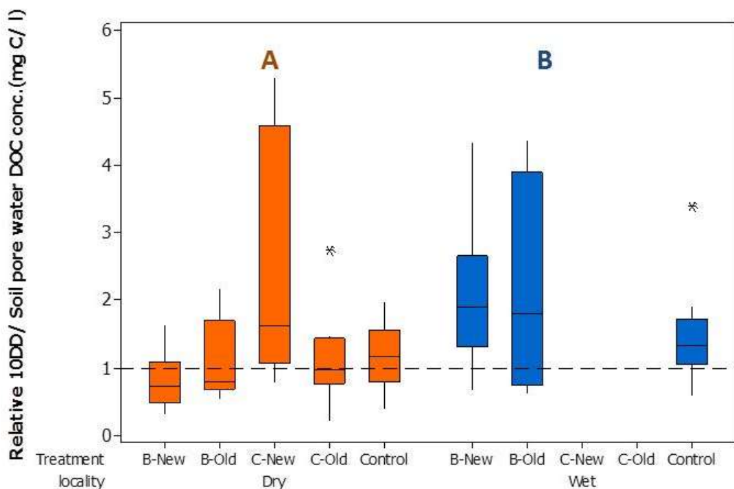
Figure 6.6: Boxplot of difference relative DOC concentration 10DD/1m. The letters signify post hoc results for difference between the factor locality (wet or dry). The dashed line represents a 1:1 ratio of DOC concentration in 10DD and soil pore water samples. Note: there are only three wet site (blue) box whiskers as there were no cut sites in the wet locality
