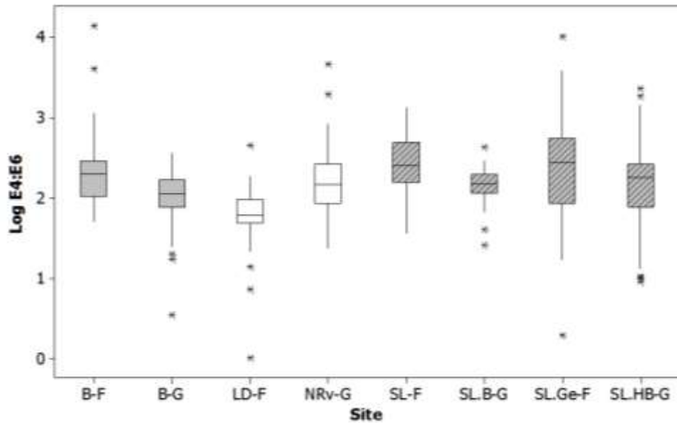
Figure 3.21: Box plot of Bleaklow sites soil pore water E_4/E_6 (logged) (2008). The box plot colours represent the following: grey are bare soil controls, white are vegetated controls and grey striped are sites with restoration treatments.
