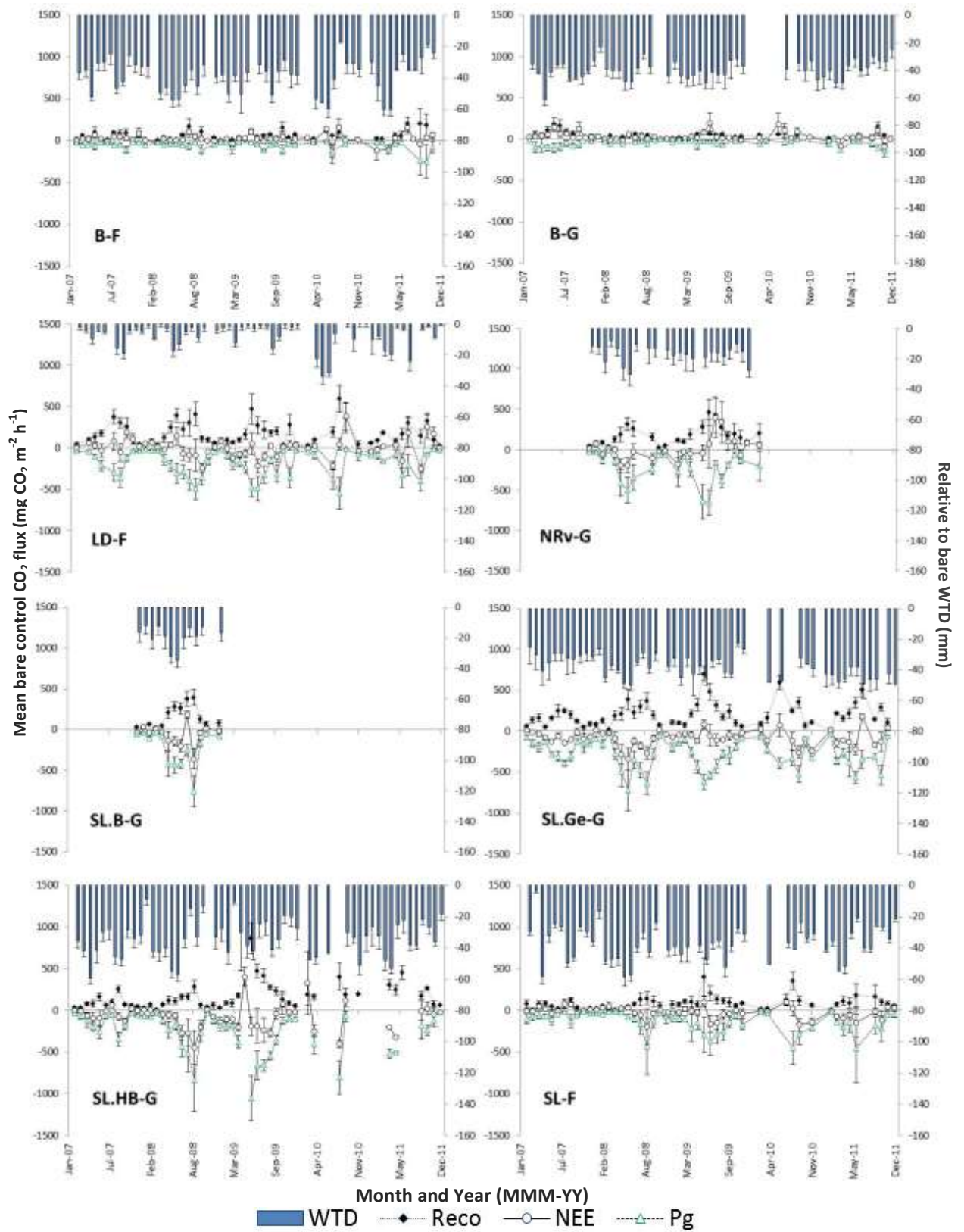
Figure 4.4: Bleaklow absolute data (Jan 2007 – Dec 2011): mean water table depth (WTD – right y-axes) and CO 2 fluxes (Reco, NEE, Pg – left y-axes) by month and site. All data-points represent the monthly site mean, with error bars defining SE mean. Blue-drop-boxes denote WTD, black-diamonds with a thin dashed connect line denote R_{eco} , white-circles with a solid black connect line denote NEE, and green-triangles with a thick dashed connect line denote P_g . (Figure adapted from Dixon et al. (2014)).
