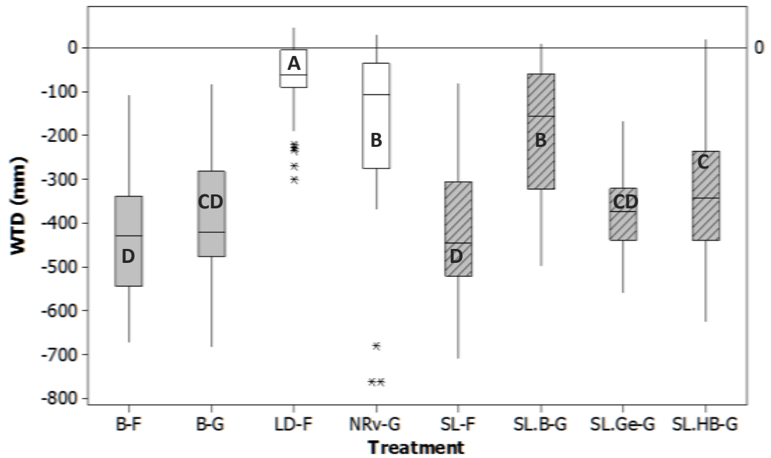
Figure 3.7: Box plot of WTD by site (2008). Letters on the plot are post hoc results of an ANCOVA (Factor inputs include: month, site and PAR). Shared letters indicate significant differences between site factor levels. The zero line indicates the peat soil surface. There are three box plot colours: grey, bare soil controls; white, vegetated controls; and grey striped, site with restoration treatment. Refer to Table 3.1 for detail on site names and treatment types.
