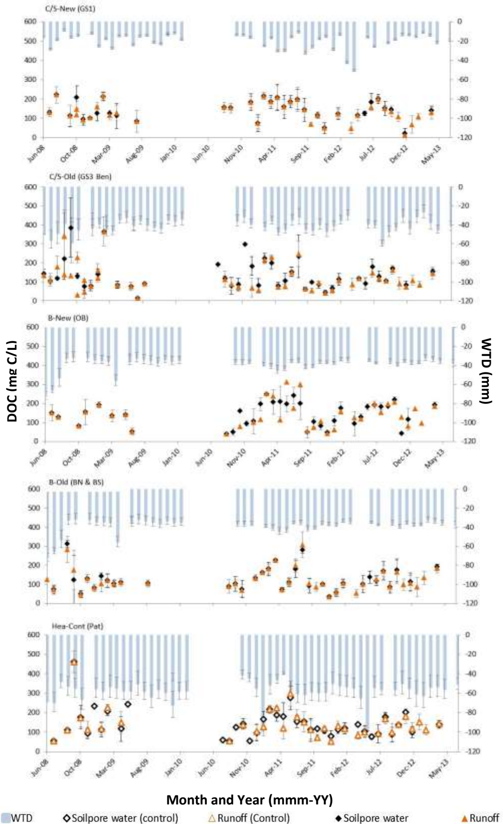
Figure 5.11: Goyt valley cut versus burn study (dry locality Big Moss) absolute data (Jun 2008 – May 2013): mean WTD (right y-axes, blue-drop-boxes) and DOC concentrations (left y-axes) in surface runoff (yellow triangles) and soil pore water (black diamond), by site, month and year. All data-points represent the monthly site mean with error bars defining the SE mean. Refer to methodology (section 2.2) for site details.
