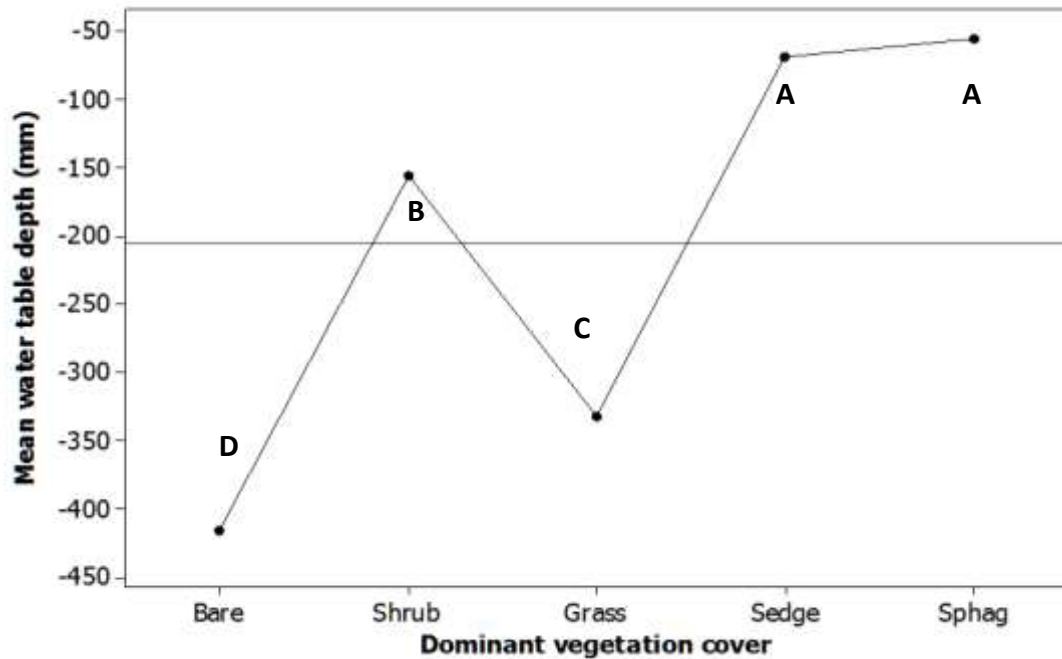
Figure 3.8: Main effects plot of WTD (2008) by primary plot cover dominance (2009). ANCOVA (Factor inputs include, month, most dominant site cover and PAR). Letters on the plot are tukey post hoc results. Shared letter indicate no significant different between levels.
