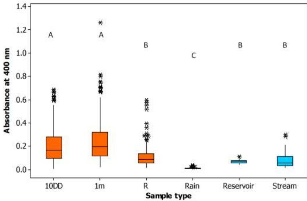
Figure 6.13: Box plot of sample absorbance at 400 nm by water sample source type (orange box plot, samples from treatment sites; blue box plot, rainfall, reservoir and stream water). The letters signify the post hoc test results. Different letters indicate significant differences between sample type factor levels.
