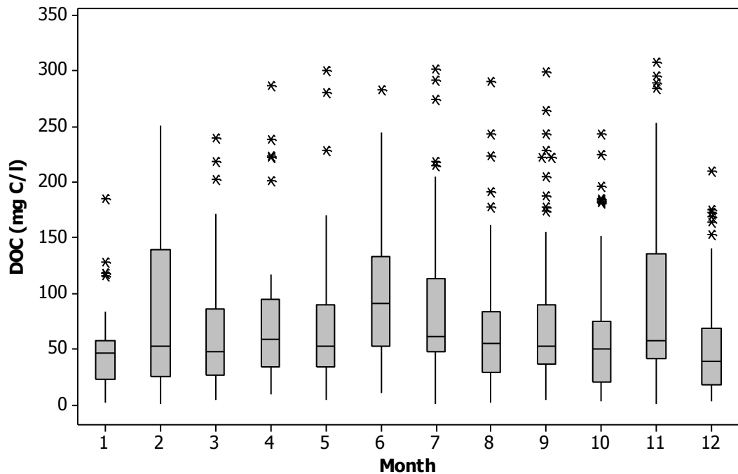
Figure 3.15: Boxplot of Bleaklow soil pore water DOC by month (2007 – 2011).
