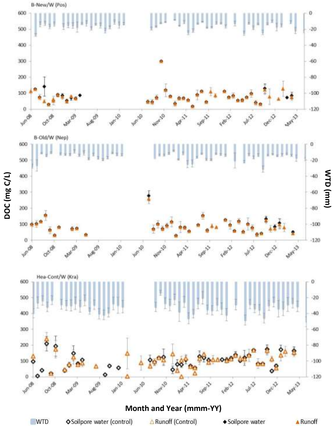
Figure 5.13: Goyt valley burn study in wet locality (Ravenslow) absolute data (Jun 2008 – May 2013): mean WTD (right y-axes) and DOC (left y-axes) by site, month and year. All data-points represent the monthly site mean with error bars defining the SE mean. Blue-drop-boxes denote WTD. Refer to methodology (section 2.2) for site details.
