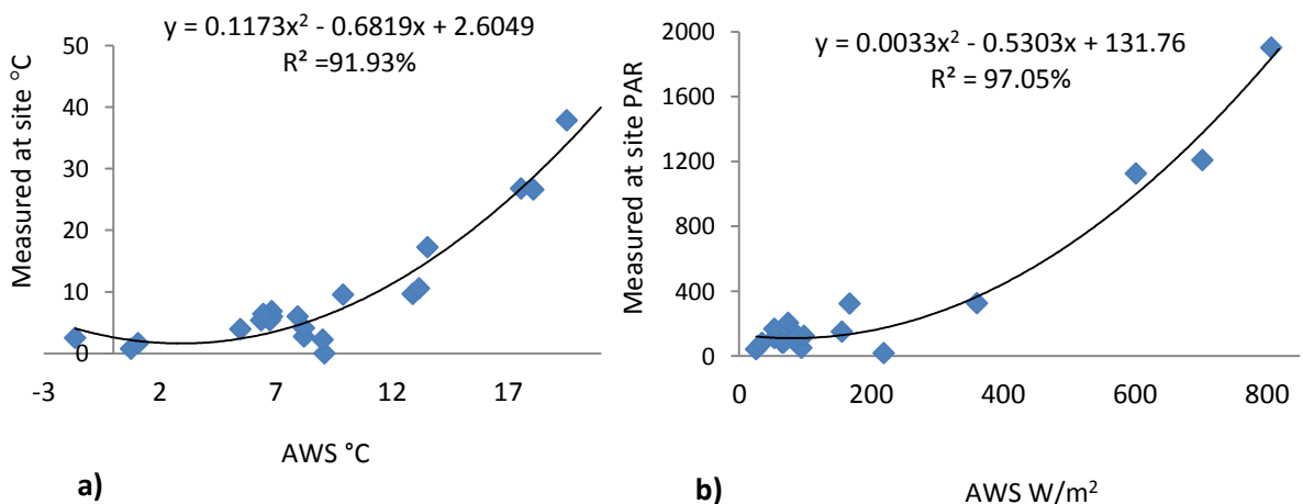
Figure 3.2: Data calibration plots: a) Temperature calibration b) Solar radiation-PAR calibration.
