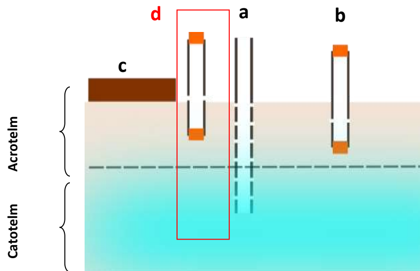
Figure 6.1: Experimental plot design. a) dipwell, b) surface runoff trap, c) gas collar, d) intermediate depth soil pore water sample trap.
