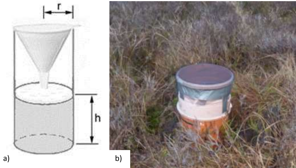
Figure 5.1. Rain gauge, a) cross section b) example of gauge in field (Ravenslow, Nep)
