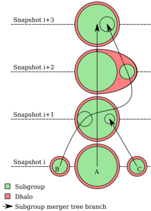
Figure 3.2: Schematic showing an example of a Dhalo merger. At snapshot i , haloes A, B and C are distinct and belong to their own individual Dhaloes. Subhaloes B and C fall into A by snapshot i + 1 , then although B is no longer residing within A at snapshot i + 2 , it still belongs to the Dhalo, and always will at later times. At snapshot i + 3 , B has rejoined A. Figure from Jiang et al. (2014).
