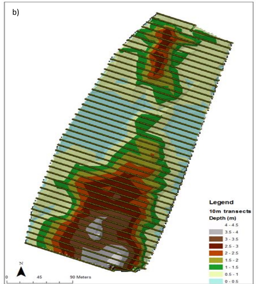
Figure 5.18 – Depth map interpolated from GPR data using 10m transects
