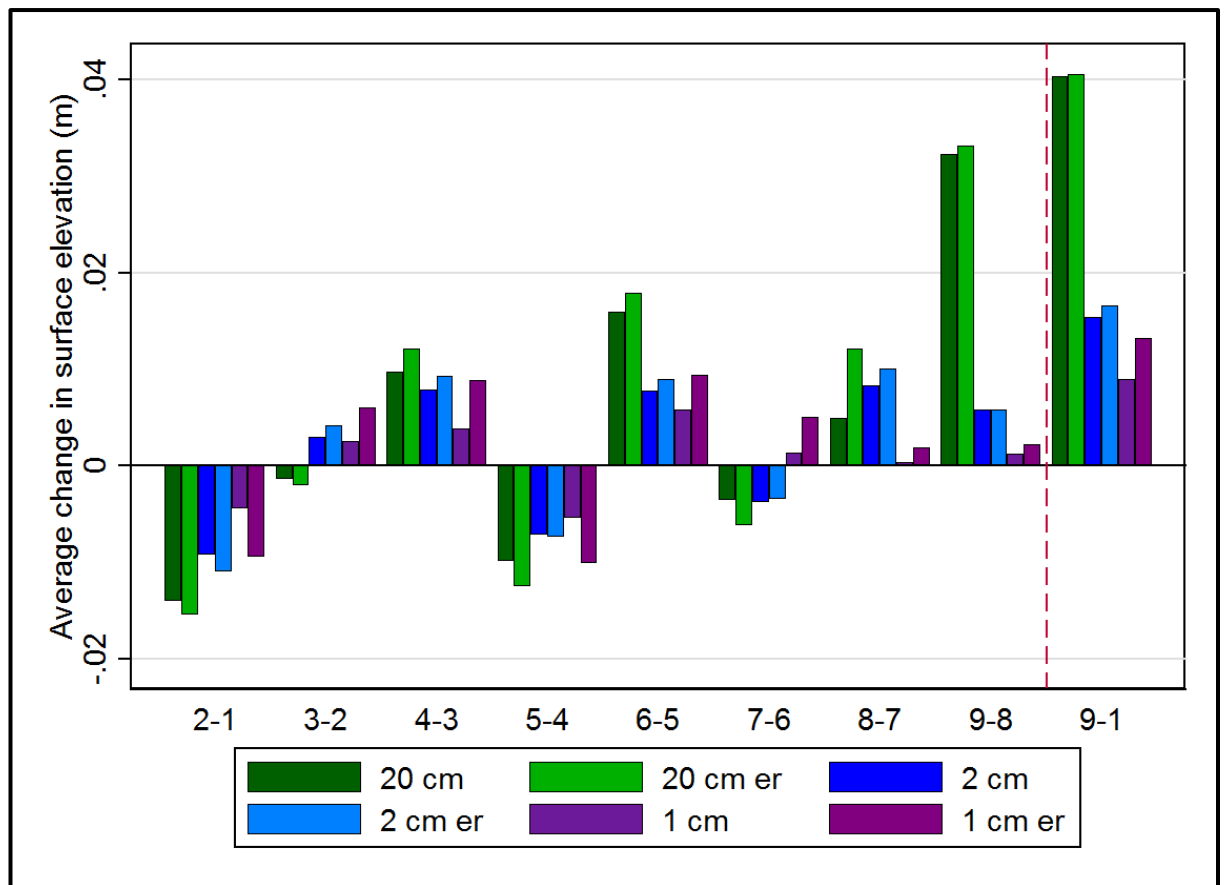
Figure 6.24 – A bar chart showing the change in surface elevation calculated using DoDs filtered at three different resolutions and calculated using DoDs with the error values (+/- 0.0071 m) removed (labelled as ‘er’ on the plot). Data calculated for the entire TLS monitoring period are shown to the right of the red dashed line.
