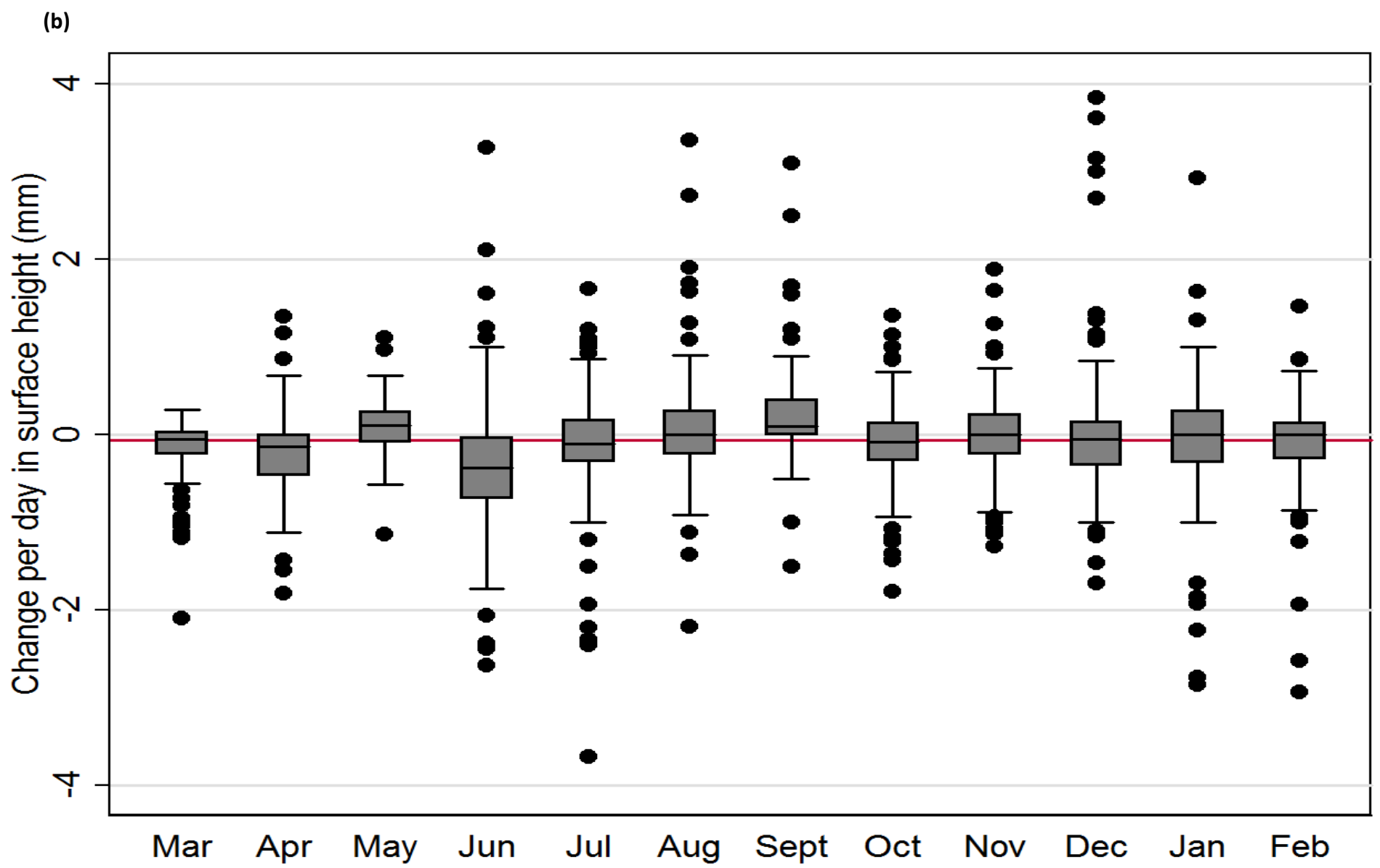
Figure 6.6 – (a) Change per day of pin exposure plotted by site and (b) change per day for each month. The red line indicates the mean value of change per day of 0.06 mm.
