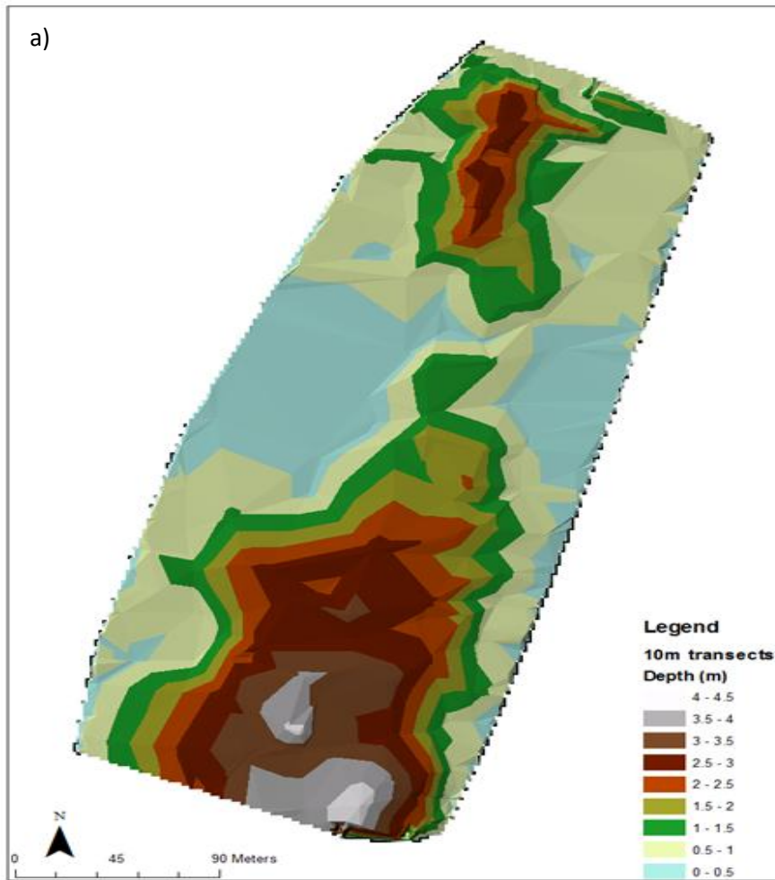
Figure 5.18 – Depth map interpolated from GPR data using 10m transects
