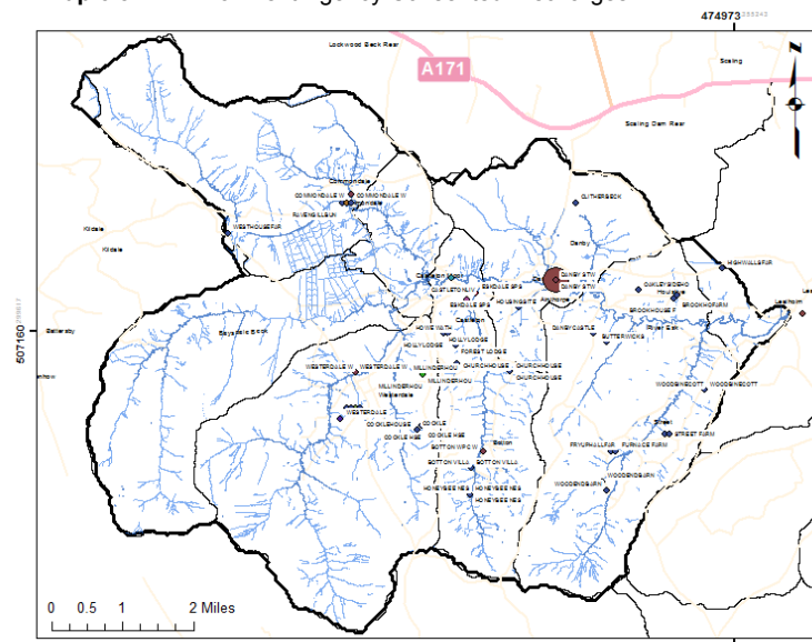
Map 3.5.4. Environment Agency Consented Discharges
