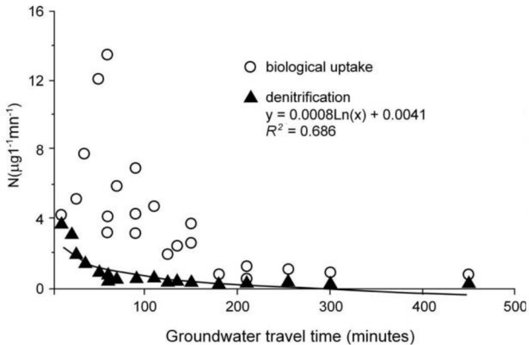
Figure 6.2. Hyporheic travel time after nitrate injection – biological uptake and denitrification impact on concentration
