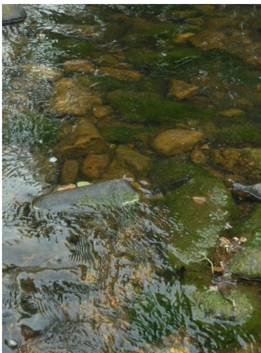
Figure 6.6. Lealholm Crunkly Gill – aquatic bryophyte moss establishment
