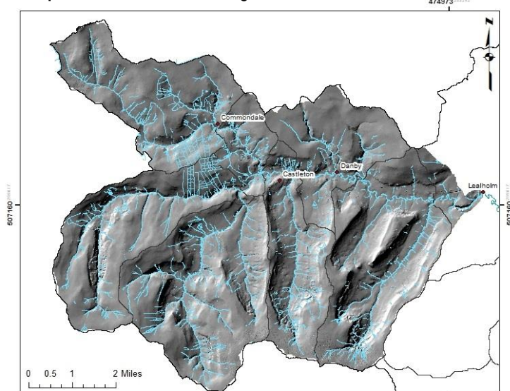
Map 3.5.3. LIDAR: Hill-shade Digital Surface Model
