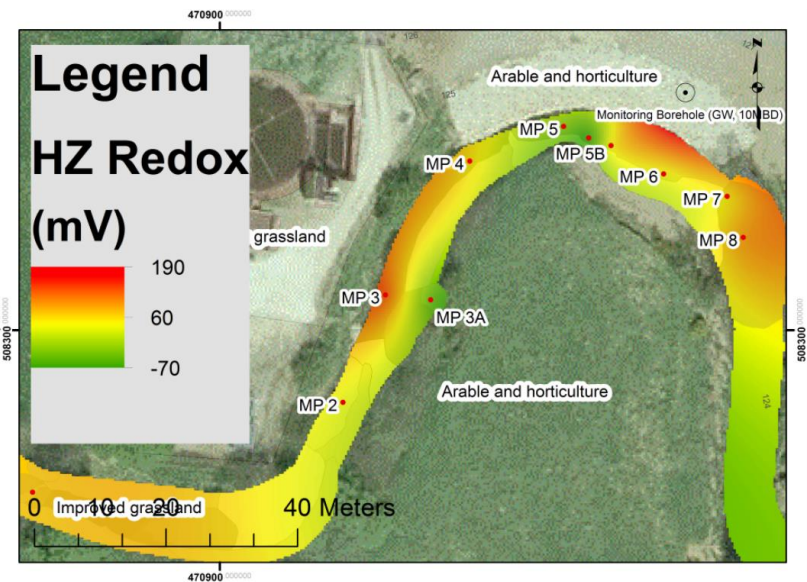
Maps 5.4. Reach-scale spatial variability in average Ammonium ( \text{NH}_4^+ ) and Redox (mV) across in-stream and hyporheic waters
