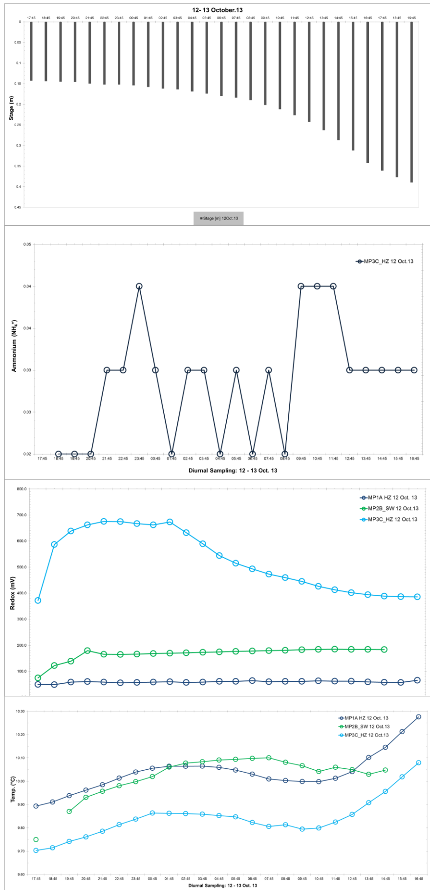
Figure 5.43. 24 Hour diurnal variability in Ammonium (NH 4 + ), Redox (mV) and Temperature (°C) across a pool-riffle-pool – 12 – 13 th October 2013
