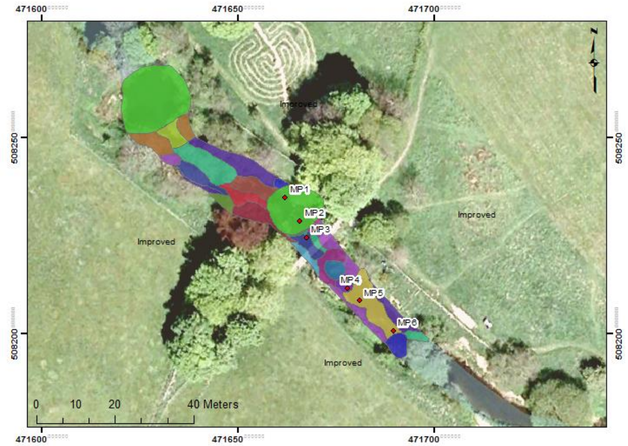
Map 4.2. Aerial Perspective: Stream-units and Riparian Landuse
