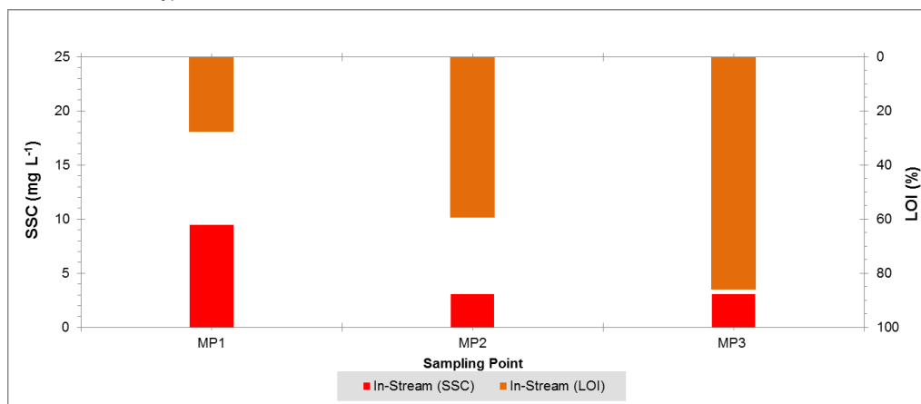
Figure 5.74. Suspended sediment concentration (SSC) ( \text{mg L}^{-1} ) and LOI (%) longitudinal change across in-stream and hyporheic waters
