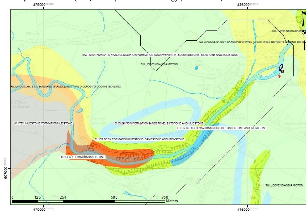
Map 3.7.3. Bedrock (halo) and Superficial Drift Geology (standard text)
