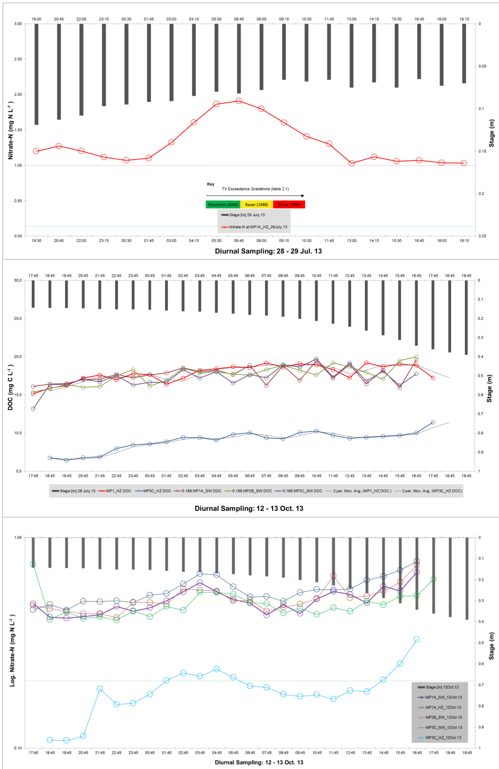
Figure 5.42. 24 Hour diurnal Nitrate-N ( N-NO_3^- ) and Carbon (DOC) change across a pool-riffle-pool and in the pore water of a riffle-head: On 12 – 13 th October 2013 and 28-29 th July 2013
