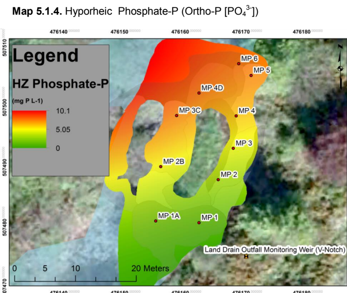
Maps 5.1 Reach-scale spatial variability in average Phosphate-P (Ortho-P) and Nitrate-N ( N-NO_3^- ) across in-stream and hyporheic waters
