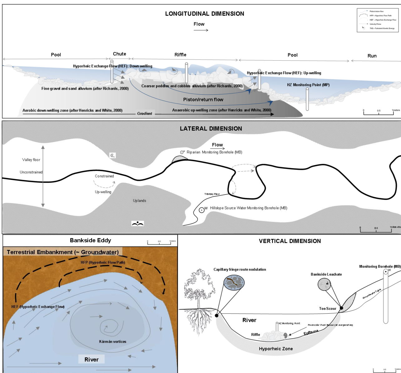
Figure 4.1. 3D sampling strategy designed to sample hydrodynamic source waters – surface, ground and hyporheic
