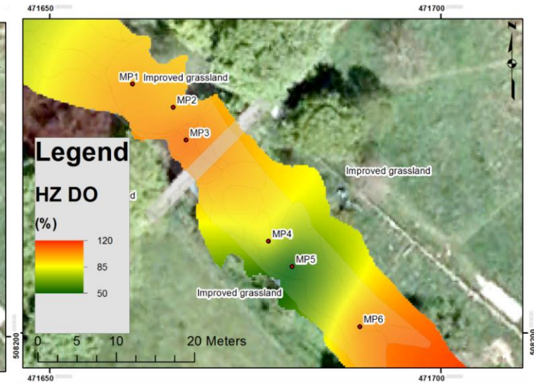
Maps 5.6. Reach-scale spatial variability in average redox and dissolved oxygen (%) across in-stream and hyporheic waters
