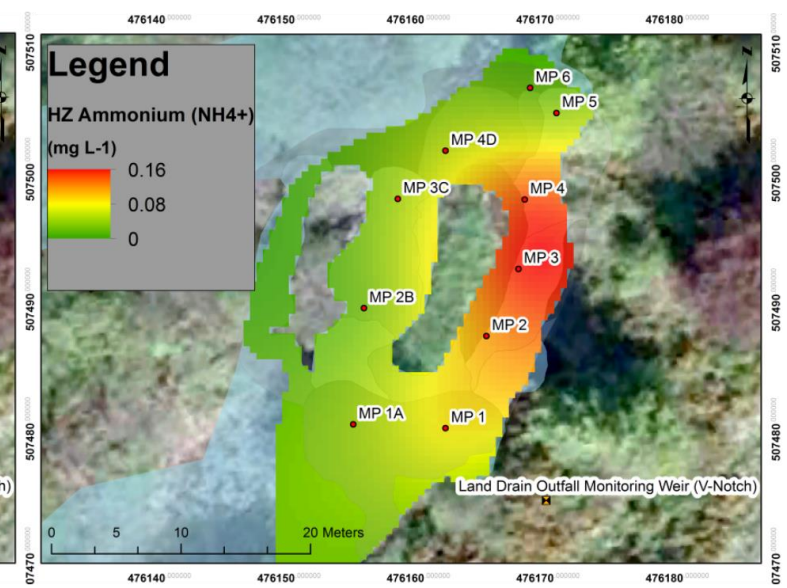
Maps 5.2. Reach-scale spatial variability in average Redox (mV) and Ammonium (NH 4 + ) across in-stream and hyporheic waters
