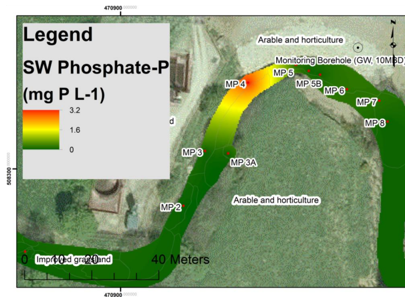
Maps 5.3. Reach-scale spatial variability in average Phosphate-P (Ortho-P) and Nitrate ( NO_3^- ) across in-stream and hyporheic waters
