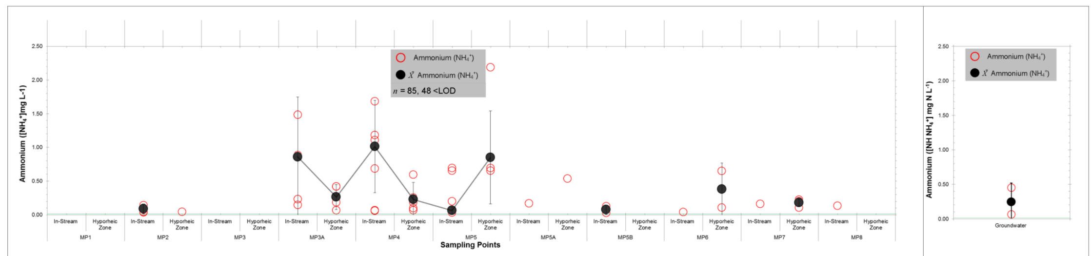
Figure 5.50. Ammonium ( \text{NH}_4^+ ) ( \text{mg L}^{-1} ) dotplot: Data array, arithmetic mean and M. margaritifera respiratory TV Main Channel
