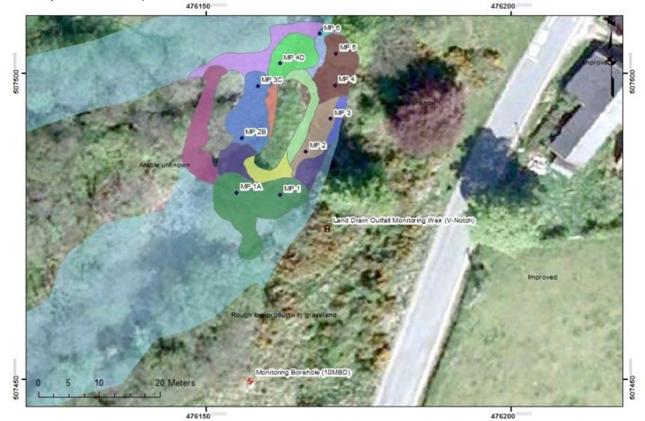
Map 3.7.2. Aerial Perspective: Stream-Unit Demarcation and Land Use
