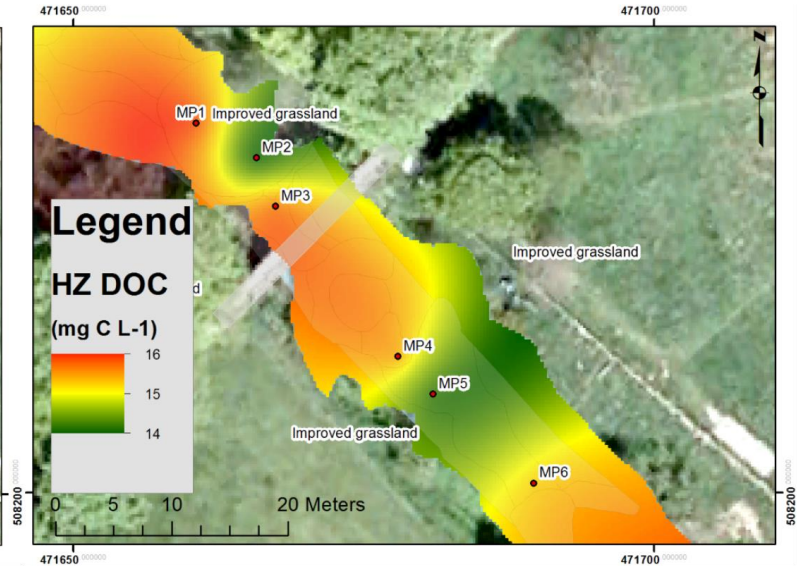
Maps 5.5. Reach-scale spatial variability in average Nitrate ( \text{NO}_3^- ) and DOC across in-stream and hyporheic waters
