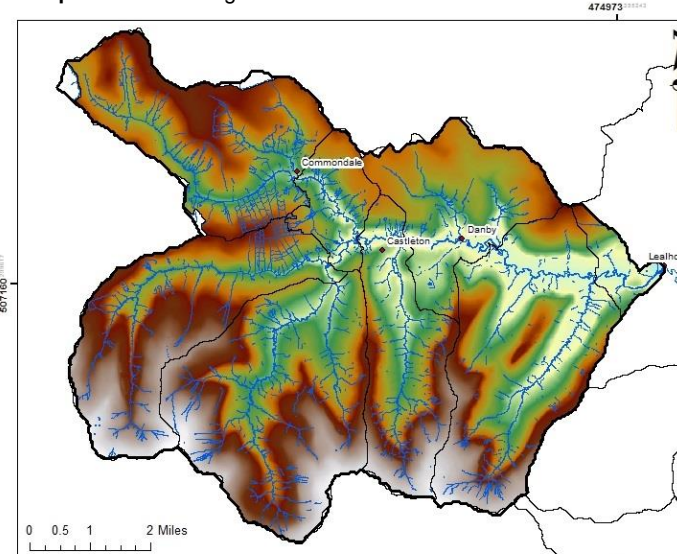
Map 3.5.2. LIDAR: Digital Surface Model
