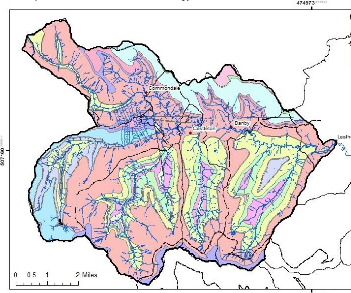
Map 3.5.5. BGS – Bedrock Geology
