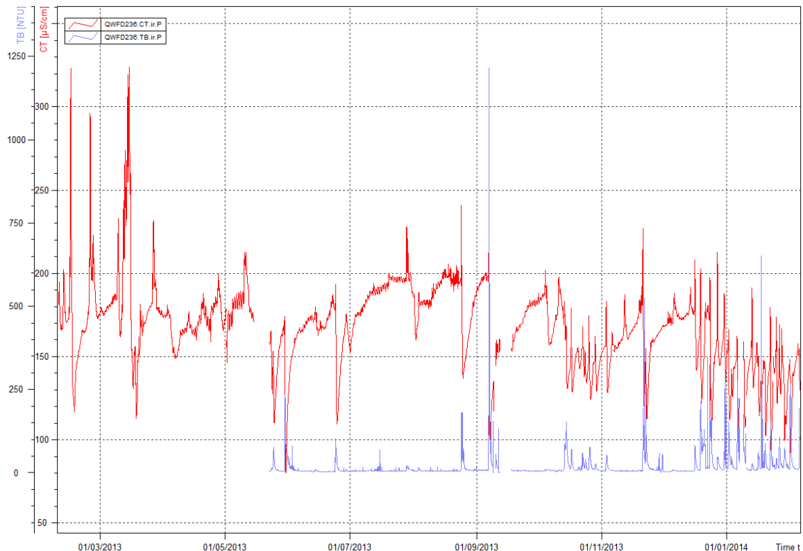
Figure 5.46. Electrical conductivity ( \mu\text{S}/\text{cm} ) proportional to turbidity (NTU)
