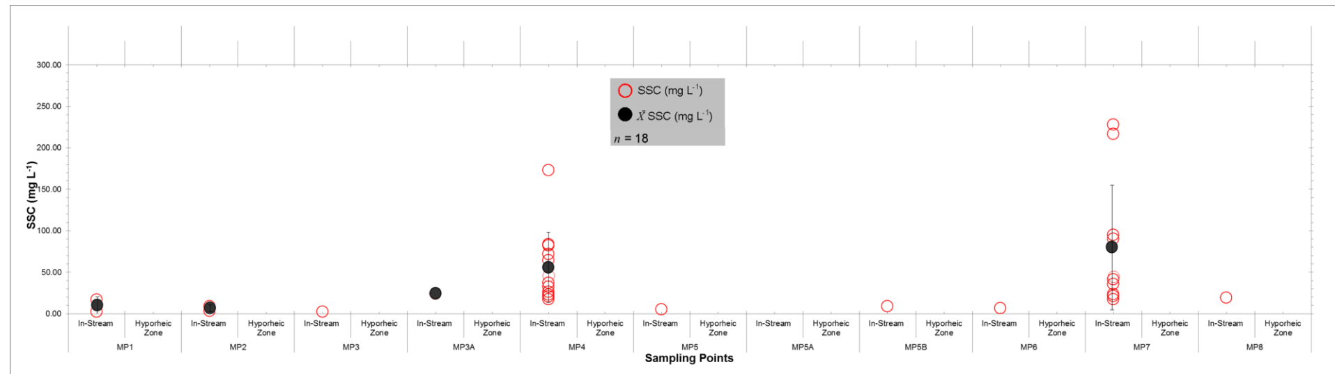
Figure 5.59. Suspended Sediment Concentration (SSC (mg L -1 )) dotplot: Data array and arithmetic mean Main Channel
