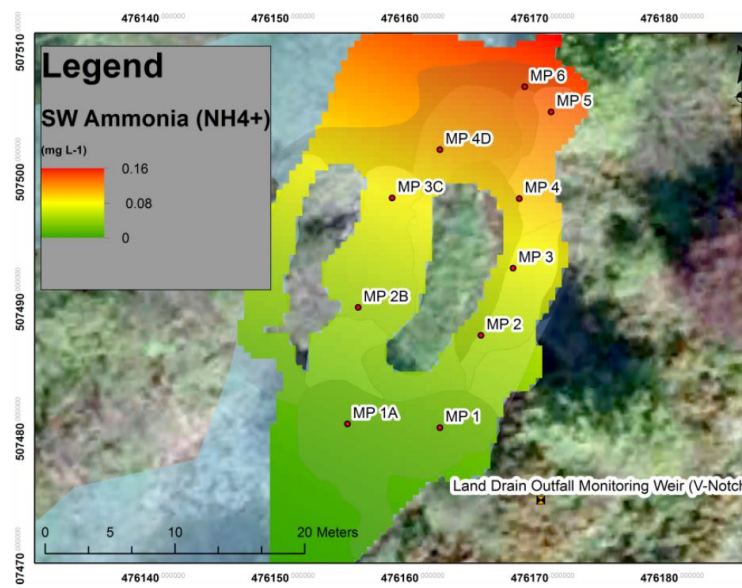
Maps 5.2. Reach-scale spatial variability in average Redox (mV) and Ammonium (NH 4 + ) across in-stream and hyporheic waters
