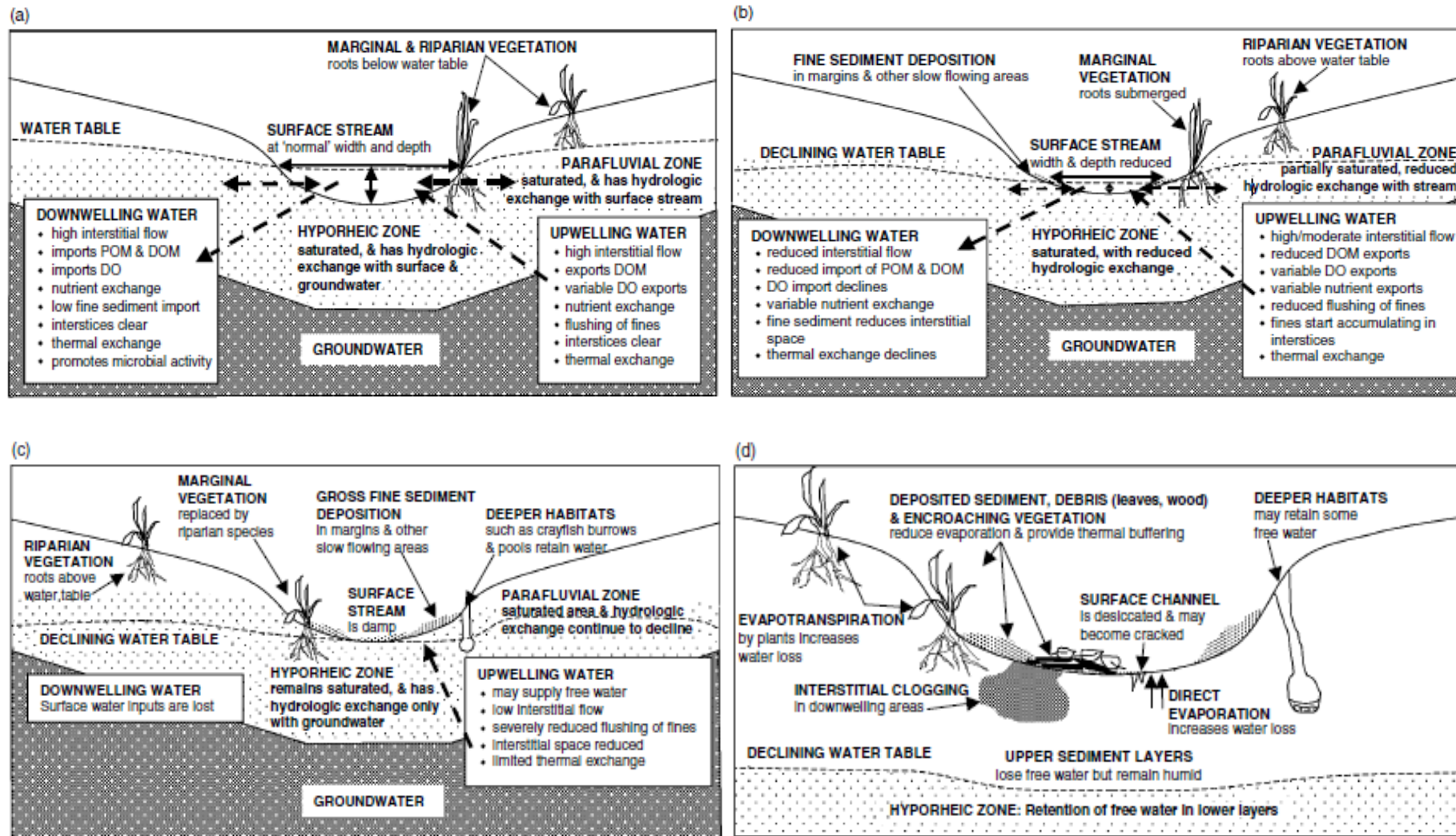
Figure 2.3. Cross-section conceptual model variable flow influences on ecohydrology in the hyporheic zone Source : Stubbington et al. , (2009), Fleckenstein et al. , (2008), Jones (1985)
