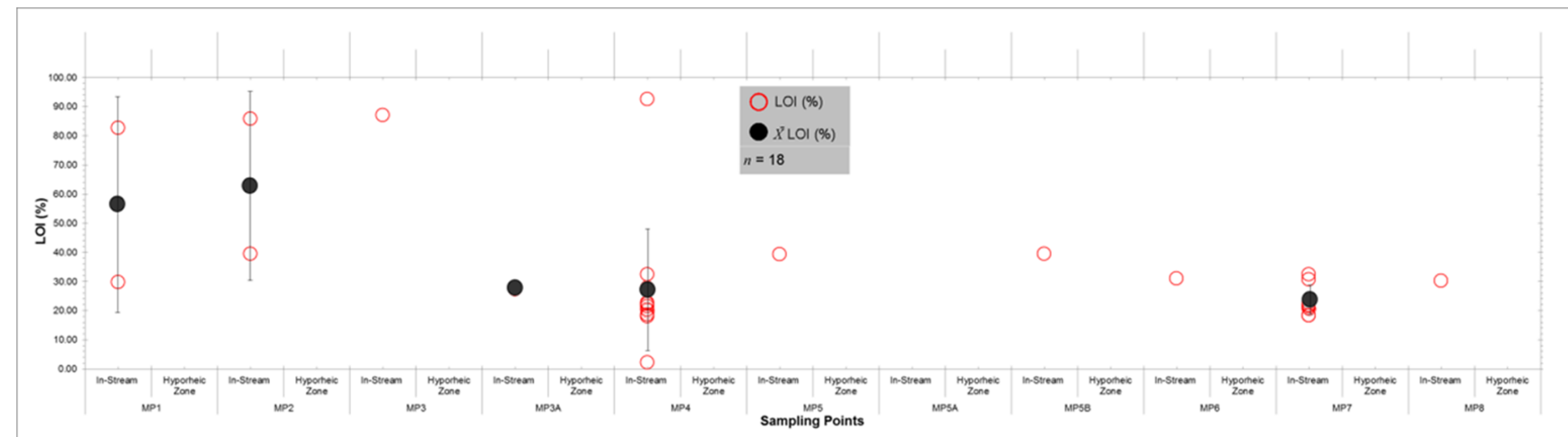
Figure 5.60. Loss-On-Ignition (%) dotplot: Data array and arithmetic mean Main Channel
