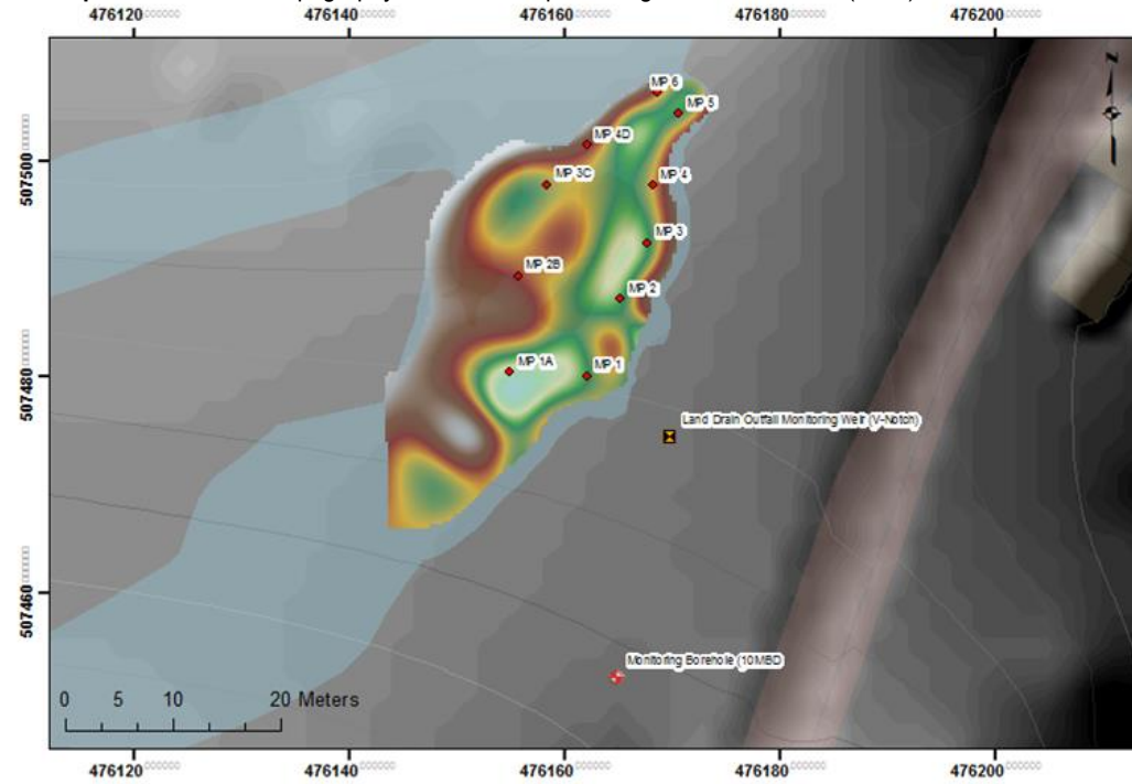
Map 3.7.1. Riverbed Topography and LIDAR Riparian Digital Surface Model (DSM)
