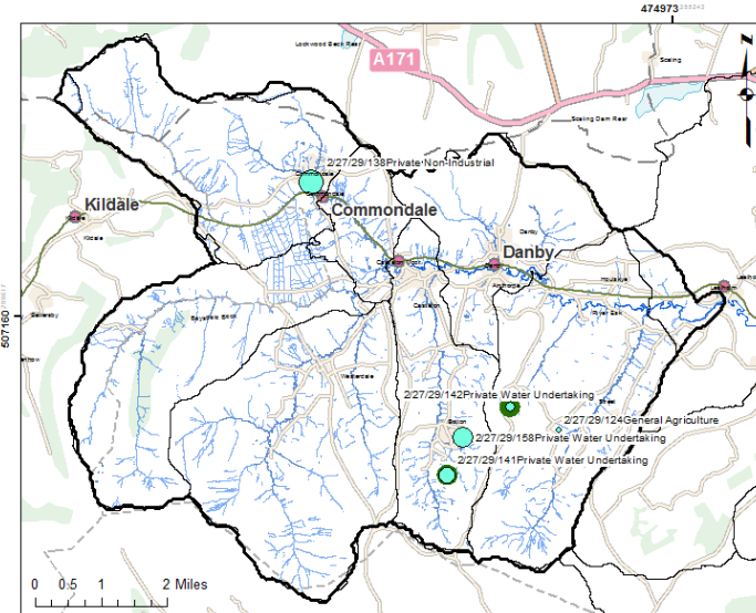
Map 3.5.1. Abstraction and Source Protection Zone Map
