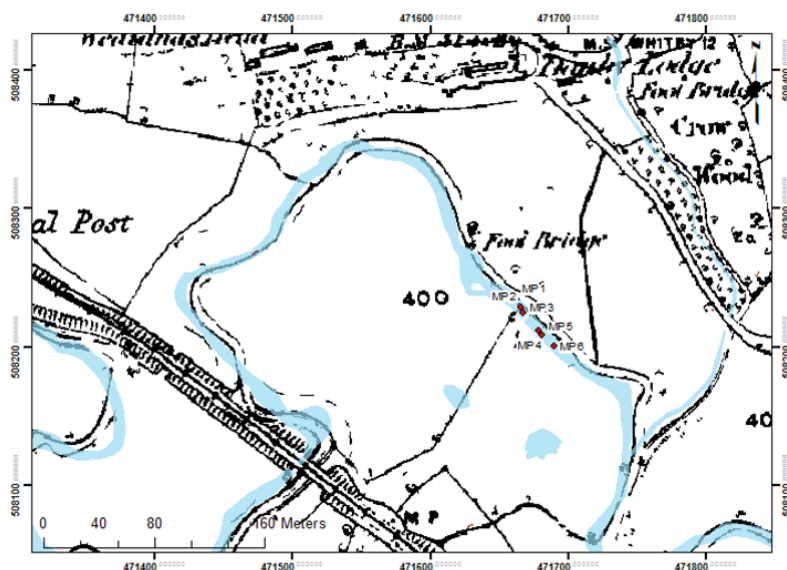
Map 3.9.1 Danby Moors Centre: 1849 and 2013 River Esk Spatial Extents
