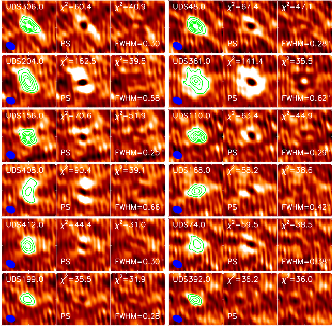
Figure 4.3: Examples showing 2'' \times 2'' images of our high resolution 870 \mu\text{m} maps ( 0.3'' ; left) alongside the residuals from fitting a point source model (PS; middle of each set of three panels) and an elliptical Gaussian model (resolved; right) for 12 example SMGs in our sample. The green contours represent 870 \mu\text{m} emission at 4, 8, 12, \dots \times \sigma , and the colour-scale in each image is clipped at \pm 3\sigma . The ALMA beam is shown in the bottom left of the left-hand column. The SMGs presented here are chosen such that they span the full range in detection significance for the sample, and are a fair representation of the data quality of our ALMA maps. In eleven of these images there are significant residuals when fitting a point source model to the 870 \mu\text{m} emission, indicating that these sources are resolved in our ALMA maps. In contrast we highlight UDS392.0, which is well-described by a point source model and is classed as unresolved in our analysis. For the full sample of 23 SMGs the median difference in \chi^2 between the best-fit extended and point-source model is \Delta\chi^2 = 20 \pm 2 . We find that 22/23 SMGs are resolved in our 0.3'' resolution imaging, and derive a median angular size for the sample of 0.30 \pm 0.04'' (deconvolved FWHM of the major axis).
