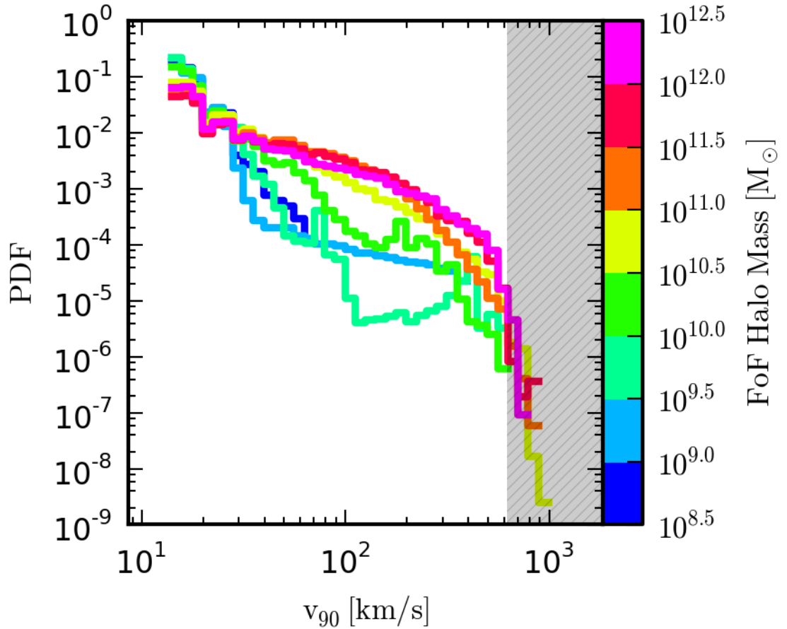
Figure 3.9: The velocity width PDF, binned by halo mass, for our sample of isolated FoF halo projections. Within each mass bin, each halo projection’s PDF is weighted by its total DLA cross section and by an integral of the halo mass function. As implied by figure 3.7, the DLA VWD is halo mass dependant, with low(high) velocity widths being preferentially hosted by low(high) mass halos. However, by isolating each halo, we neglect neutral gas in the IGM and multiple halo intersections / projection effects.
