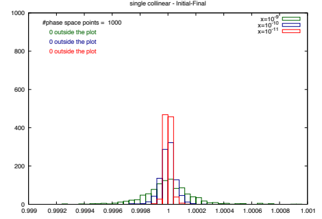
(b) Collinear limit between initial-final partons 1 and i , such that x = s_{1i}/s_{12} approaches zero in the unresolved limit.
