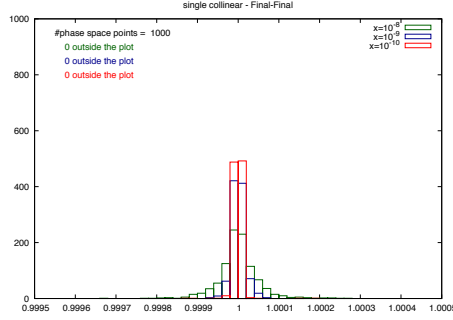
(a) Collinear limit between final-state partons i and j , such that x = s_{ij}/s_{12} approaches zero in the unresolved limit.
