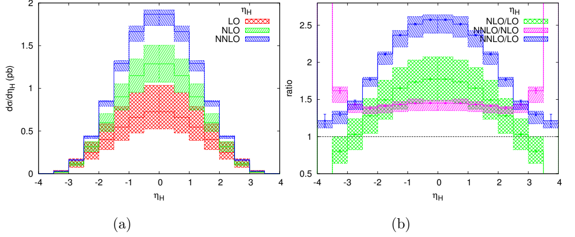
Figure 10.3: (a) Rapidity distribution of the Higgs boson in inclusive H + jet production in pp collisions with \sqrt{s} = 8 TeV at LO, NLO, NNLO and (b) Ratios of different perturbative orders, NLO/LO, NNLO/LO and NNLO/NLO.
