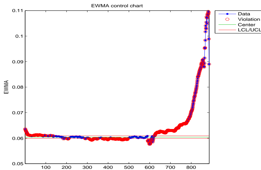
Figure B.65: EWMA chart for the 75 th percentile of the healthy bearing.
