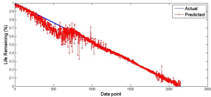
Figure 6.22: Refined RUL estimation of bearing 3 (training dataset).
