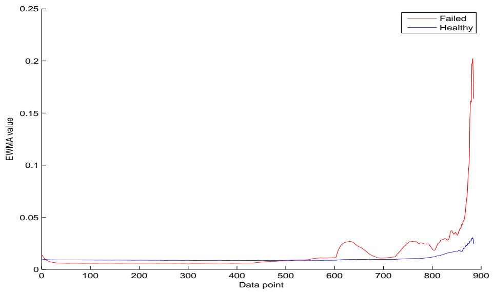
Figure B.24: Variance over time of the failed and healthy bearing.
