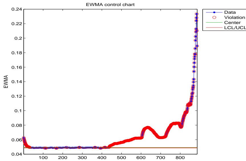
Figure B.64: EWMA chart for the 75 th percentile of the failed bearing.
