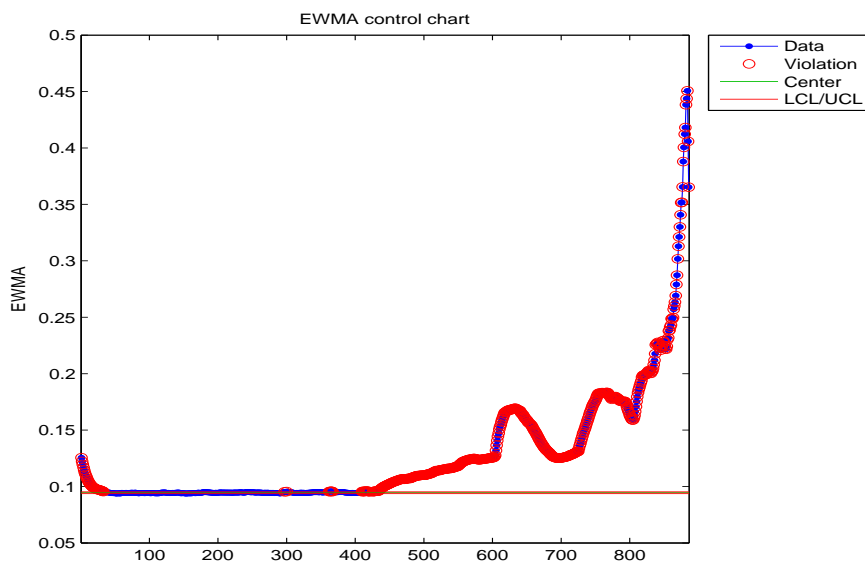
Figure B.67: EWMA chart for the 90 th percentile of the failed bearing.
