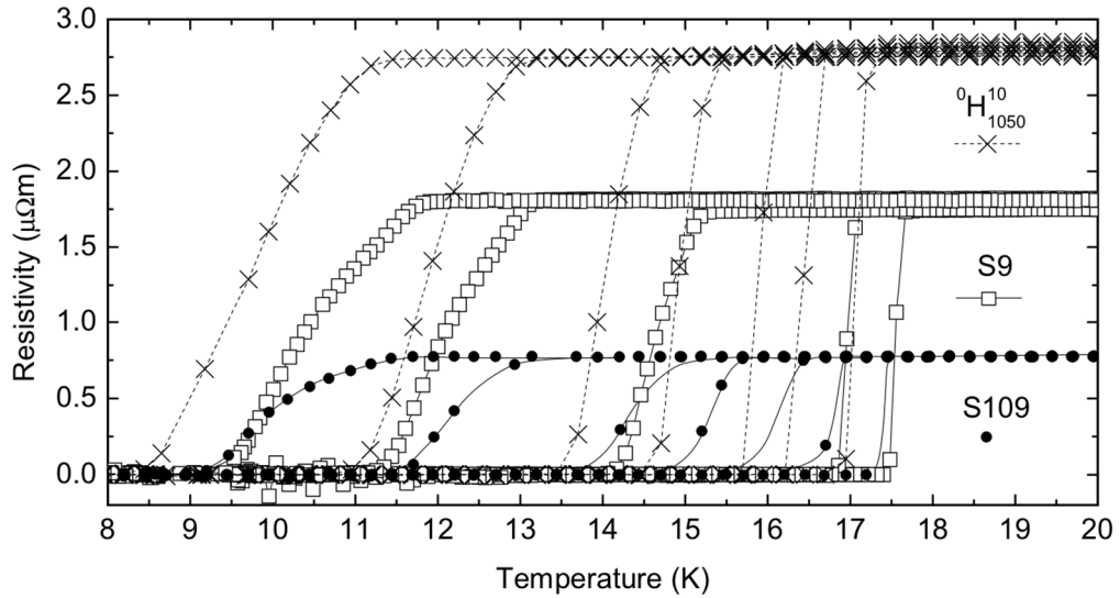
Figure 5.1: Normal state resistivity data of three microcrystalline samples. Samples S9 and S109 (see Table 4.1) are sintered samples and sample {}^0H_{1050}^{10} is a sintered sample that was HIPed for ten minutes at 1050 °C and at 2000 bar. Samples S109 and {}^0H_{1050}^{10} were measured in applied fields 0, 0.5, 1.0, 2.0, 3.0, 5.5 and 8.0 T. Sample S9 was measured in applied fields, 0, 0.5, 3.0, 6.0 and 8.0 T. The lines are guides to the eye.
