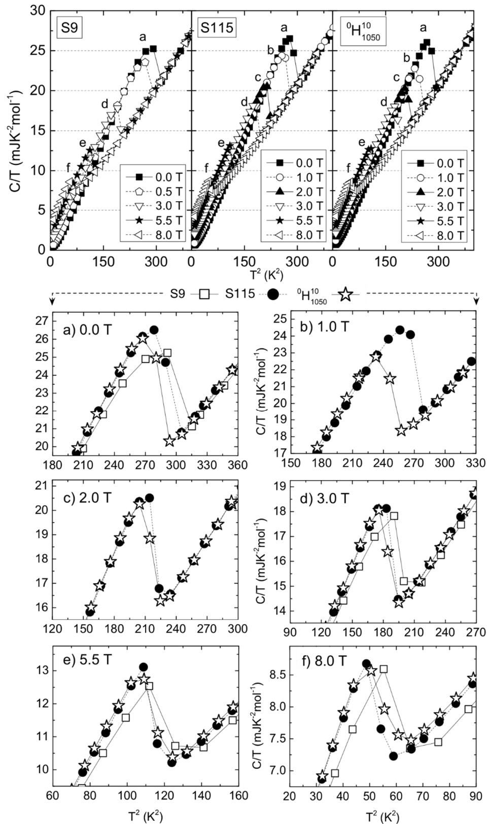
Figure 5.5: Debye plots of the sintered samples S9 and S115 and the HIPed sample {}^0H_{1050} in applied magnetic fields 0 to 8.0 T. The data for each of the fields 0, 1.0, 2.0, 3.0, 5.5 and 8.0 T are independently shown in plots a) to f) respectively.
