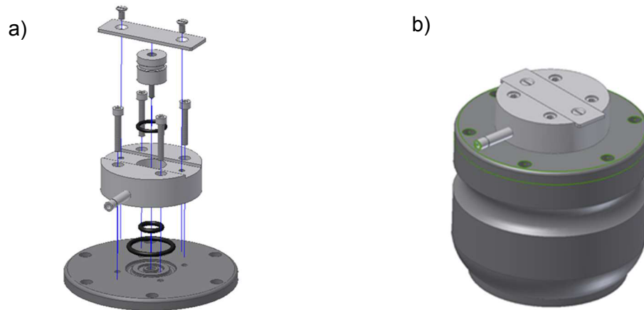
Figure 4.17: The modified Nb vial. a) Exploded view of the valve assembly – all parts were machined from stainless steel 316L. b) Fully assembled vial and valve.
