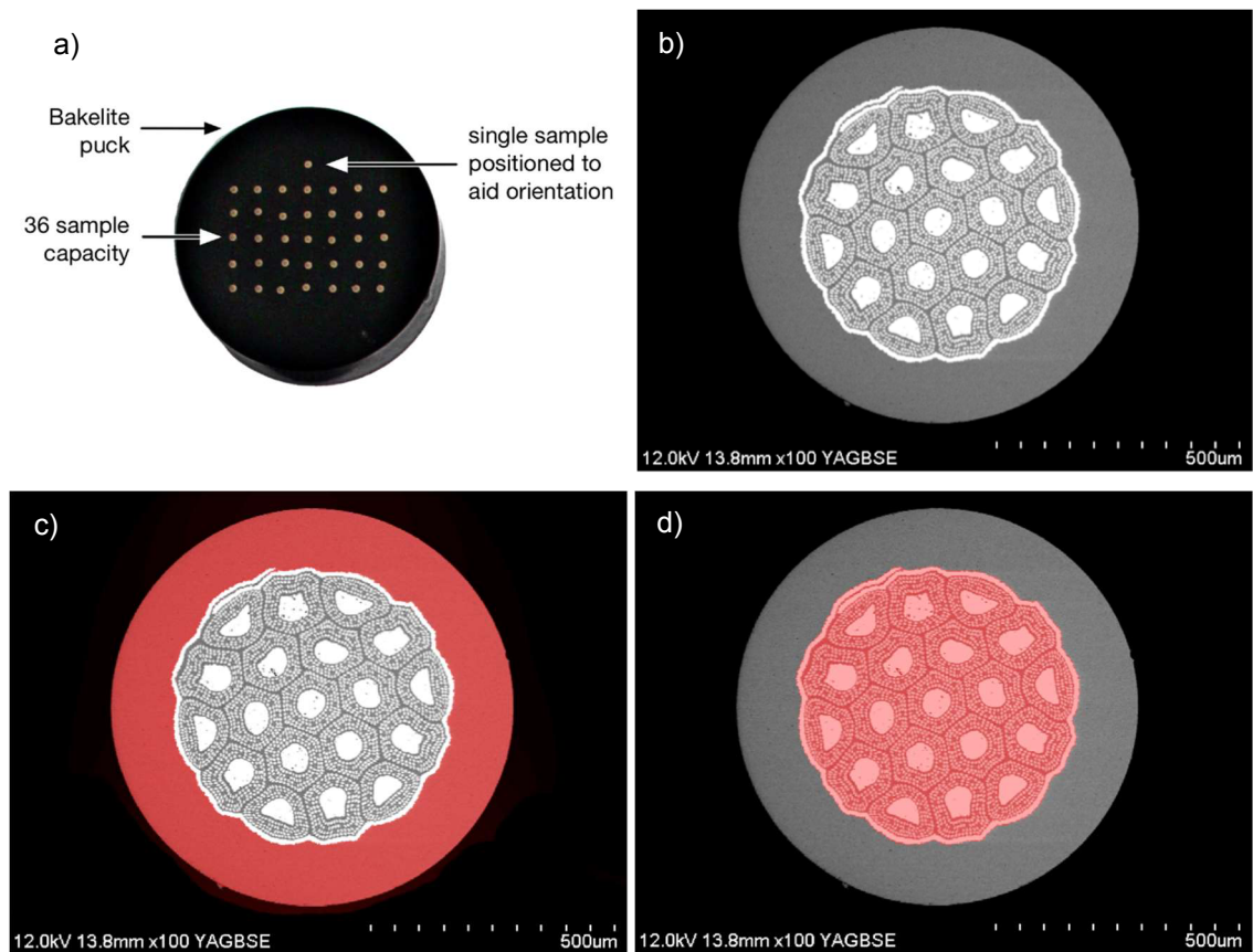
Figure 6.36: Copper to non-copper ratio; a) mounting puck (Bakelite) used to image the cross-sections of up to 36 samples with the SU-70 FEG SEM, b) example image, c) copper region highlighted, d) non-copper region highlighted.
