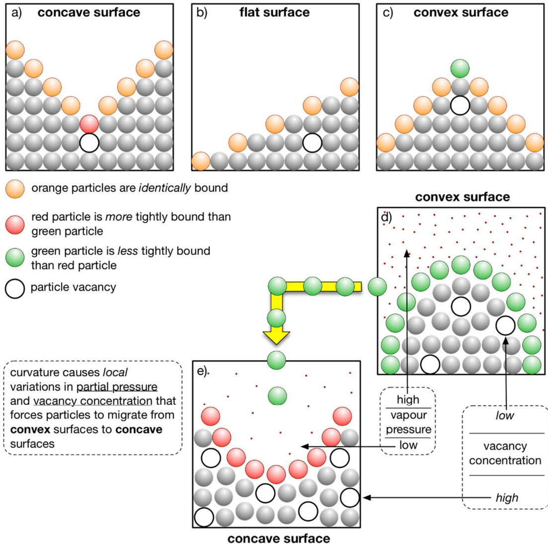
Figure 4.19: Three surfaces each enclosed within a sealed, evacuated, container; a) a concave surface, b) a flat surface, and c) a convex surface. Each container is heated until an equilibrium vapour pressure is obtained within. The red particle (box (a)) is more tightly bound than the green particle (box (c)) and therefore the partial pressure within box (c) is greater than that in box (a) due to the ease with which the green particle can leave its convex surface. These three boxes also show that it is easier for vacancies to form under the concave surface (box (a)) than under the convex surface (box (c)). This is because the difference in the binding energies of the vacancies and their respective surface particles is less under the concave surface (box (a)) than the convex surface (box (c)). Boxes (d) and (e) summarise the discussion given in the text. (Figure adapted from [126].)
