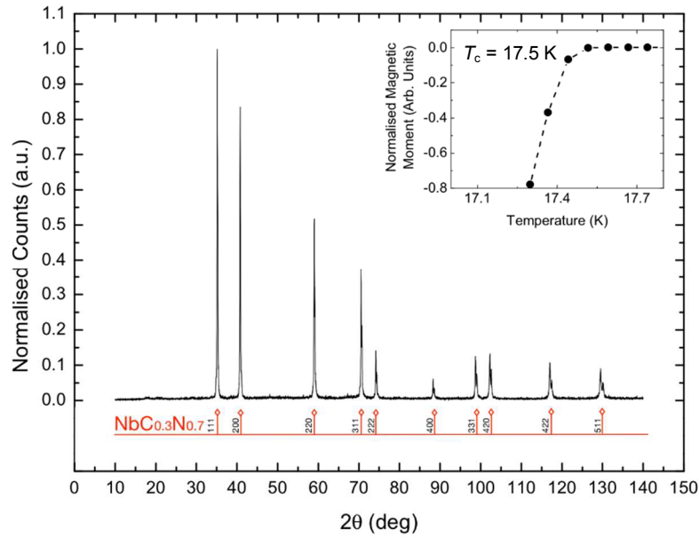
Figure 4.9: Typical XRD data of fabricated \text{NbC}_{0.3}\text{N}_{0.7} . These XRD data were taken from measurements conducted on pellet 6 of sintered batch 1 material, SB_6^1 , (see Table 4.2). The red lines with open symbols indicate the expected peak positions for \text{NbC}_{0.3}\text{N}_{0.7} [118]. The inset shows the zero field magnetic susceptibility data from which the onset of T_c was obtained.
