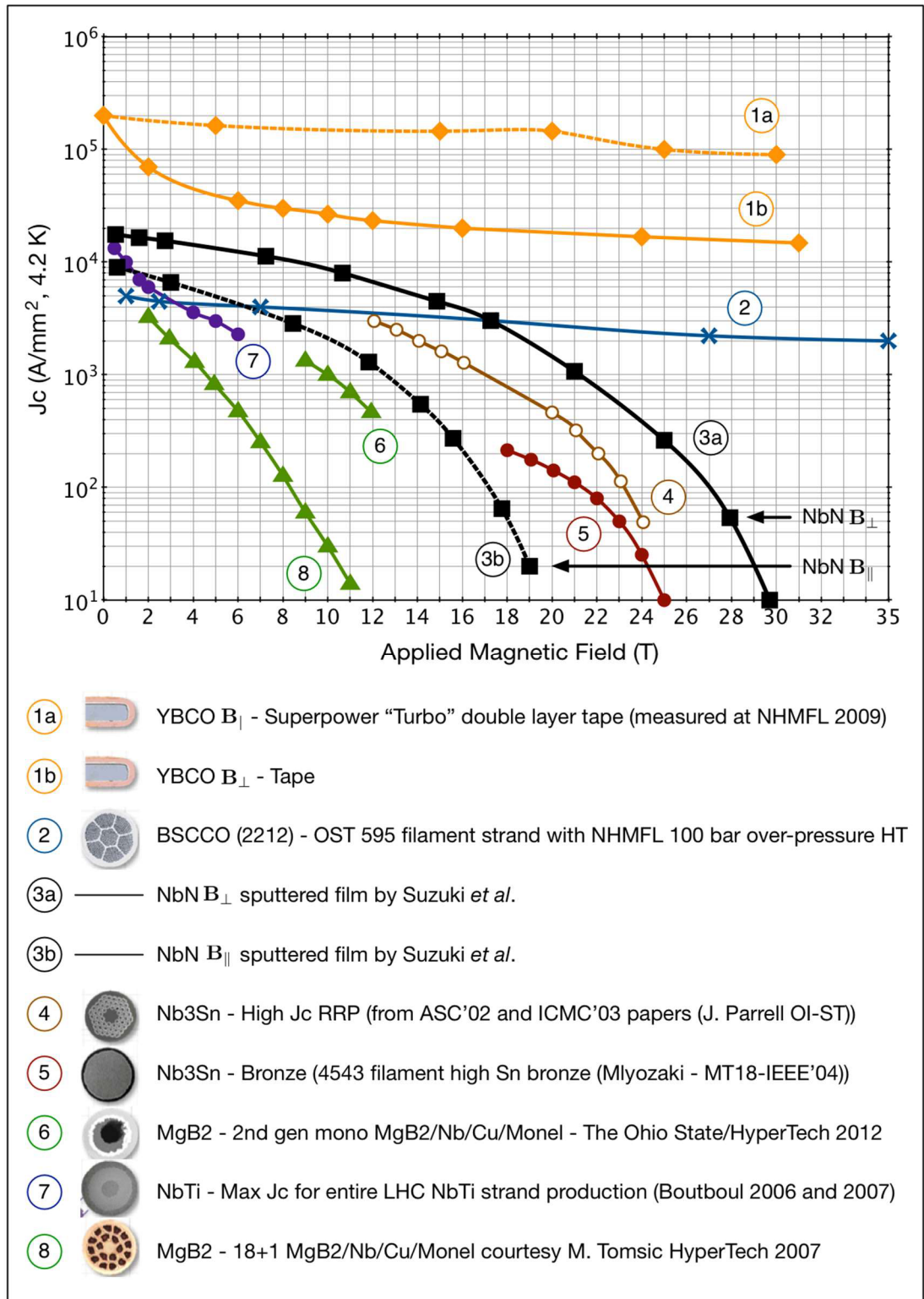
Figure 3.27: The critical current density as a function of applied magnetic field for a number of Type II superconductors. The black square symbols represent the NbN sputtered film in two orientations in accord with the findings of Suzuki et al. [111]. (Graph adapted from [112].)
