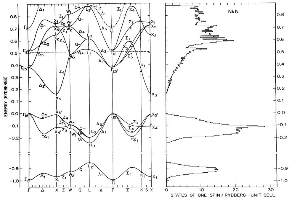
Figure 3.4: Band structure and density of states of niobium nitride [70]. The dashed horizontal line represents the Fermi energy for stoichiometric niobium nitride.
