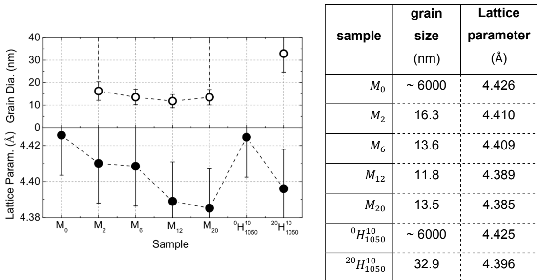
Figure 4.23: Comparison between grain size and lattice parameters of milled samples M_0 to M_{20} to HIPed samples {}^0H_{1050}^{10} and {}^{20}H_{1050}^{10} . The values for each dimension are tabulated on the right. The grain sizes for samples M_0 and {}^0H_{1050}^{10} are too large to be plotted in the figure but the tabulated data shows that their grain size is approximately the same.
