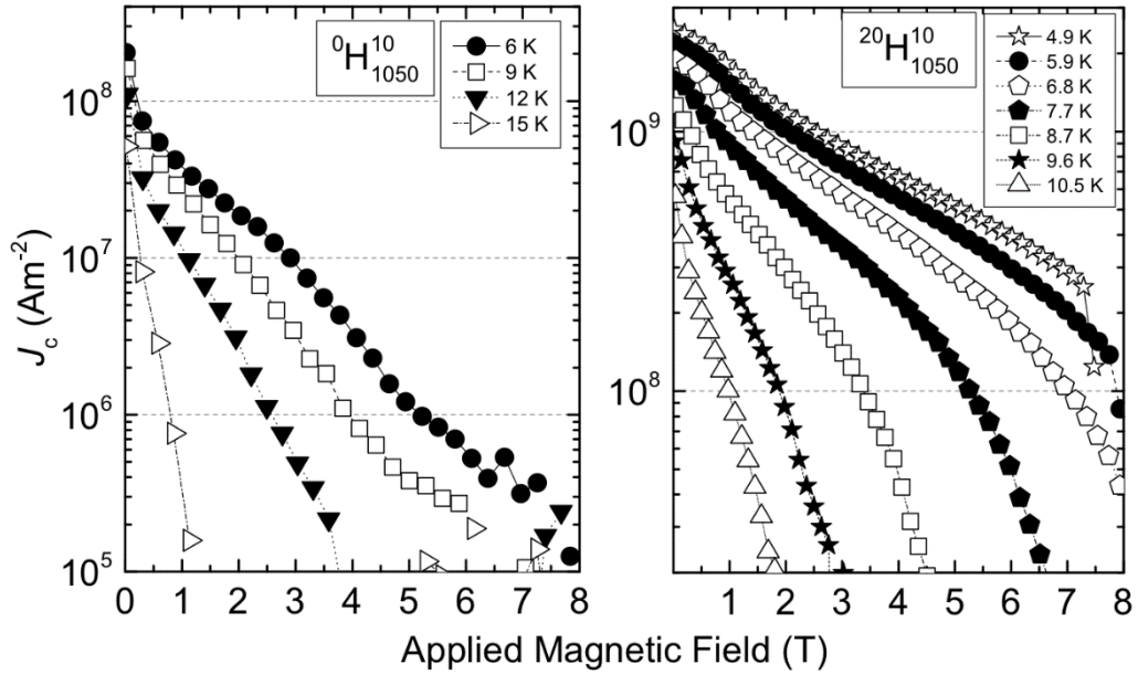
Figure 5.14: Critical current density as a function of applied magnetic field of the nanocrystalline sample, ^{20}\text{H}_{1050}^{10} (in the temperature range 4.9 to 10.5 K), and the microcrystalline sample, ^0\text{H}_{1050}^{10} (in the temperature range 6 to 15 K).
