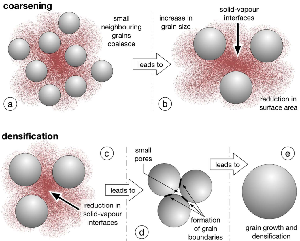
Figure 4.3: The two main processes that drive solid-state sintering are coarsening and densification . (a) The coalescence of small neighbouring grains leads to (b) increases in grain size and reductions in surface areas that produce a coarsened , porous bulk. (c) Reductions in solid-vapour interfaces lead to (d) grain boundary and small pore formation that produce (e) grain growth and densification .
