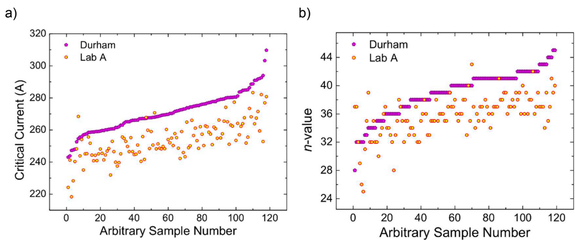
Figure 6.13: Comparison of the critical currents (a) and n -values (b) of a set of internal tin strands independently heat-treated and measured by Durham and Lab A.
