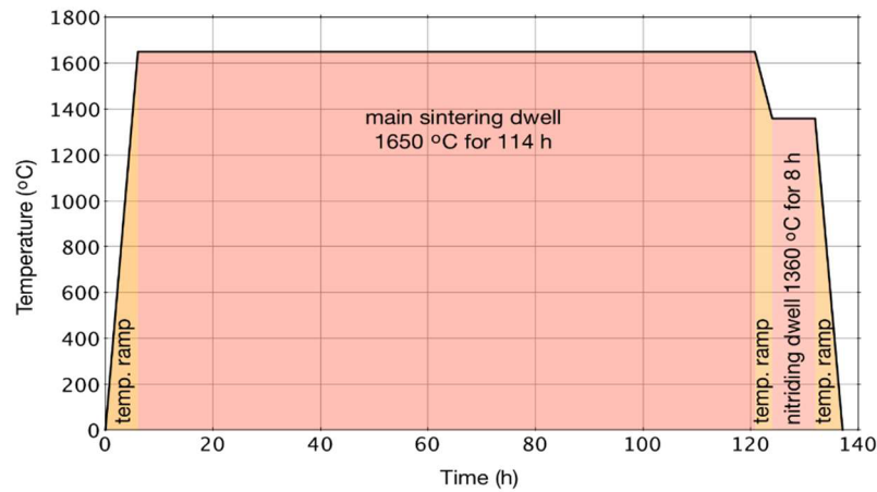
Figure 4.5: Heat-treatment profile for sintering NbC 0.3 N 0.7 sample pellets in a flowing nitrogen atmosphere. Temperature program; ramp to 1650 °C at 264 °C/h and dwell for 114 hours, ramp to 1360 °C and dwell for 8 hours, switch off heaters.
