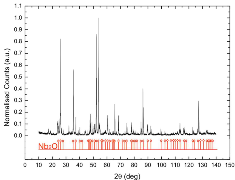
Figure 4.6: Typical XRD data of the crust that forms around the surface of the \text{NbC}_{0.3}\text{N}_{0.7} sample pellets during solid state sintering (without gas guard). The red lines with open symbols indicate the expected peak positions for \text{Nb}_2\text{O} (obtained from [116]).
