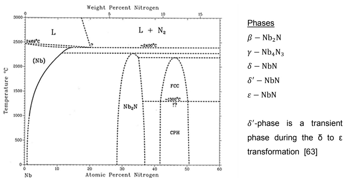
Figure 3.1: Phase diagram of niobium nitride [64], supplemented from [56, 65-69]. The \delta -phase structure is the one of interest in this review.
