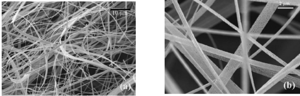
Figure 3.17: Scanning electron micrographs of the nanowires and nanoribbons produced by Patel et al. Image (a) is low magnification and image (b) is high magnification [98].
