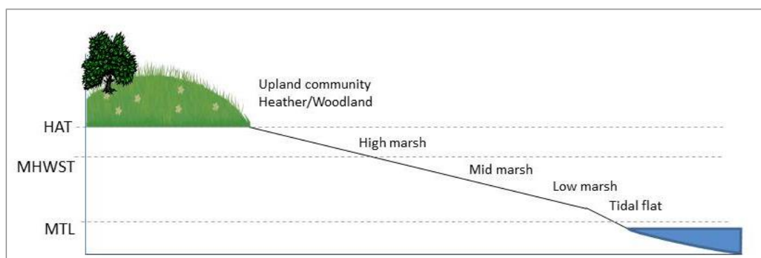
Figure 2.1: Schematic diagram of a salt-marsh environment showing zonation and reference water levels. (HAT – Highest Astronomical Tide, MHWST – Mean High Water Spring Tides, MTL – Mean Tide Level)
