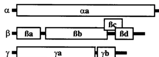
Figure 1: A schematic diagram of BSMV \alpha RNA, \beta RNA and \gamma RNA. \alpha a gene encodes for a helicase. \beta a encodes for the coat protein. \beta b , \beta c and \beta d encode for proteins involved in viral movement. \gamma a encodes for the RNA polymerase and \gamma b encodes for a RNA binding protein involved in pathogenecity (Holzberg et al 2002). Figure modified from Holzberg et al 2002.
