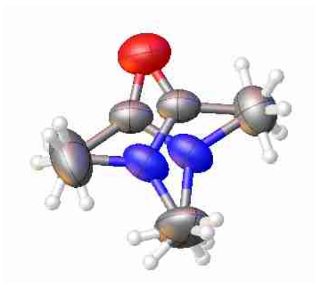
Figure 6.16 Asymmetric unit of cryo-crystallised dimethylacetamide.
