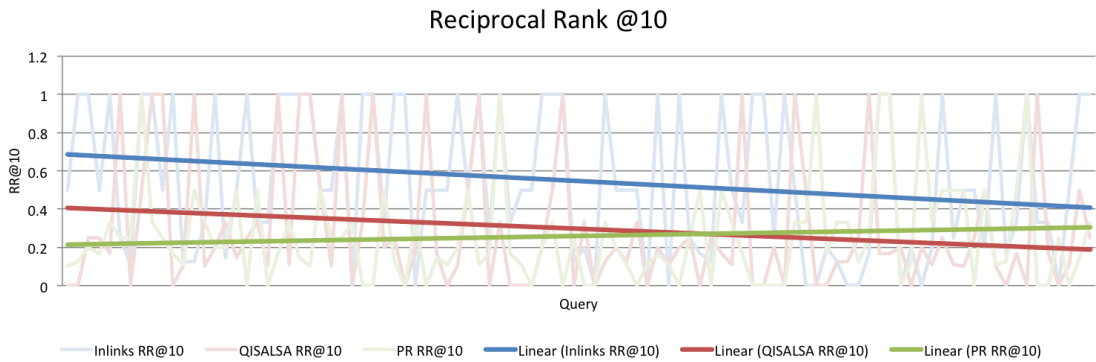
Figure 4.7: Trend of Reciprocal rank @10 for each query
