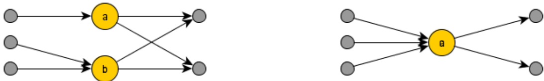
Figure 2.2: Collapsing axiom
