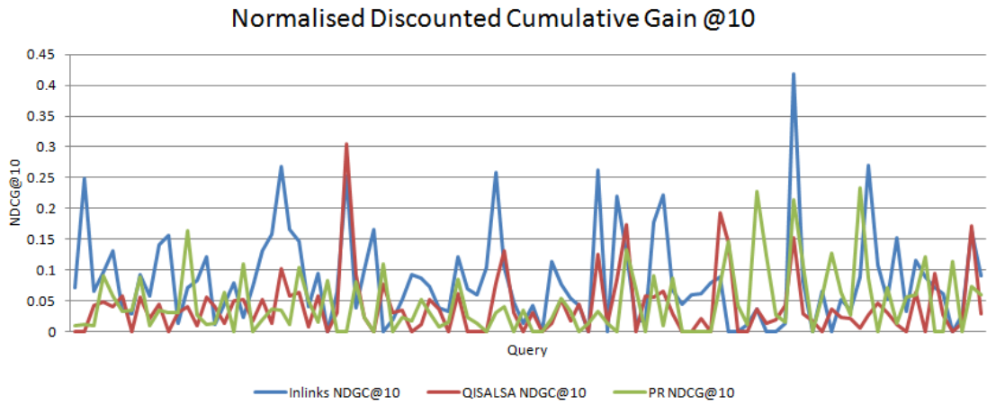
Figure 4.2: Normalized discounted cumulative gain @10 for each query
