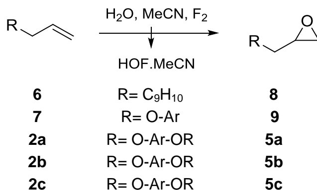
Scheme 6.14 – General reaction for epoxidation of alkenes using HOF.MeCN
