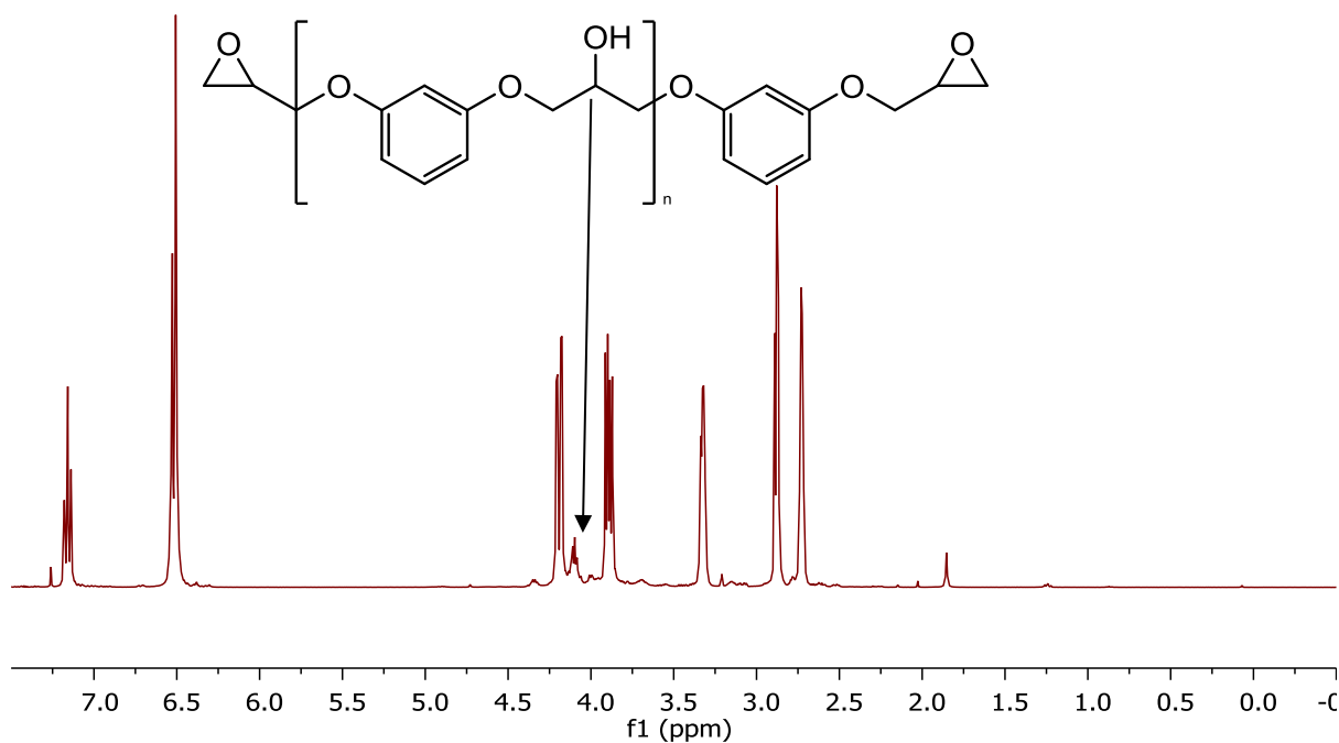
Figure 4.2 – ^1\text{H} NMR spectrum for impure resorcinol diglycidyl ether
