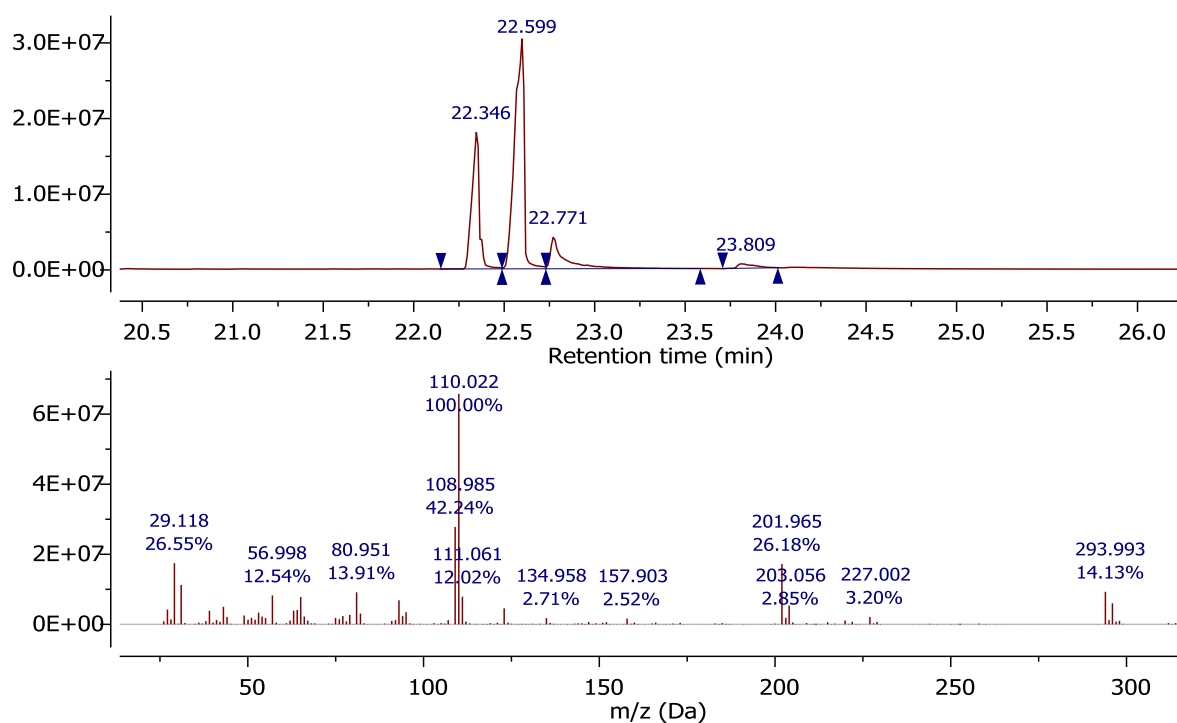
Figure 2.15 – GC-MS spectrum for hydroquinone dichlorohydrin ether. The selected mass spectrum is for peaks 22.35; 22.60 and 22.77 min which relate to the mass of the desired product. The mass peak of 110.0 m/z relates to hydroquinone which occurs due to fragmentation.
