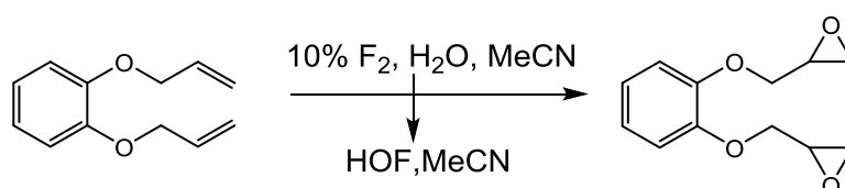
Scheme 3.4 – Conversion of catechol diallyl ether to the epoxide using HOF.MeCN prepared in ‘batch’.
