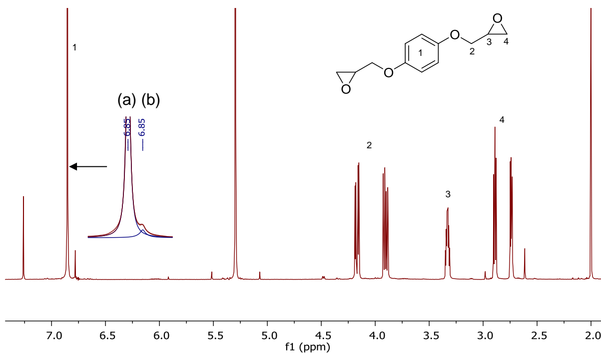
Figure 3.5 – ^1\text{H} NMR spectrum for hydroquinone diglycidyl ether after 30 mins collection of HOF.MeCN
