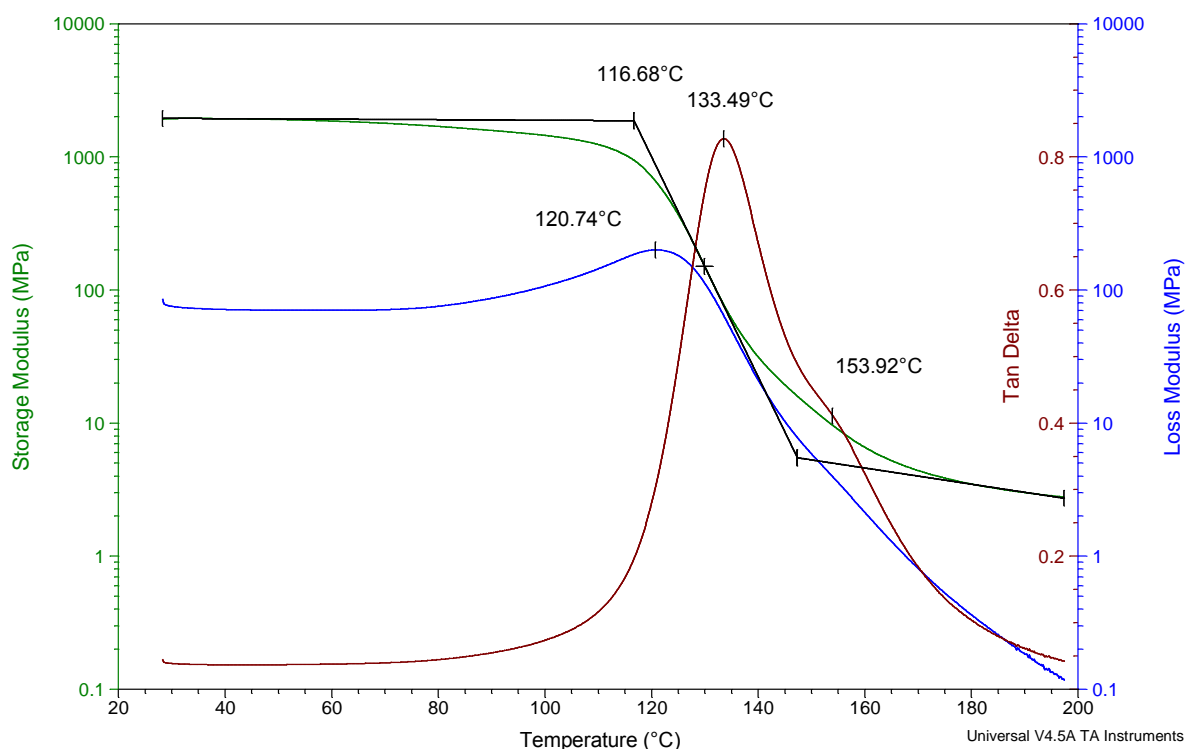
Figure 5.10 – DMTA graph for HDGE and L-PACM polymer films..
