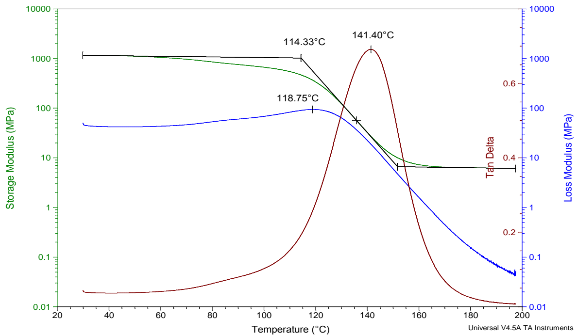
Figure 5.9 – DMTA plot for HDGE and L-PACM polymer films.
