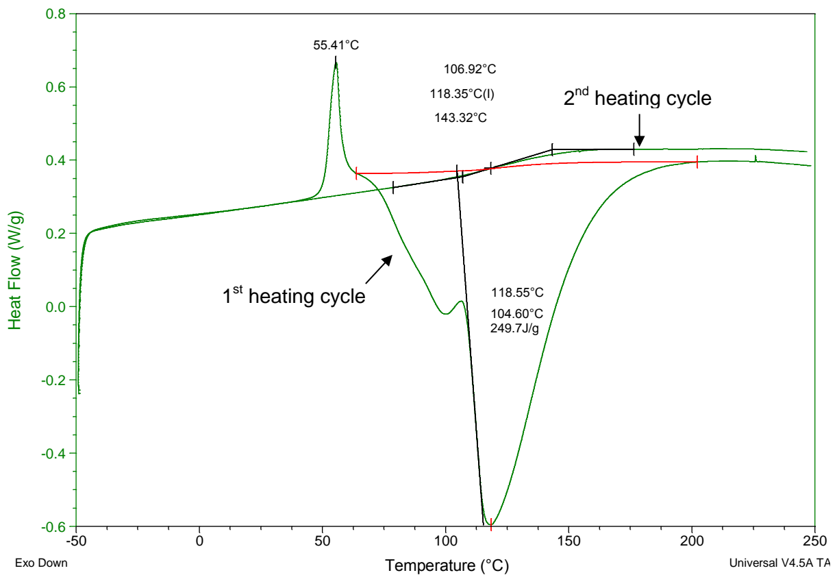
Fig 4.23 – DSC graph for kinetic study of HDGE with L-PACM
