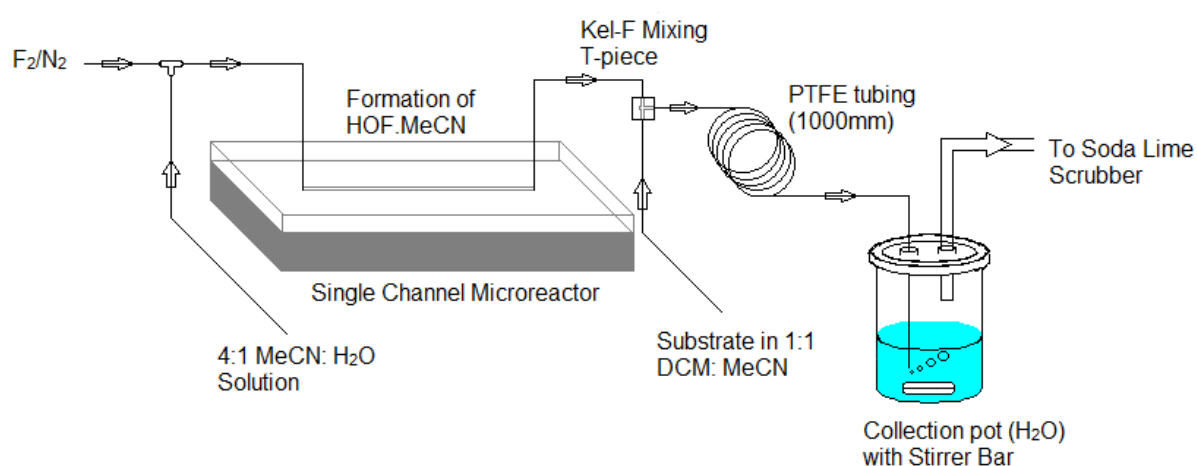
Figure 3.8 – Continuous flow experimental set-up
