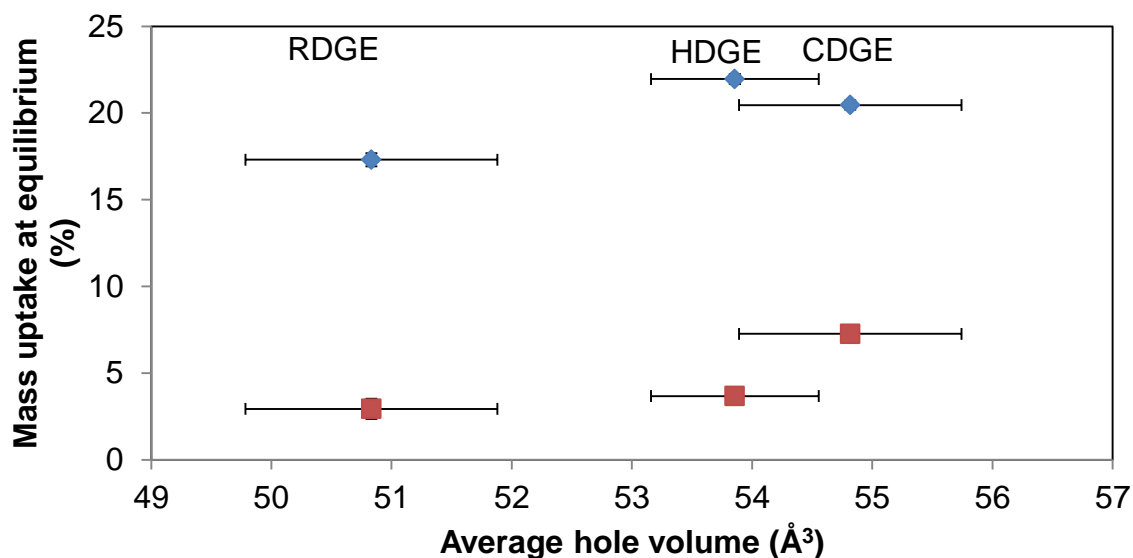
Figure 5.20 – Graphic representation of solvent uptake versus average hole volume.
