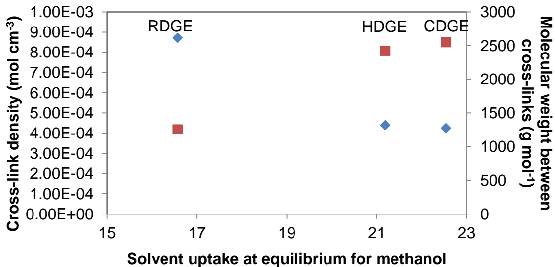
Figure 5.19a – Plot of methanol uptake versus \vartheta_e and M_c . \blacklozenge \vartheta_e ; \blacksquare M_c
