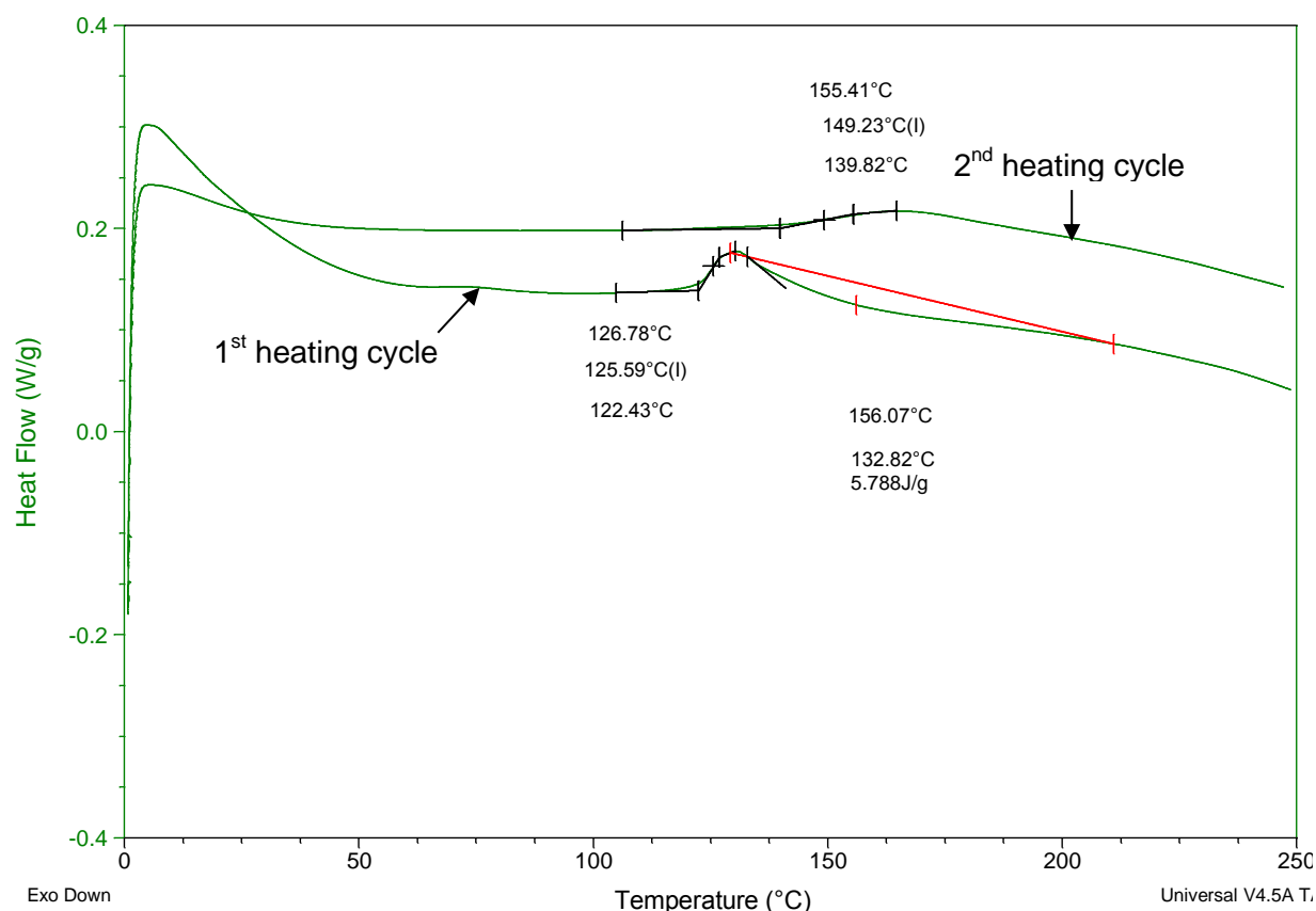
Figure 4.22 – DSC graph for the initial cure of HDGE at 110°C
