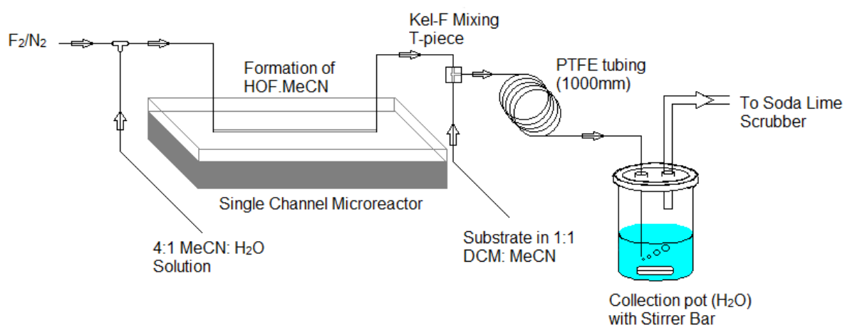
Figure 6.2 – Reaction set up for continuous flow HOF.MeCN reactions
