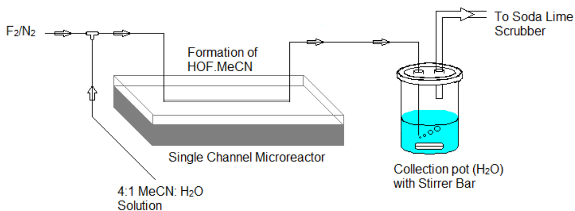
Figure 3.2 – Experimental set up for batch epoxidation using HOF.MeCN
