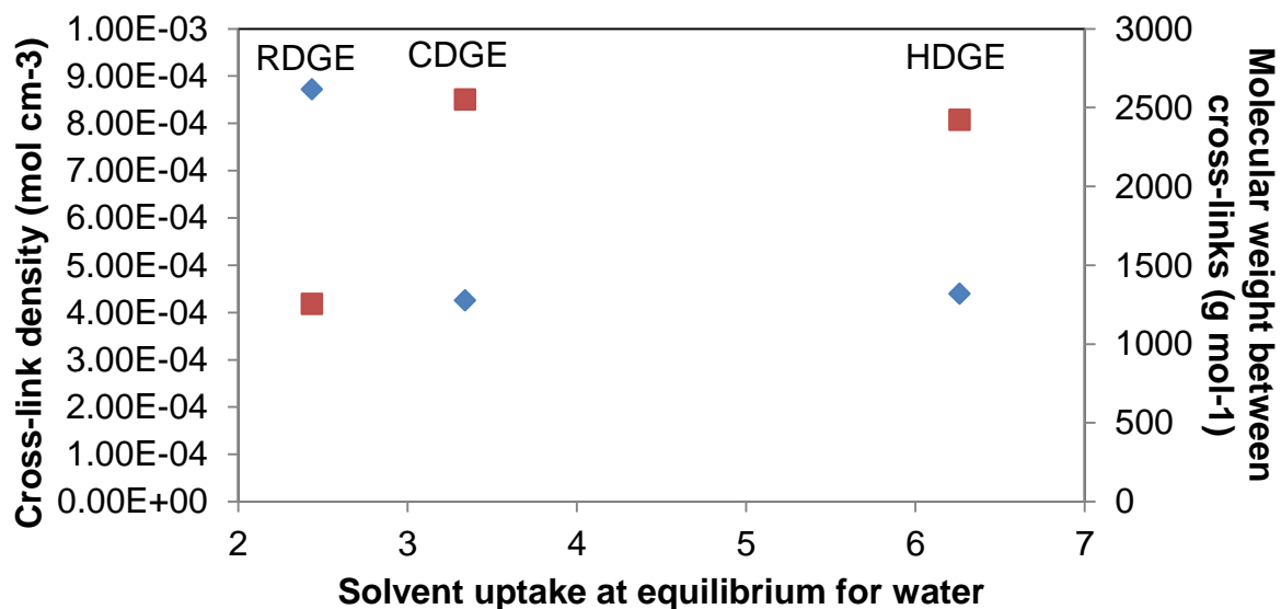
Figure 5.19b – Plot of methanol uptake versus \vartheta_e and M_c . \blacklozenge \vartheta_e ; \blacksquare M_c
