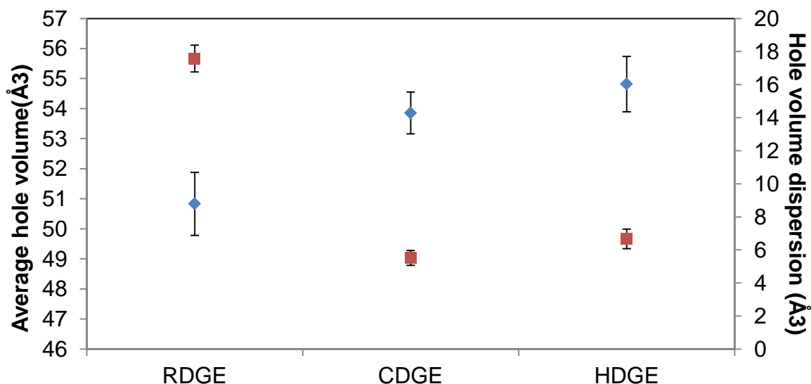
Figure 5.11 – Graphic representation of results from positron annihilation spectroscopy: \blacklozenge is average hole volume; \blacksquare is hole volume dispersion.
