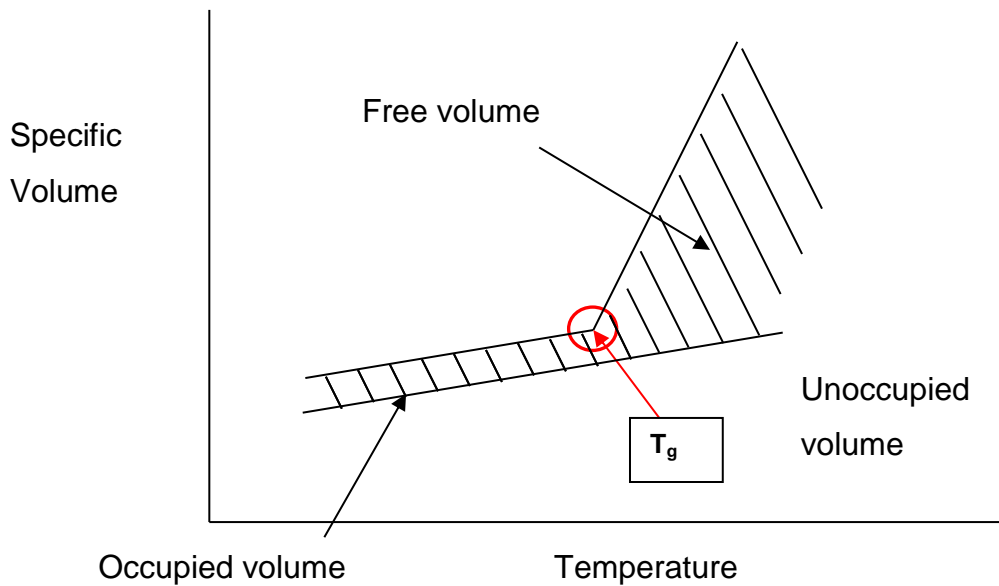
Figure 1.7 – Effect of the T_g on the specific volume
