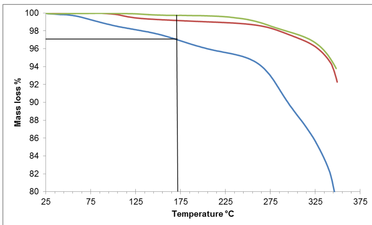
Figure 4.29 – TGA results for all of the epoxides to determine a cure temperature that does not degrade the polymers. – RDGE; – HDGE and – CDGE, the line relates to less than 3% degradation of CDGE.
