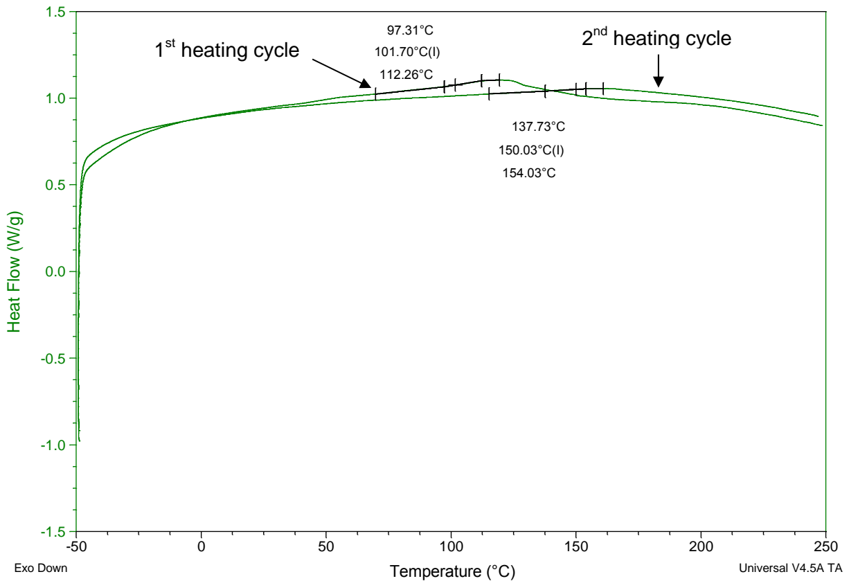
Figure 4.25 – DSC graph for HDGE with L-PACM cured at 110°C for 20 hours.
