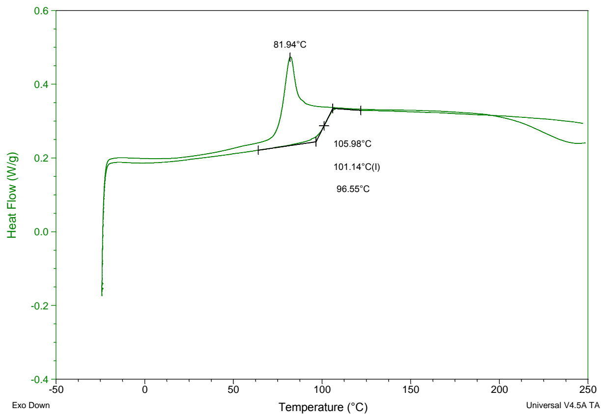
Figure 4.27 – DSC graph for CDGE with L-PACM cured at 60°C for 18 hours
