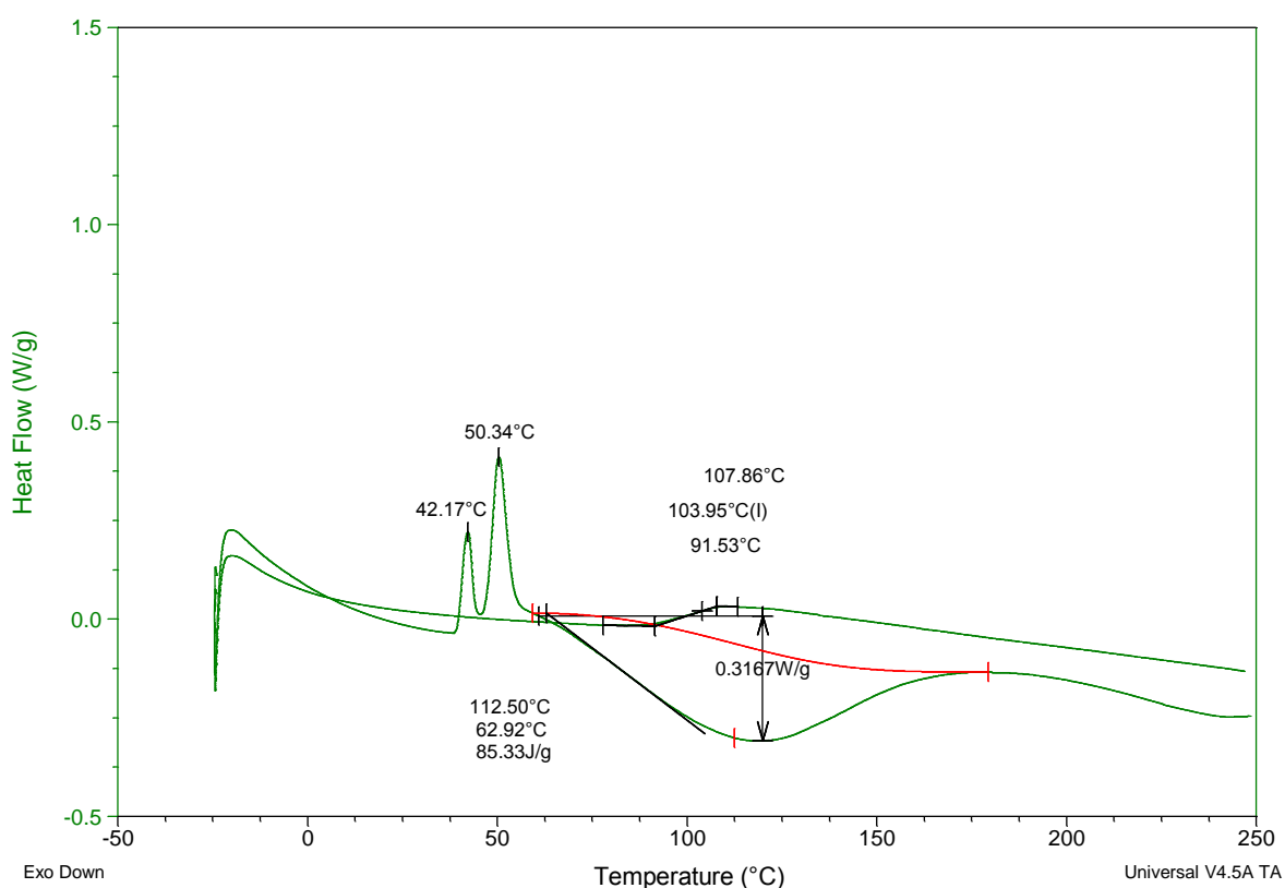
Figure 4.26 – DSC graph for kinetic study of CDGE with L-PACM
