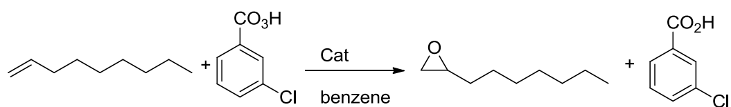
Scheme 1.4 – epoxidation of 1-nonene with m -chloroperbenzoic acid
