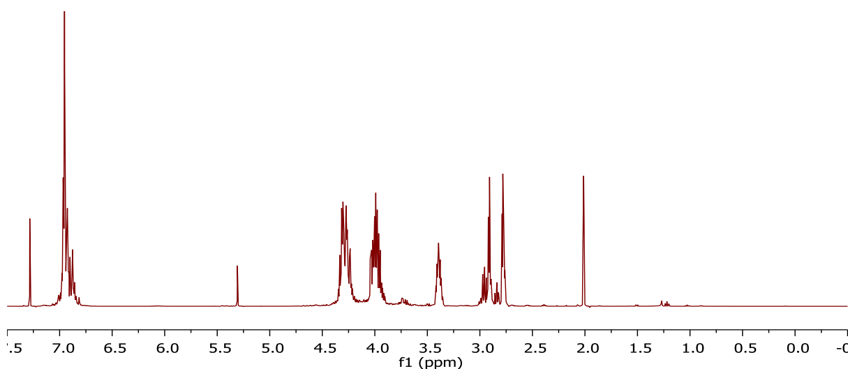
Figure 2.22 – 1 H NMR for catechol diglycidyl ether after 3.5 molar equivalents of potassium hydroxide. The peaks at 2.16 and 5.29 ppm correspond to acetone and dichloromethane respectively.
