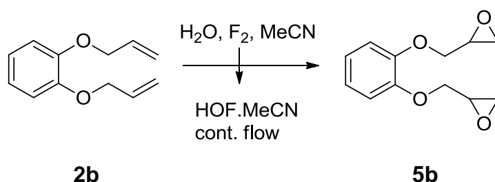
Scheme 6.22 – Epoxidation of catechol diallyl ether using HOF.MeCN
