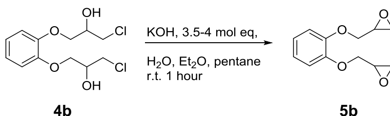
Scheme 6.13 – synthesis of hydroquinone diglycidyl ether
