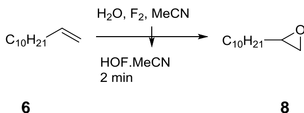
Scheme 6.15 – Epoxidation of dodec-1-ene
