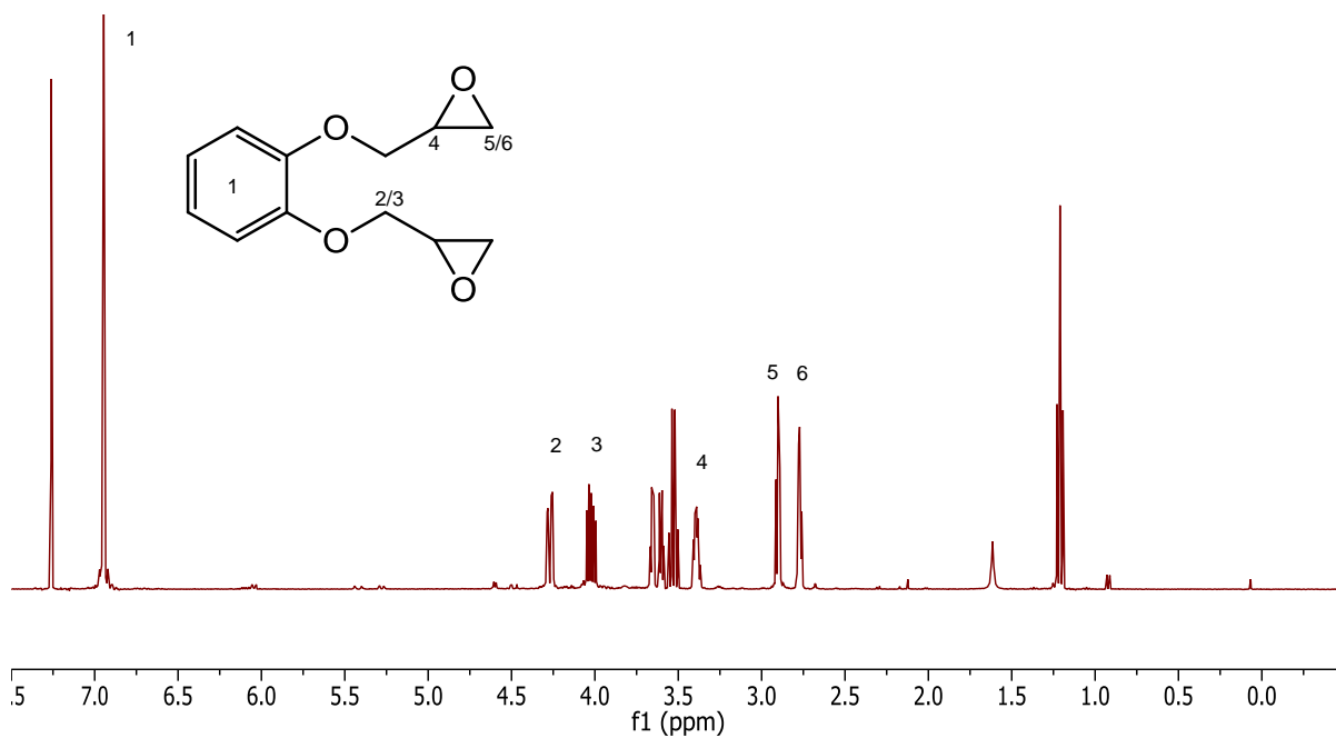
Figure 4.8 – ^1\text{H} NMR spectrum for catechol diglycidyl ether recrystallized from 2-ethoxyethyl ether and methyl isobutyl ketone (1:1)
