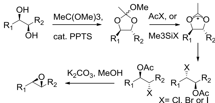
Scheme 1.2 – Synthesis of epoxides using halohydrins as developed by Kolb et al
