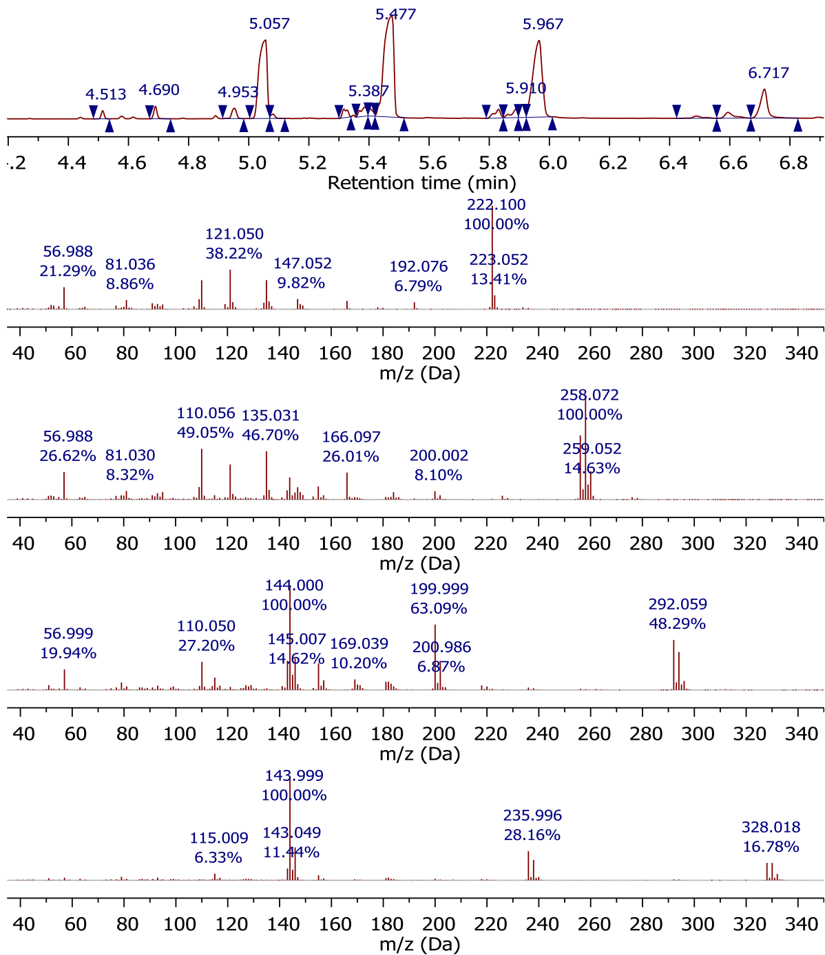
Figure 2.23 – GC-MS for catechol diglycidyl ether after 3 equivalents of potassium hydroxide.
