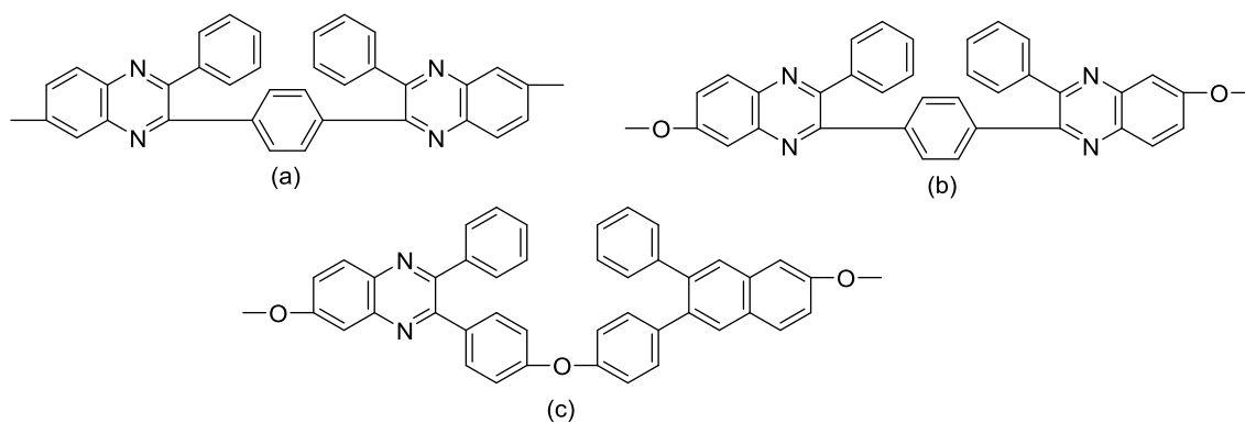
Figure 1.4 – Different linkers of phenylquinoxaline monomer unit 40 .
