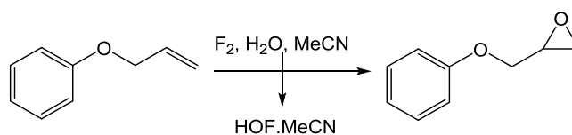
Scheme 3.2 – Conversion of phenol allyl ether to the epoxide using HOF.MeCN prepared in 'batch'.
