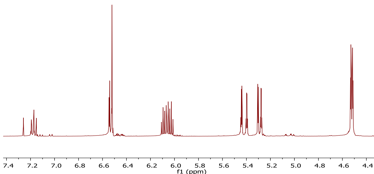
Figure 2.9 – NMR spectrum for the attempted synthesis of resorcinol diallyl ether using potassium tert -butoxide as the base.
