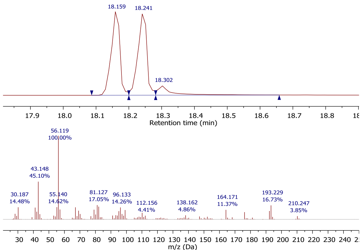
Figure 4.11 – GC-MS trace for Sigma Aldrich PACM. 18.159 = t-t, 18.241 = c-t, 18.302 = c-c
