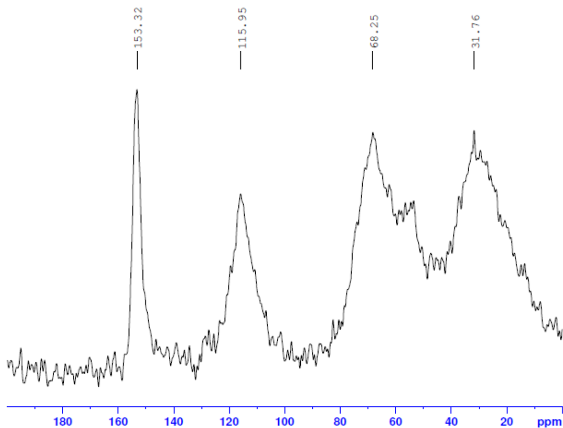
Figure 5.5 – ^{13}\text{C} NMR spectrum of the polymer network from HDGE and L-PACM
