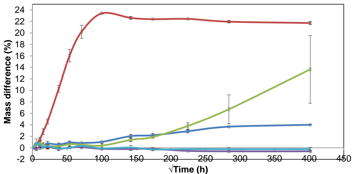
Figure 5.16 – Uptake of solvent in CDGE and L-PACM polymers. — water; — methanol; — ethanol; — propan-2-ol and — tert -butanol.
