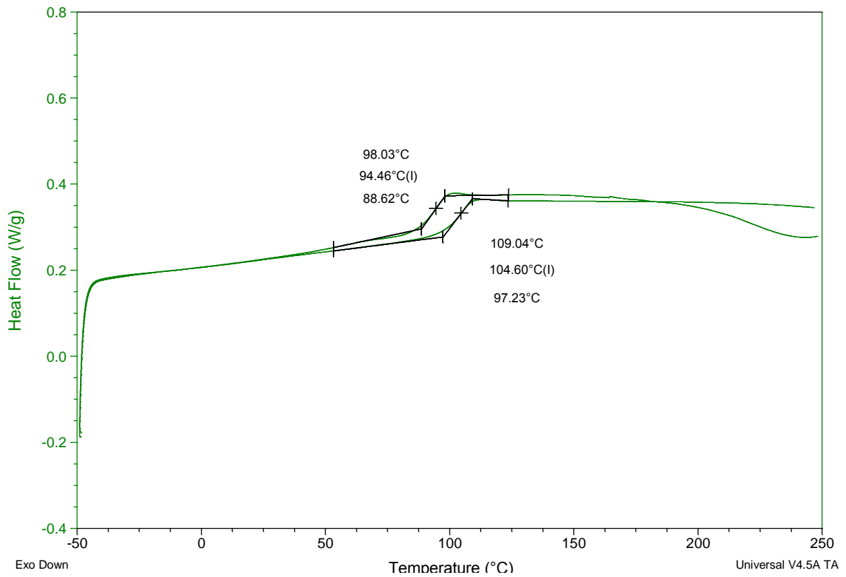
Fig 4.32 – DSC graph for CDGE with L-PACM cured at 100°C for 16 hours and post cured at 170°C using PTFE mould
