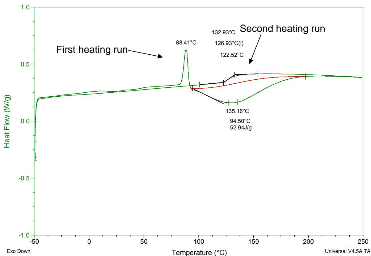
Figure 4.20 – DSC graph for after 60°C cure.
