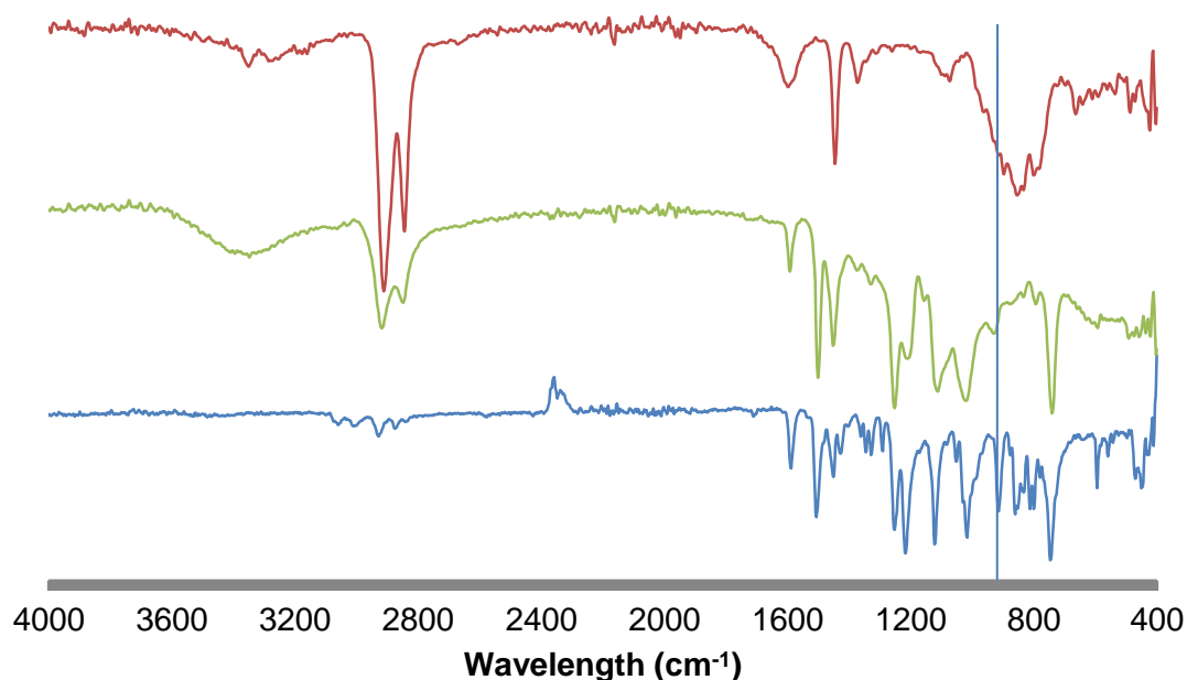
Figure 5.3 – IR spectrum for CDGE/ L-PACM polymer and monomers. – L-PACM, – polymer and – CDGE monomer.
