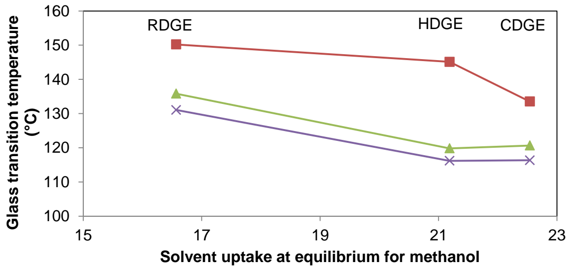
Figure 5.17 – Graphic representation of solvent uptake of methanol versus glass transition temperature. ■ is T_g from \tan \delta ; ▲ is T_g from E'' and X is T_g from E' .
