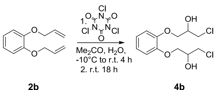
Scheme 6.10 – Synthesis of catechol dichlorohydrin ether
