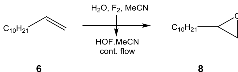
Scheme 6.19 – Epoxidation of dodec-1-ene in continuous flow
