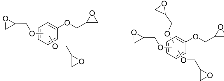
Figure 7.2 – tri and tert- functional glycidyl ethers.
