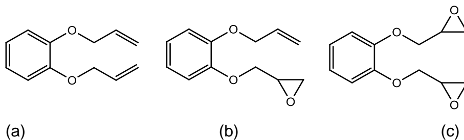
Figure 3.7 – Reaction products from the HOF.MeCN reaction of catechol diallyl ether (a) starting material, (b) mono epoxidised product and (c) desired product
