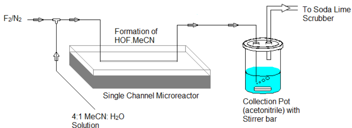
Figure 6.1 – Reaction set up for batch reactions with HOF.MeCN
