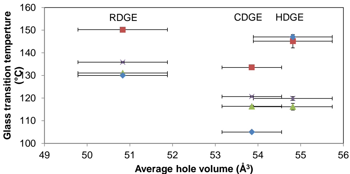
Figure 5.12 – Graphic representation of results from positron annihilation spectroscopy compared to DMTA results. ♦ T_g from DSC; ■ is T_g from Tan \delta ; ▲ is T_g from E' and X is T_g from E'' .
