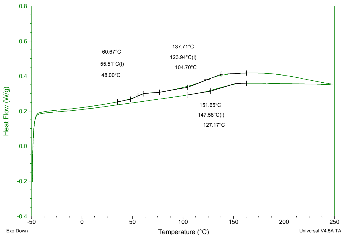
Figure 4.31 – DSC graph for HDGE with L-PACM cured at 100°C for 16 hours and post cured at 170°C using PTFE mould
