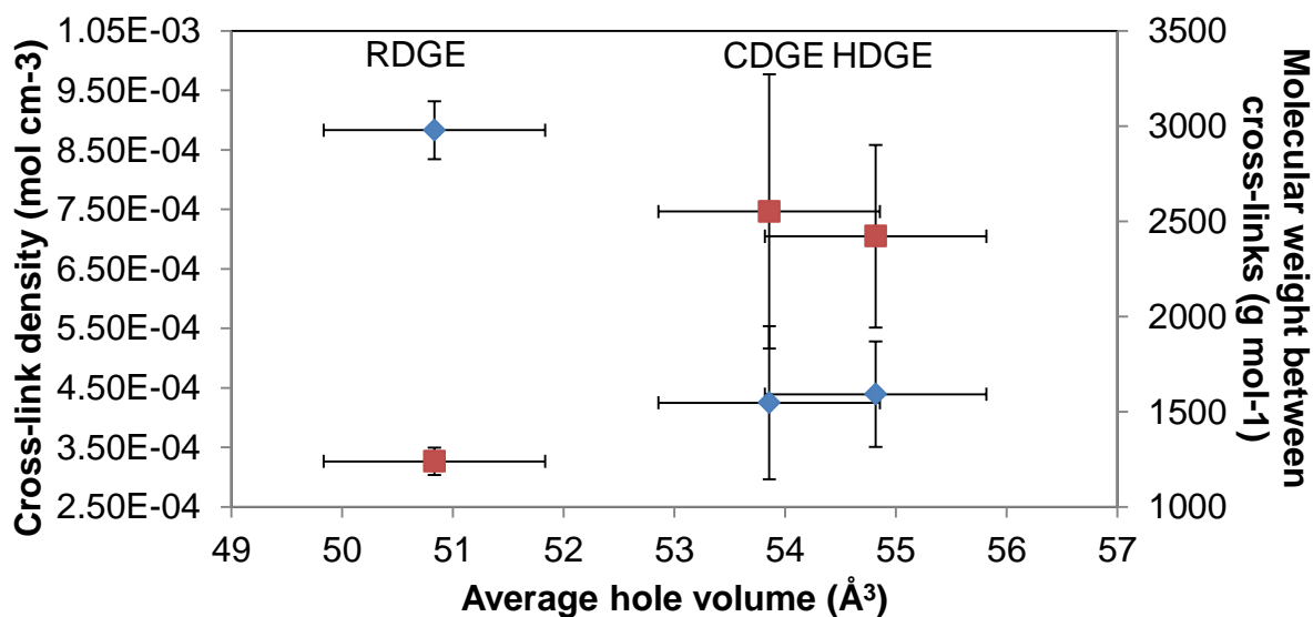
Figure 5.13 – Graphic comparison of results from positron annihilation spectroscopy and DMTA results: ♦ cross-link density; ■ molecular weight between cross-links
