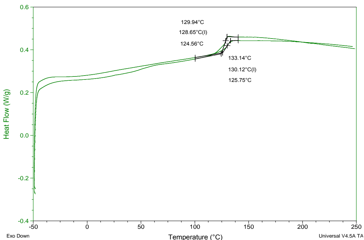
Figure 4.30 – DSC graph for RDGE with L-PACM cured at 100°C for 16 hours and post cured at 170°C using PTFE mould
