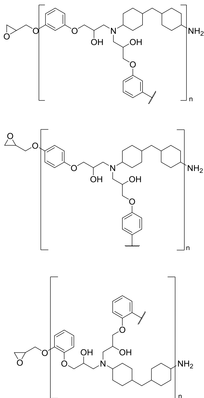
Figure 5.7 – Structure of epoxy-amine polymer formed by RDGE and L-PACM (top), HDGE and L-PACM (middle) and CDGE and L-PACM (bottom).
