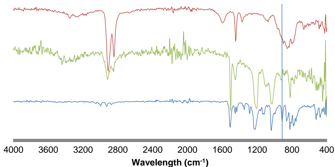
Figure 5.2 – IR spectrum for HDGE/ L-PACM polymer and monomers. – L-PACM, – polymer and – HDGE monomer.
