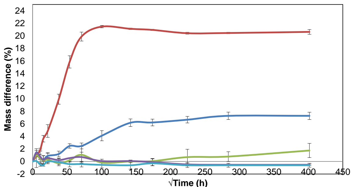
Figure 5.15 – Uptake of solvent in HDGE and L-PACM polymers. — water; — methanol; — ethanol; — propan-2-ol and — tert -butanol.
