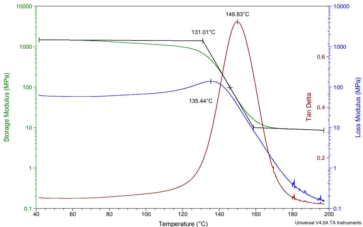
Figure 5.8 – DMTA plot for RDGE and L-PACM polymer films (sequence 2).
