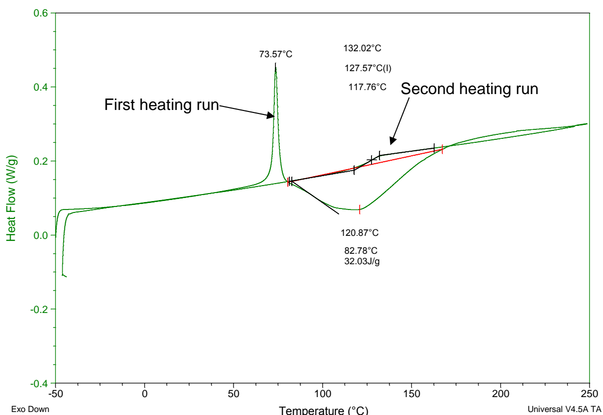
Figure 4.18 – DSC graph for a kinetic study of RDGE with Sigma Aldrich PACM
