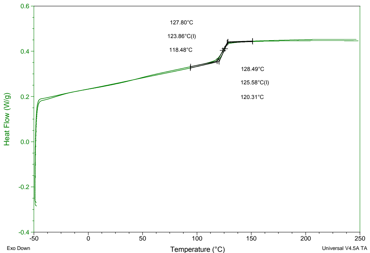
Figure 4.21 – DSC graph for after 140°C post cure.
