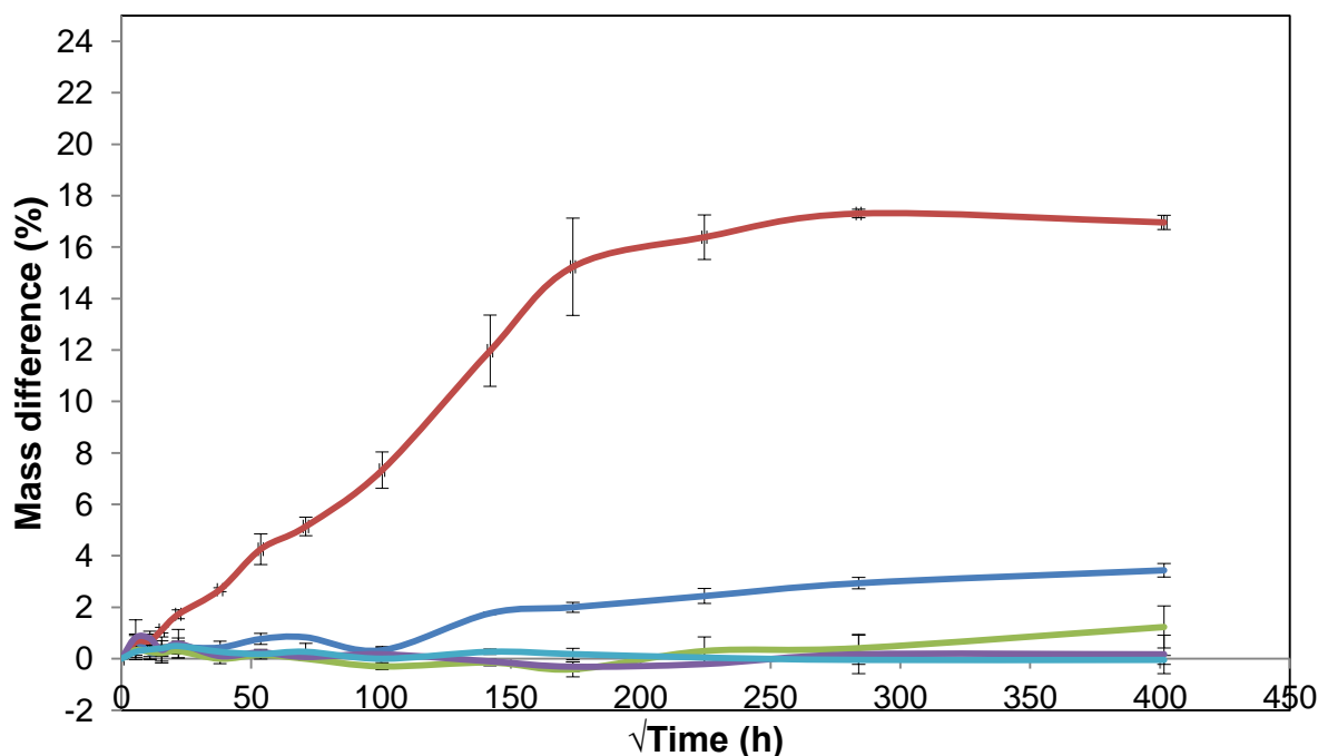
Figure 5.14 – Uptake of solvent in RDGE and L-PACM polymers. – water; – methanol; – ethanol; – propan-2-ol and – tert -butanol.
