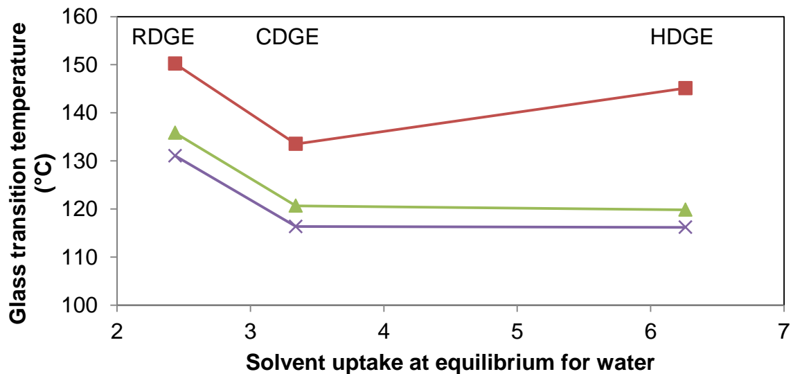
Figure 5.18 – Graphic representation of solvent uptake of water versus glass transition temperature. ■ is T_g from \tan \delta ; ▲ is T_g from E'' and X is T_g from E' .
