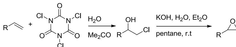
Scheme 2.7 – Synthesis of epoxides using trichloroisocyanuric acid
