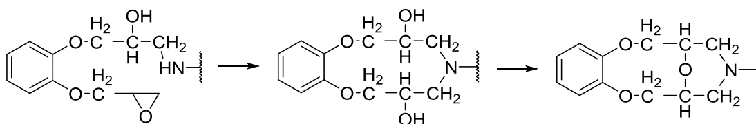
Scheme 5.1 – Formation of cyclized ether with ring opening of neighbouring epoxides by the same amine.
