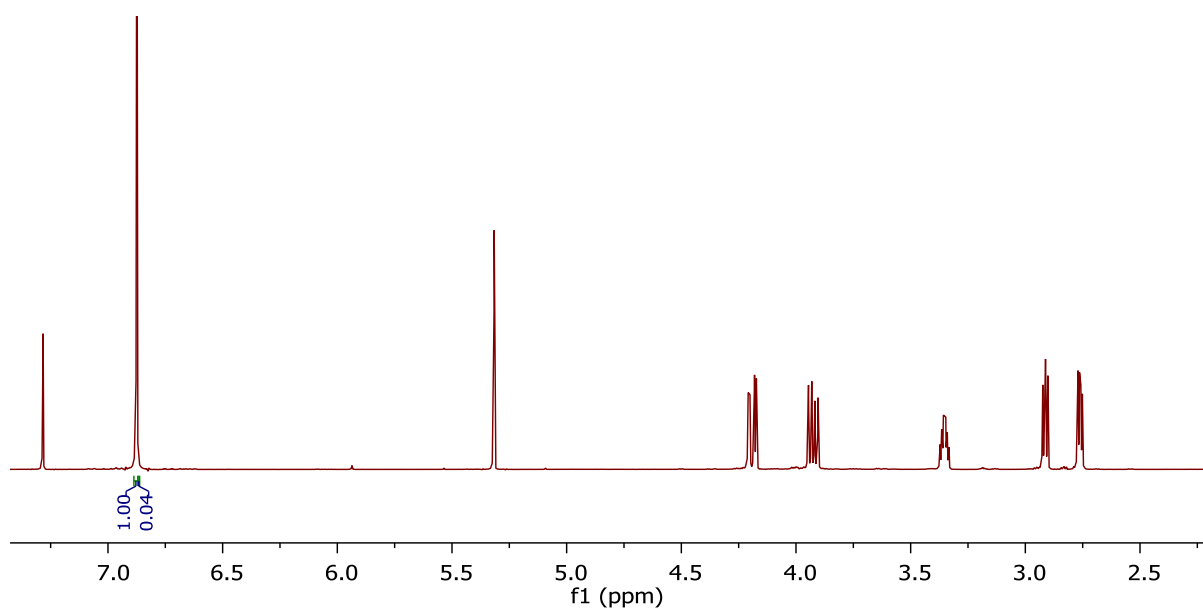
Figure 3.12 – ^1\text{H} NMR analysis of the organic layer after collection with \text{D}_2\text{O} and \text{NaOD} .
