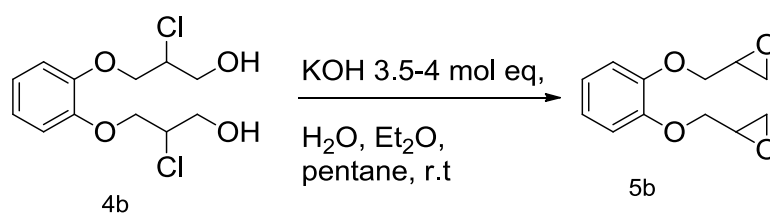
Scheme 2.13 – Ring closing of catechol dichlorohydrin ether to create catechol diglycidyl ether.
