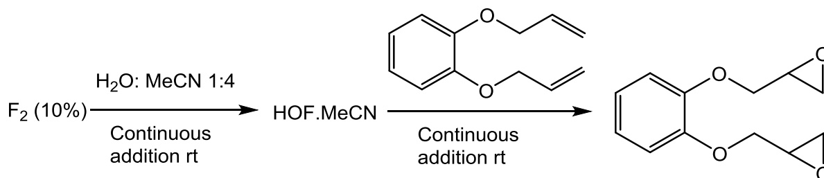
Scheme 3.7 – Continuous flow epoxidation of catechol diglycidyl ether
