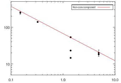
RXJ0740.9+5526
