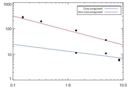
RXJ1320.1+3308
