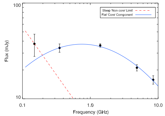
RXJ1315.4-1623
