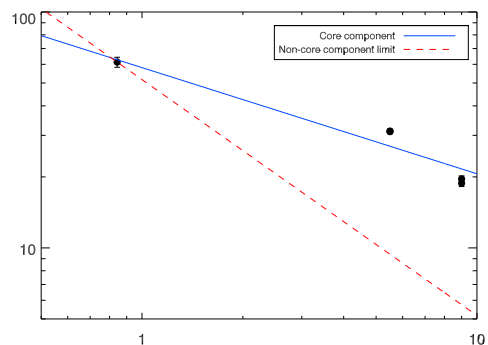
RXJ1539.5-8335
