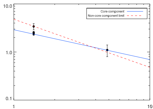
RXJ1440.6+0327
