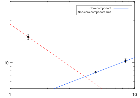
RXJ0352.9+1941
