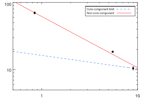
RXJ1947.2-7623
