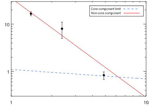
RXJ0419.6+0225
