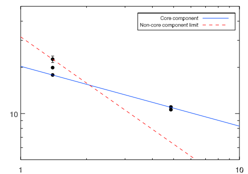
RXJ1442.2+2218
