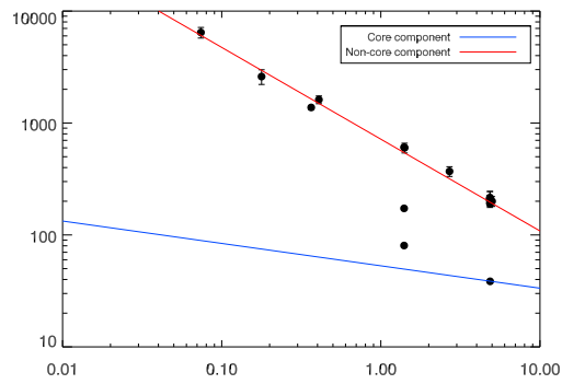
RXJ1604.9+2356
