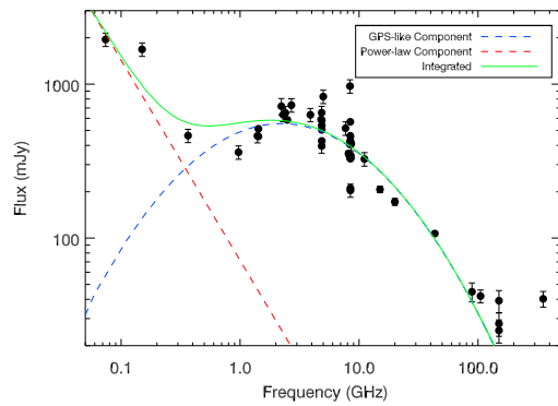
RXJ1558.4-1410
