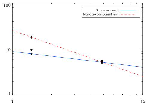
RXJ1733.0+4345
