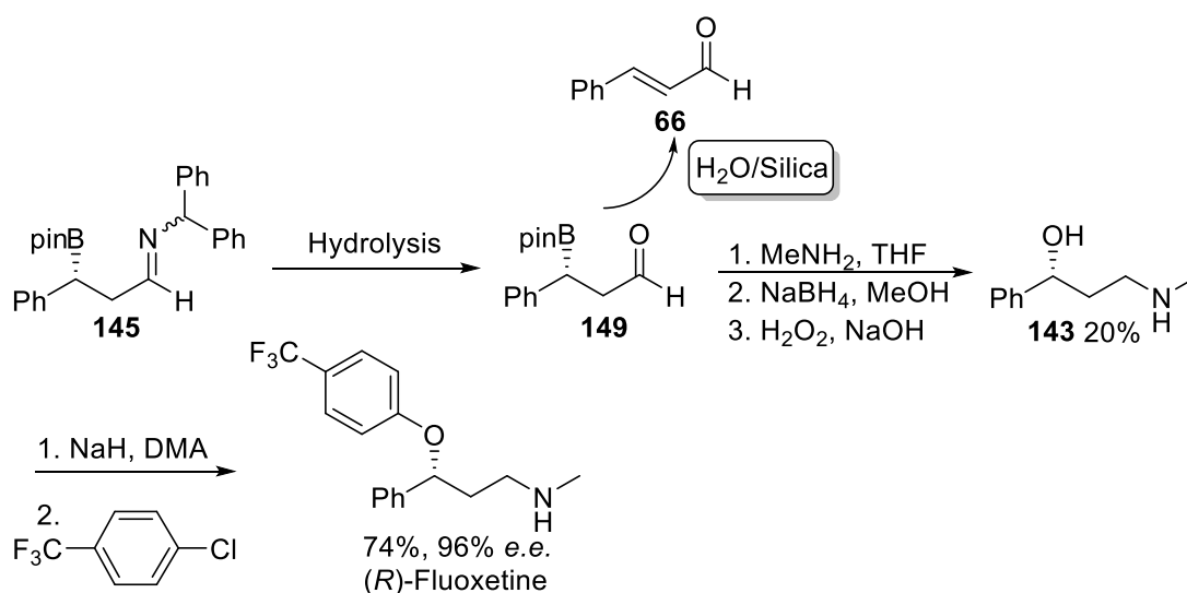
Scheme 42 Hydrolysis and reductive amination approach to Fluoxetine.
