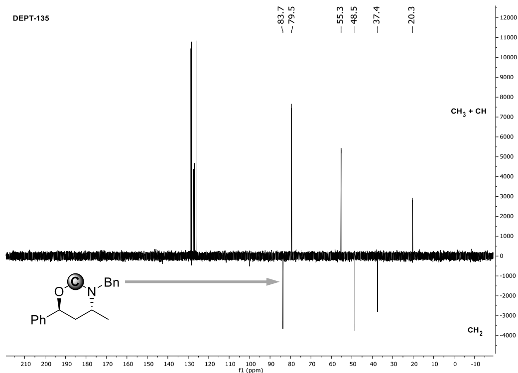
Figure 9 13 C NMR DEPT-135 Analysis on compound 65 : CH 2 appear negative; CH 3 and CH appear positive (quaternary carbons are not visible).
