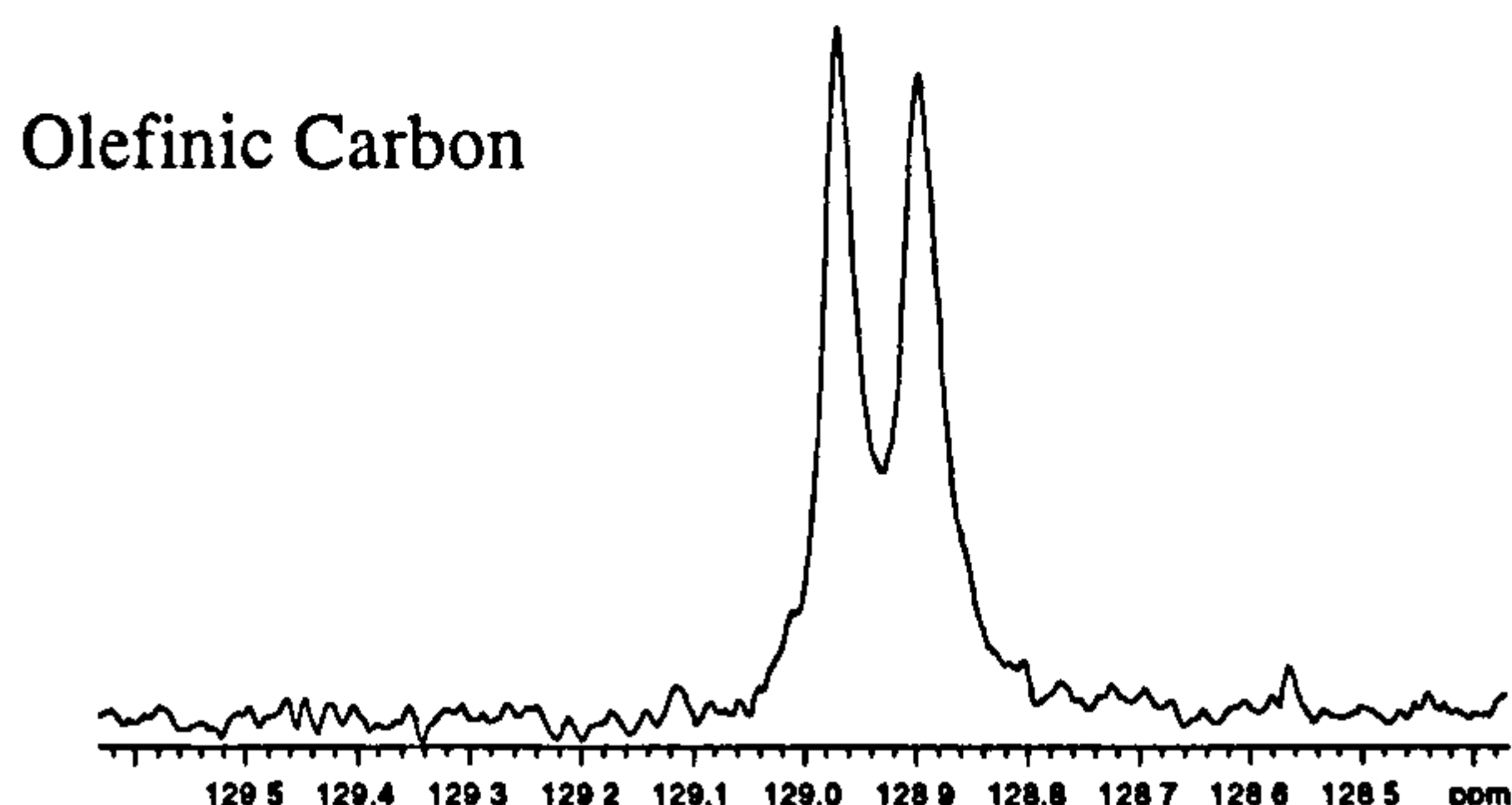
Figure 5-5 Olefinic carbon peaks in the ^{13}\text{C} NMR spectrum of the polymer of 1-cyano-1- tert -butoxycarbonyl-2-vinylcyclopropane
