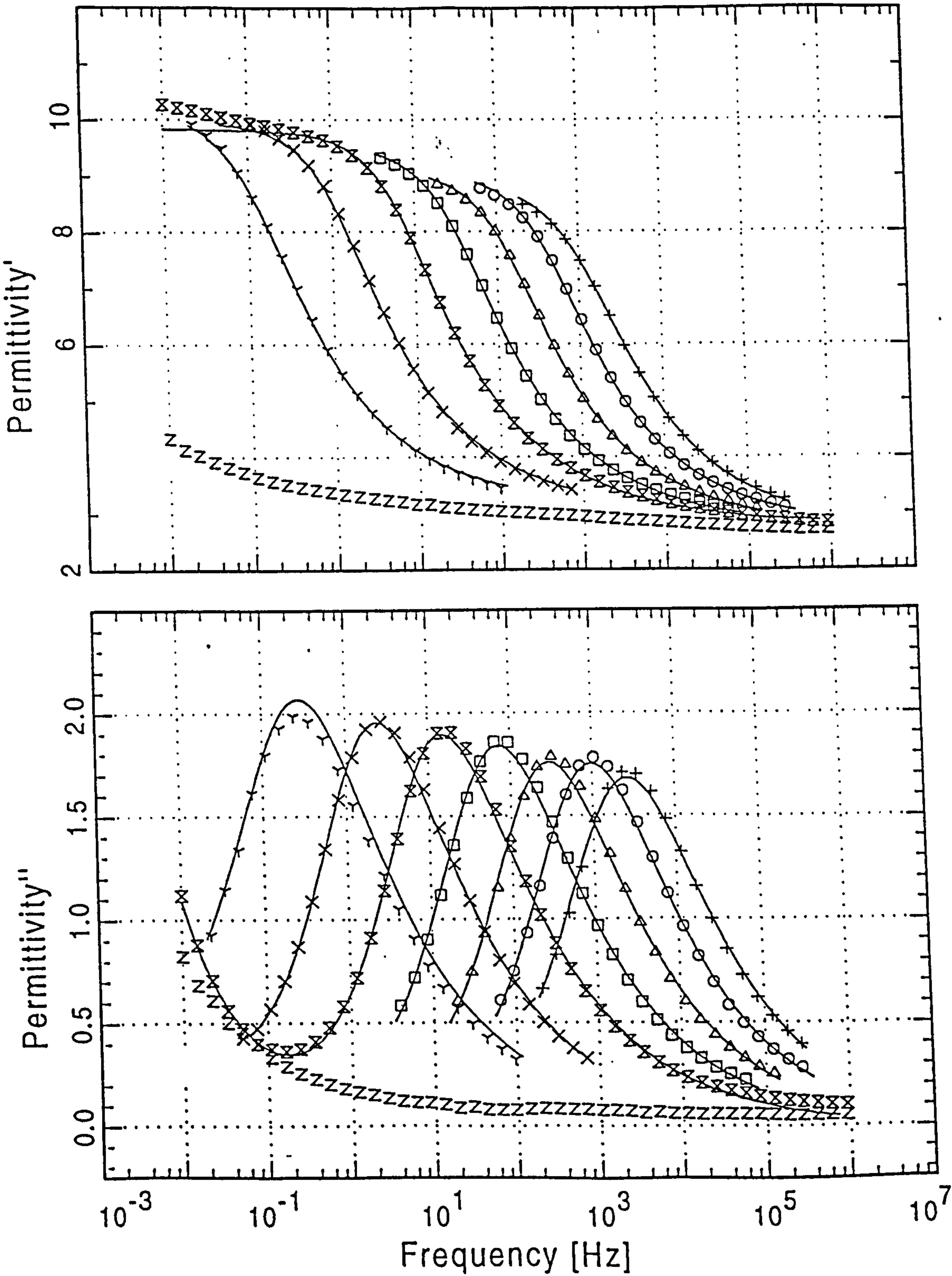
Appendix 6.2 Graphs of real and imaginary permittivity against frequency for the butyl ester homopolymer
