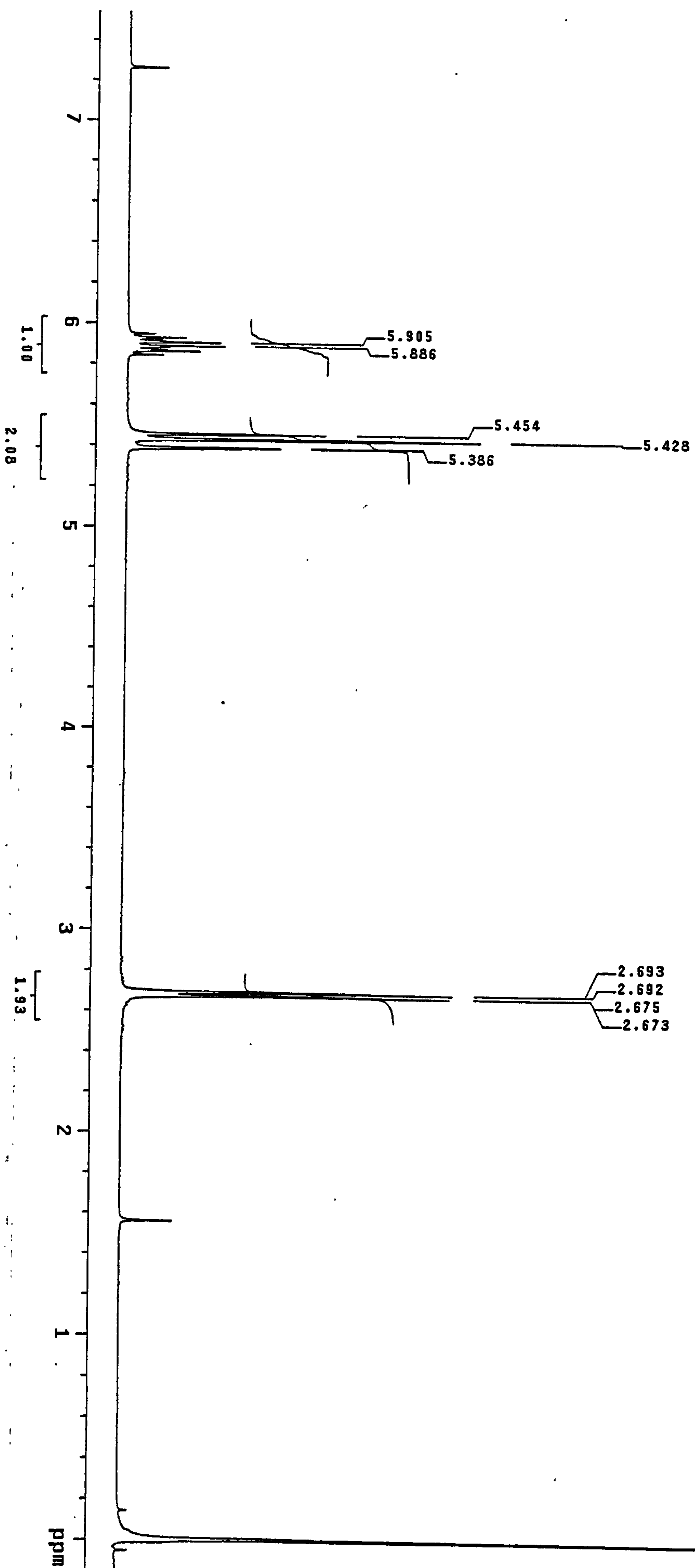
Appendix 1.10 ^1\text{H} NMR spectrum of diallyl malononitrile
