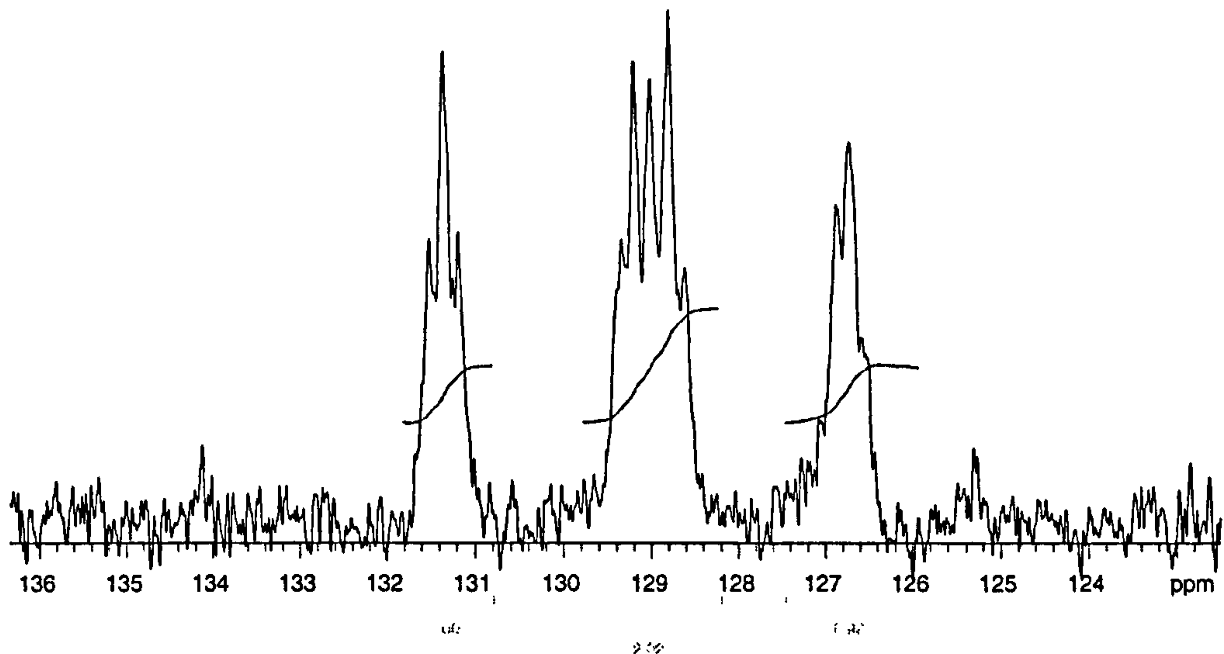
Figure 6-2 Olefinic carbon peaks in the ^{13}\text{C} NMR spectrum of copolymer B showing the 1:2:1 splitting pattern
