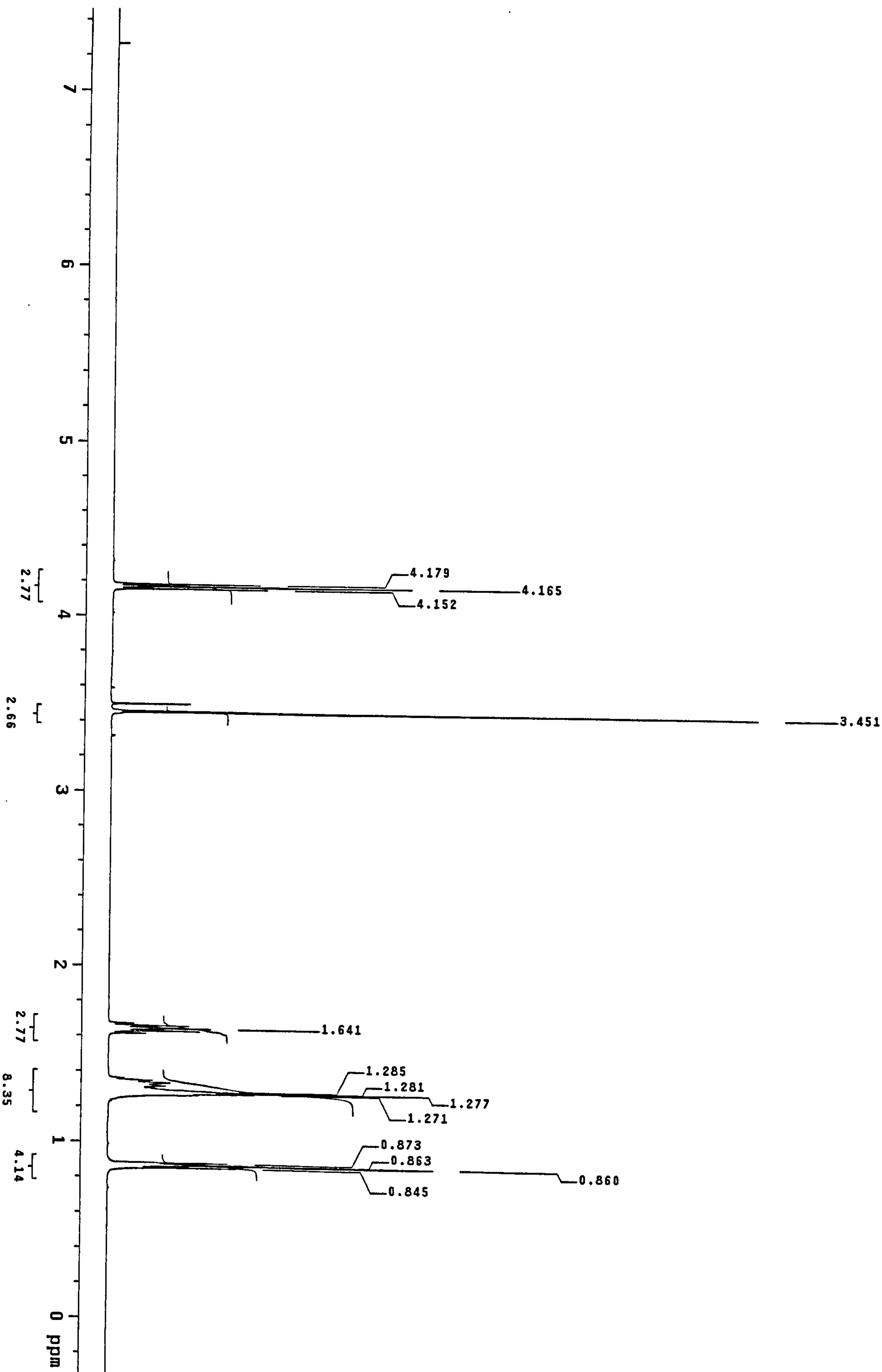
Appendix 4.10 ^1\text{H} NMR spectrum of hexyl-cyanoacetate
