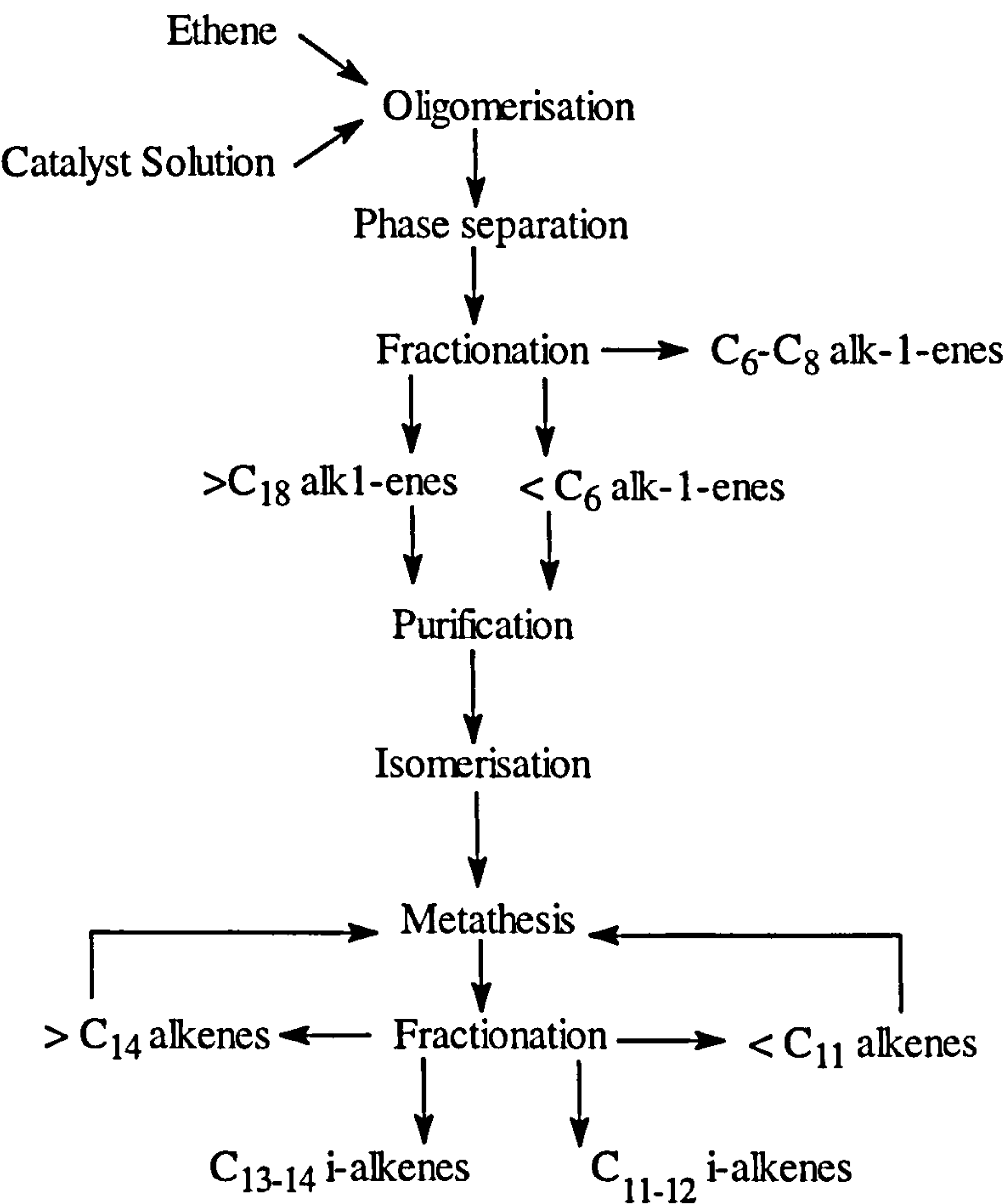
Figure 2-1 Schematic for the SHOP process
