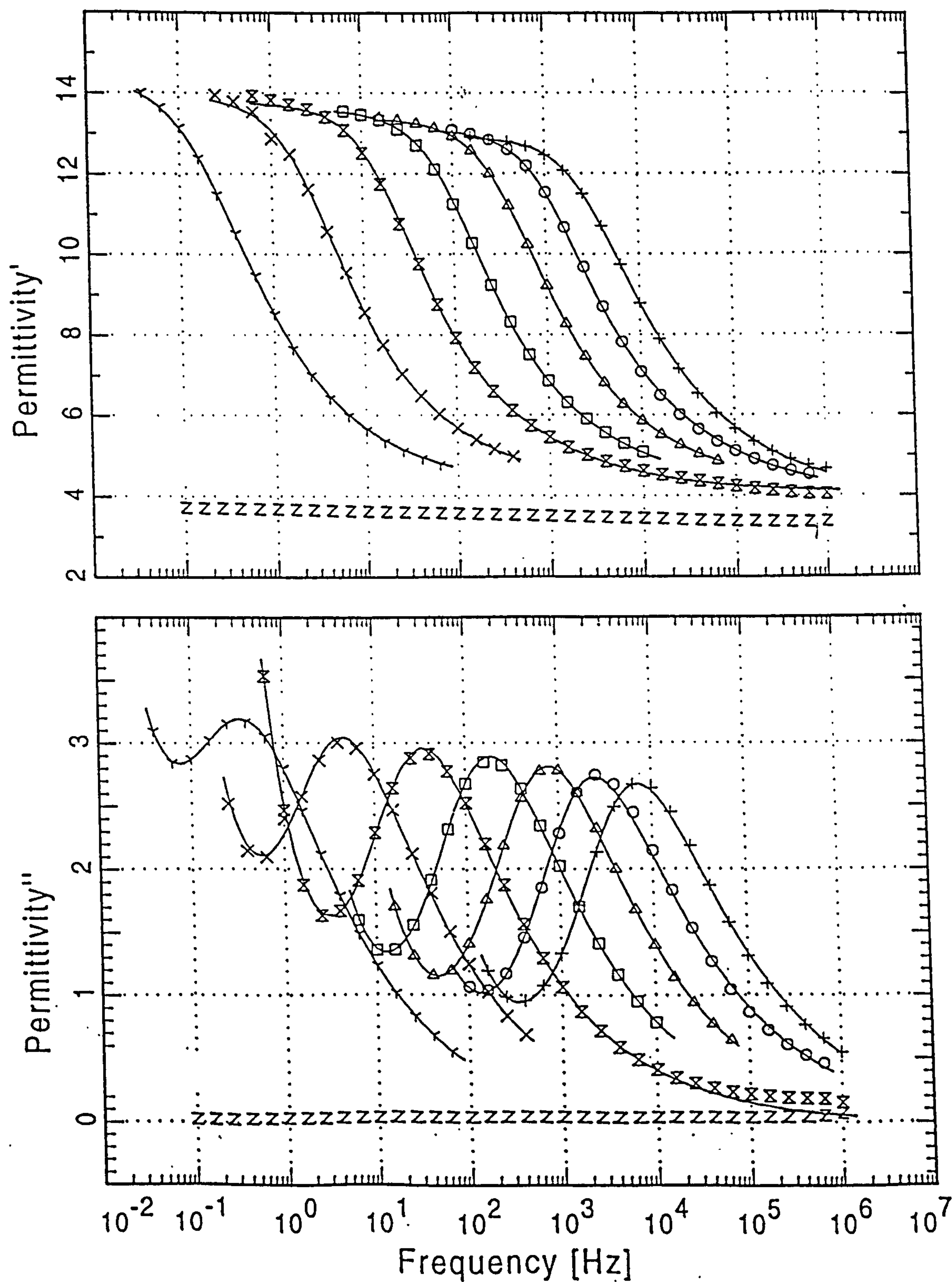
Appendix 6.1 Graphs of real and imaginary permittivity against frequency for the tert -butyl ester homopolymer
