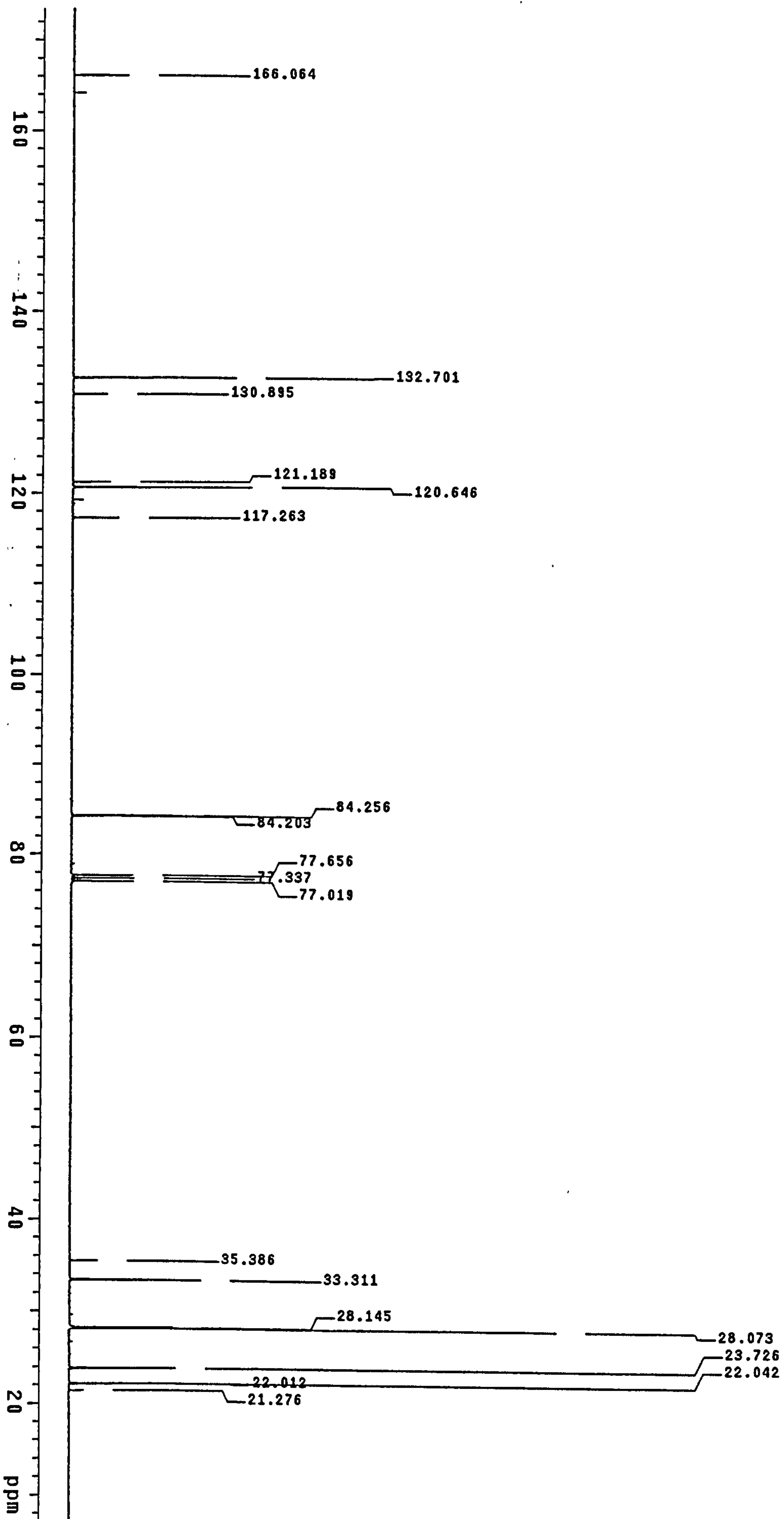
Appendix 4.3 ^{13}\text{C} NMR spectrum of 1-cyano-1- tert -butoxycarbonyl-2-vinylcyclopropane
