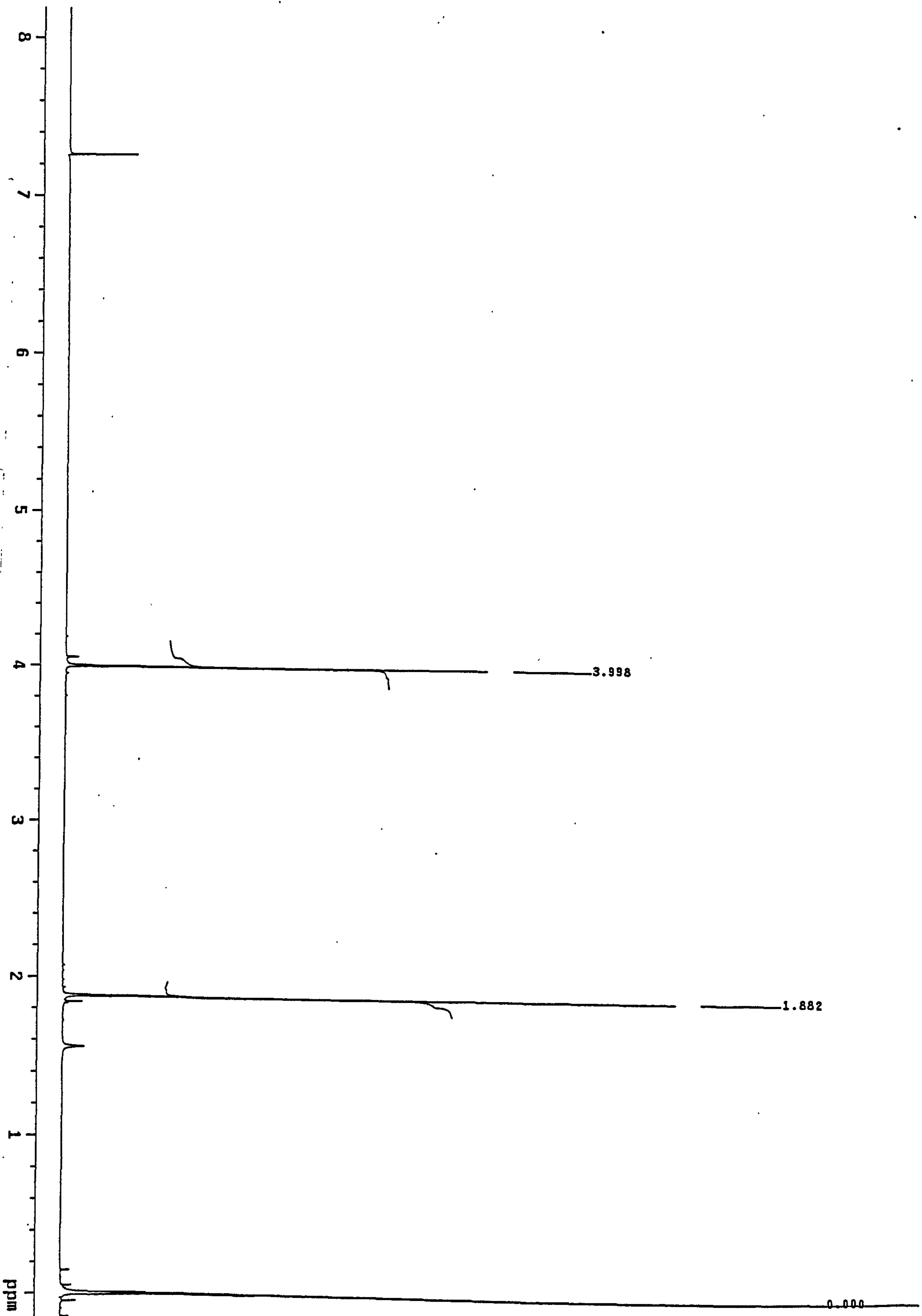
Appendix 2.5 1 H NMR spectrum of trans -1,4-dibromo-2,3-dimethyl-2-butene
