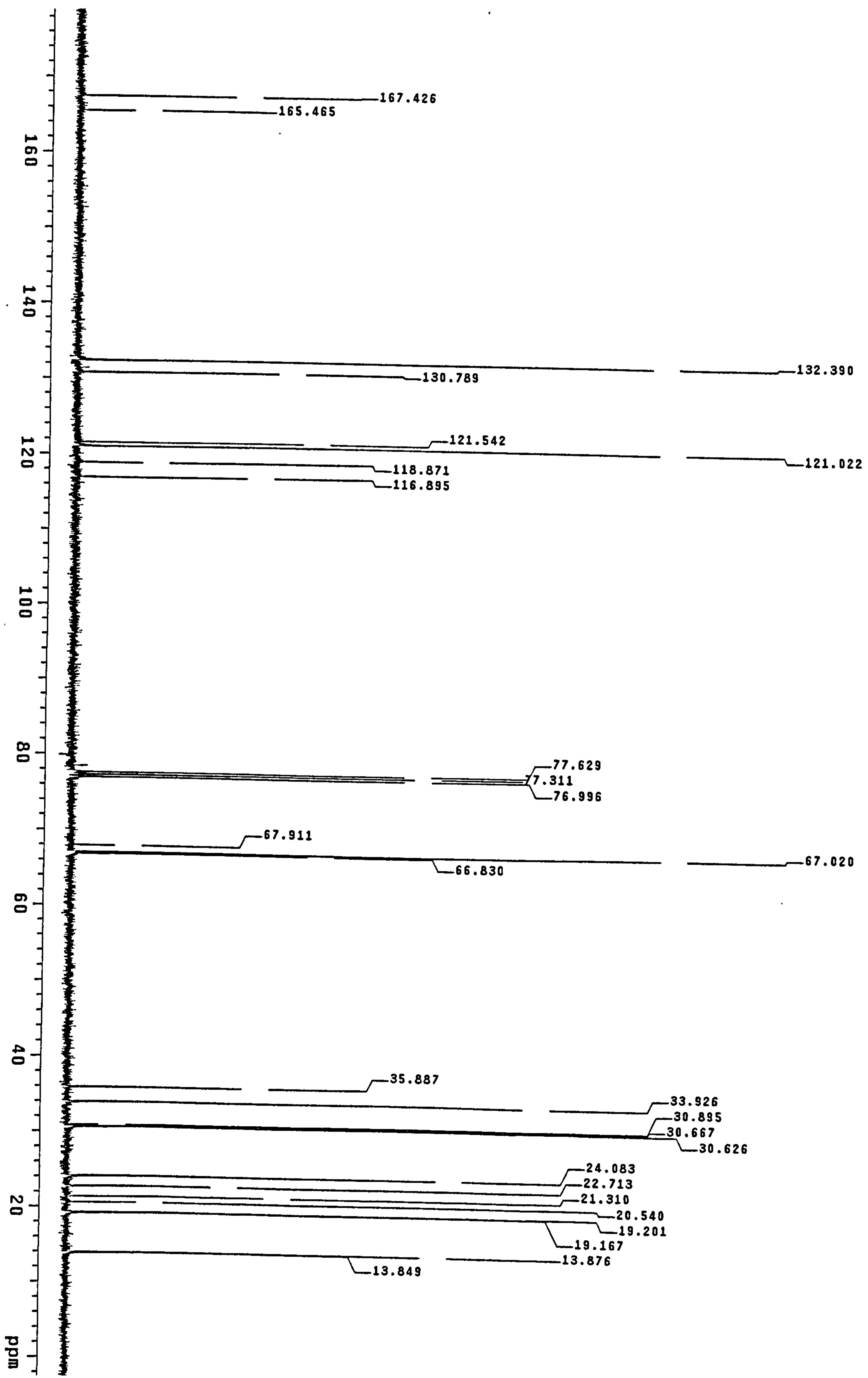
Appendix 4.7 ^{13}\text{C} NMR spectrum of 1-cyano-1-n-butoxycarbonyl-2-vinylcyclopropane
