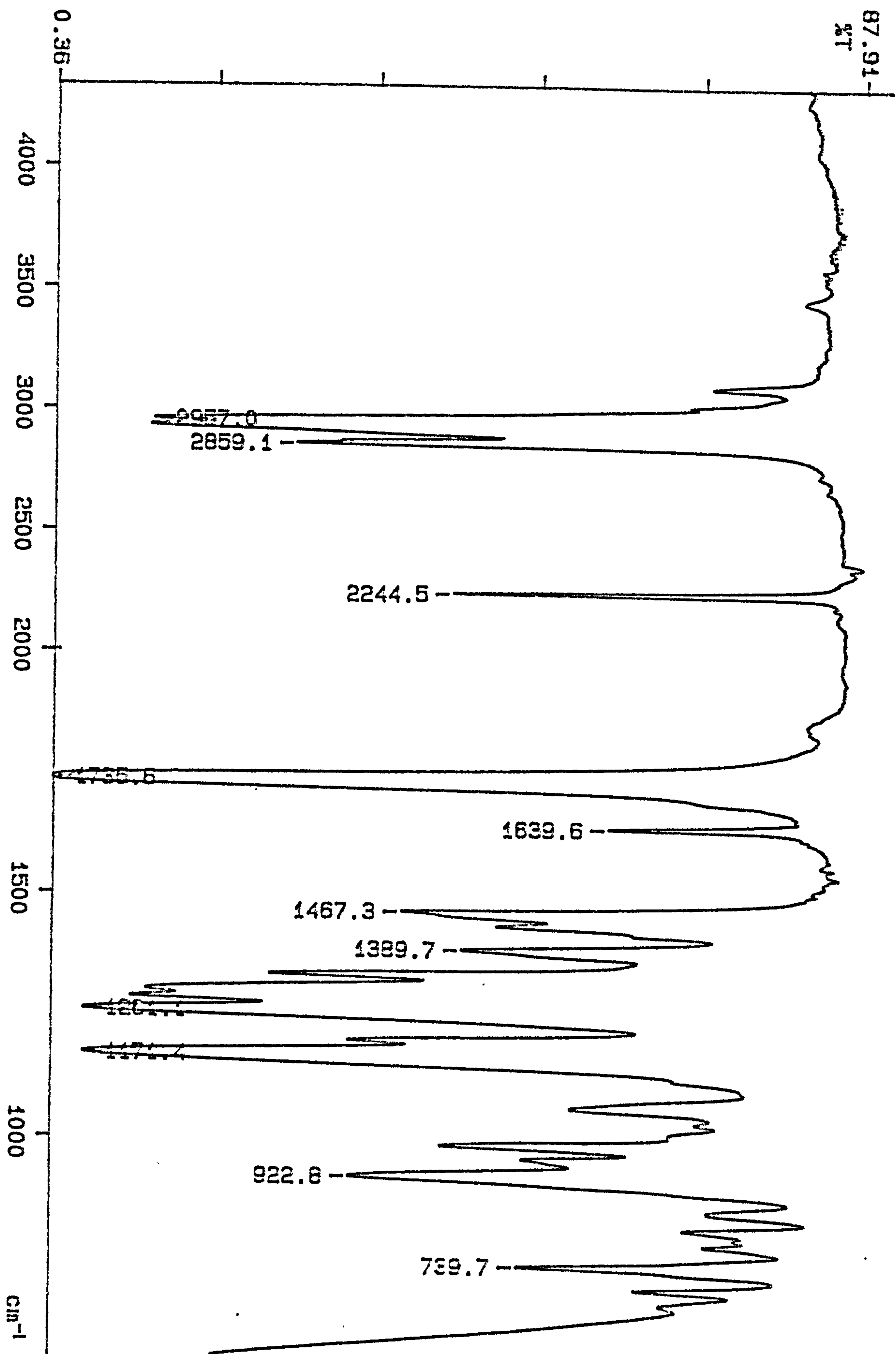
Appendix 4.5 Infra-red spectrum of 1-cyano-1-n-butoxycarbonyl-2-vinylcyclopropane
