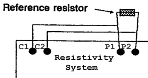
Figure 4.3. Measurement setup using a high precision reference resistor (ABEM, Terrameter SAS 300 C, instruction manual)
