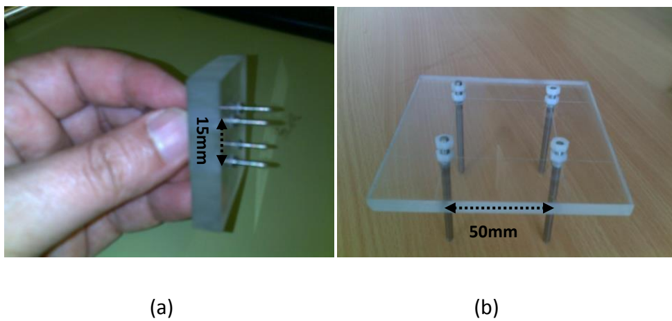
Figure 3.14. Square resistivity devices constructed in this study
