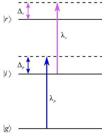
Figure 1.4: Two-photon, three-ladder Rydberg excitation scheme. Atoms in the ground state |g\rangle are excited to the intermediate state |i\rangle via a single-photon from the probe laser at \lambda_p . The atoms in state |i\rangle are excited to the Rydberg state |r\rangle via a single-photon at \lambda_c from the coupling laser. The probe ( \Delta_p ) and coupling ( \Delta_c ) laser detunings are also shown.
