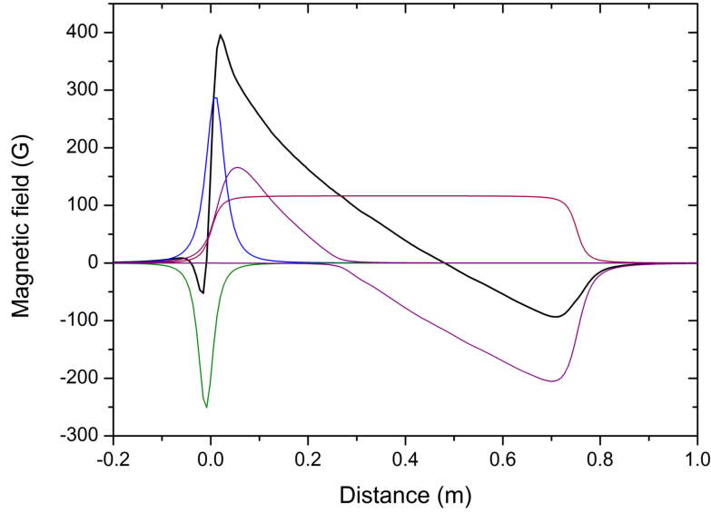
Figure 5.6: The individual contributions from each coil to the total magnetic field profile (black) for Yb. The solenoid is shown in red, coils 1 and 2 in purple, coil 3 in blue and coil 4 in green. The location of the MOT is -0.075 m on this scale.
