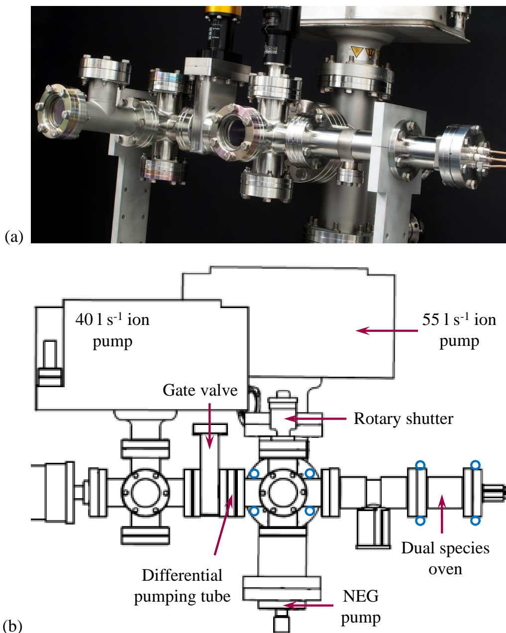
Figure 3.8: (a) A photograph taken of the oven and spectroscopy sections before their first bake. At this time the 40\text{ l s}^{-1} ion pump was still on an old vacuum system and wasn't added until the final bake out of the entire vacuum system, however the tee for it to be attached to can be seen towards the left of the photograph. (b) A schematic of the oven and spectroscopy sections, with key components such as the gate valve, differential pumping tube and pumps labelled. The locations of the water cooled clamps are shown as pairs of blue circles.
