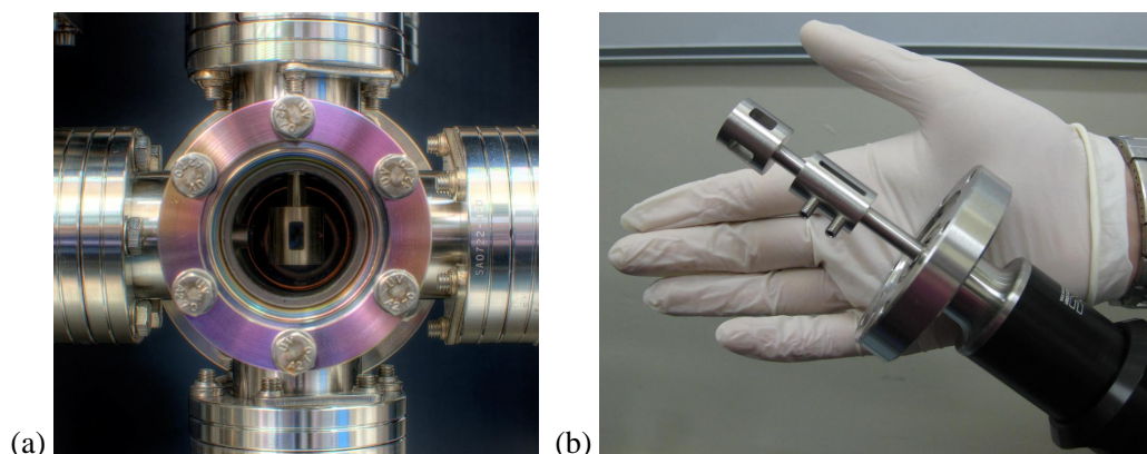
Figure 3.9: (a) The rotary shutter is centred on the atomic beam position and allows the atomic beam to be blocked when not in use. The differential pumping tube can be seen in the left of the viewport. (b) Two of the apertures in the shutter can be seen along with the grub screws holding the shutter on to the motorised feedthrough. The two long slots allow trapped gas from the threads of the grub screws to escape.
