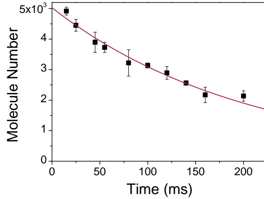
Figure 8.7: Lifetime of ^{87}\text{RbCs} molecules in the | -2(1,3)d(0,3) \rangle state at 181 G held in the optical dipole trap. A magnetic field gradient of 44 G/cm is applied to levitate the molecules and the power in each beam of the dipole trap is 100 mW. Under these conditions, there is no trapping potential for the atoms. The solid line shows an exponential fit to the results, which yields a lifetime of 0.21(1) s.
