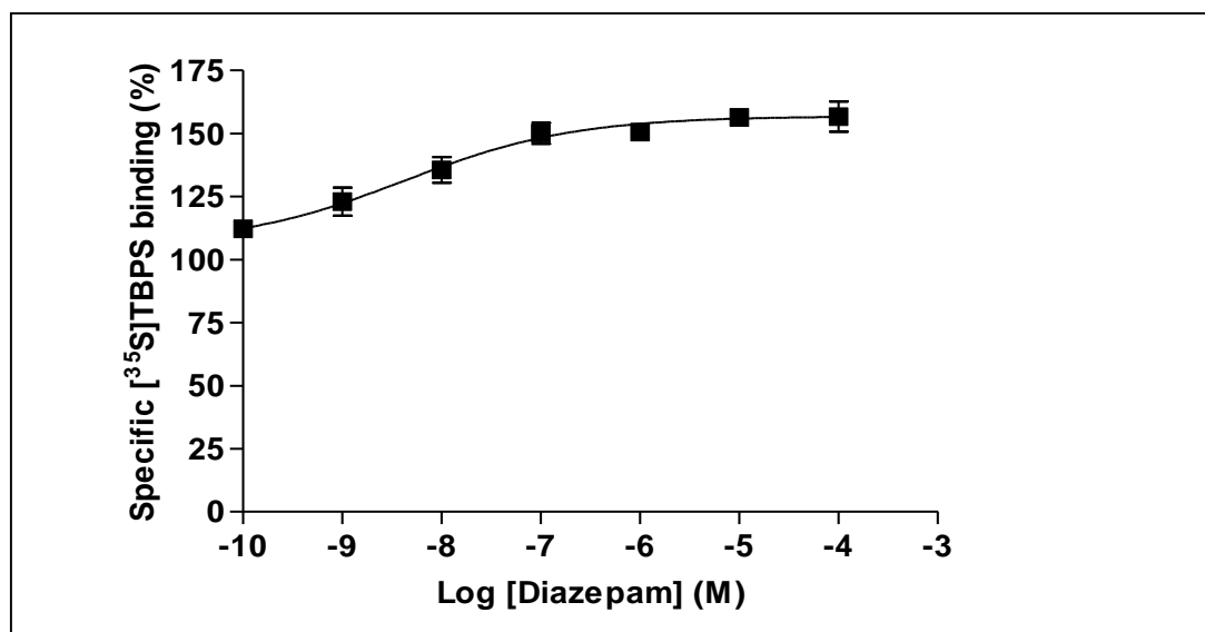
Fig 2.12 [ 35 S] TBPS competition binding to well-washed adult rat forebrain membranes in the presence of diazepam. Results are mean \pm SD for three independent experiments each performed in triplicate.
