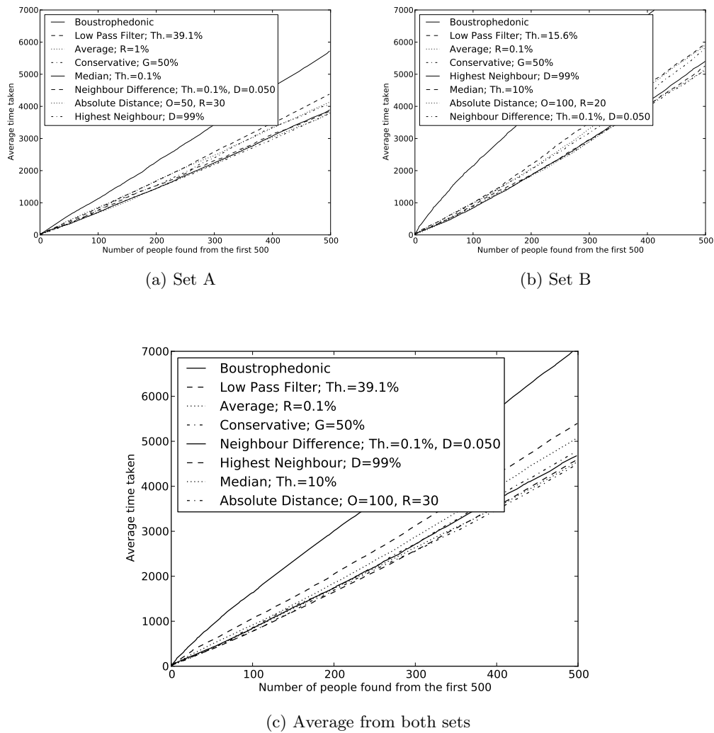
Figure 3.14: The time taken to find 500 people, the probability of whose discovery is based on both the likelihood of their existence and on the likelihood of their being found if this is the case. The data is averaged over 10 base maps in each of two map sets, both individually and collectively.
