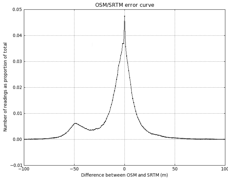
Figure 6.3: OSM / SRTM error curve, showing the proportionate number of readings for each error value. Graph cropped to errors between \pm 100 m. 0.34% of readings lie below and 0.70% of readings lie above this range.
