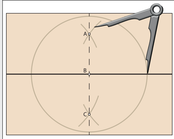
Figure 1.8: The likely method used to subdivide an arc of a circle perfectly in half, using dividers.
