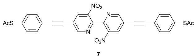
Fig. 1.13 Molecular structure of bipyridyl-dinitro oligo(phenyleneethynylene) dithiol (BPDN-DT) investigated in Lörtscher's work. (Reproduced from reference 37 )
