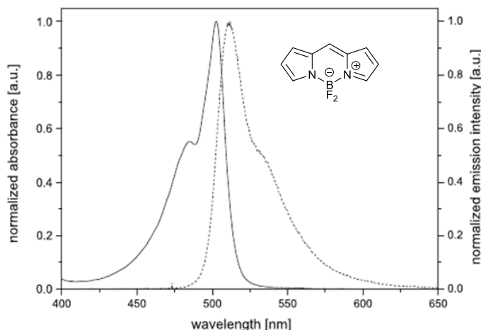
Figure 6.5 : Absorption (solid line) and fluorescence emission (dashed line) spectra of “naked” BODIPY in DCM (adapted from Schmitt et al. 6 )
