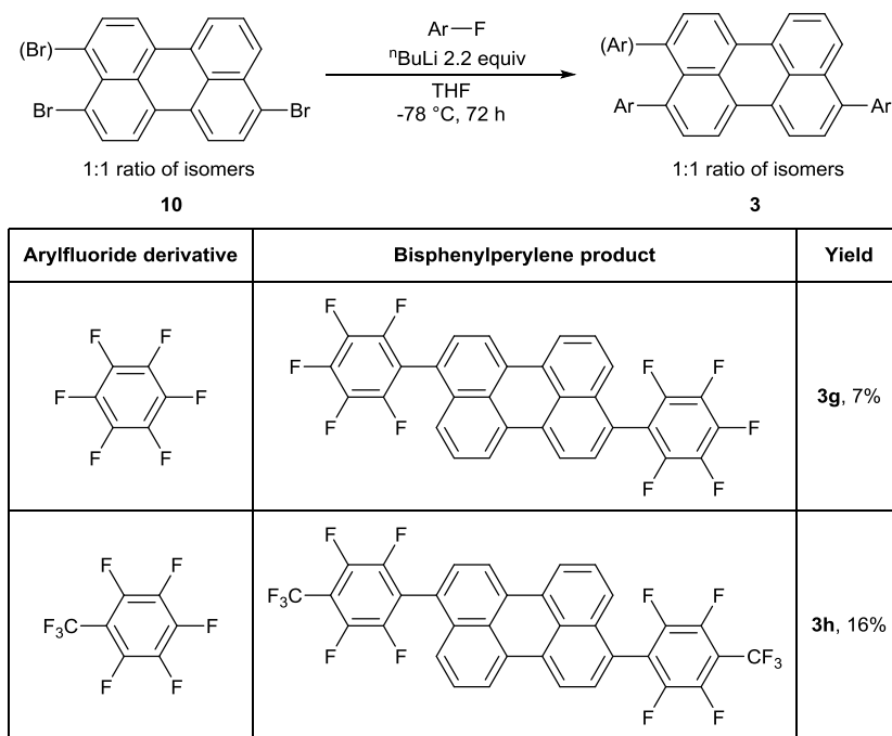
Figure 4.7 : S_NAr synthesis of highly fluorinated bis -phenylperylenes
