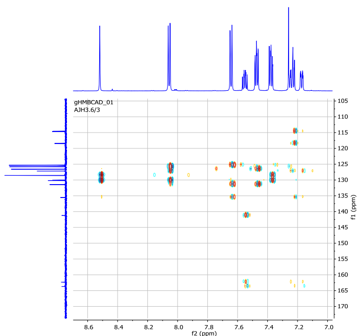
Figure 2.35 : HMBC spectrum of 1c
