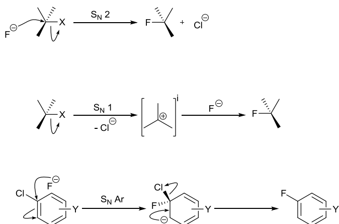
Figure 1.23 : HALEX reactions
