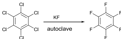
Figure 1.24 : Perfluorobenzene synthesis
