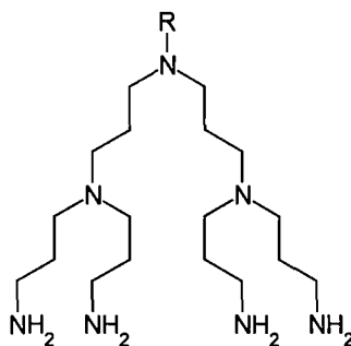
Figure 1.2: The Vögtle Cascade Structure.
