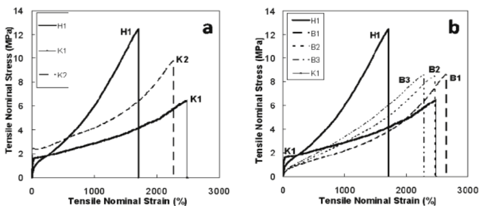
Figure 1.11 Tensile stress-strain behavior for HyperBlock ( H1 ), Kraton polymers ( K1 , K2 ), blends of H1 and K1 containing 10% H1 ( B1 ), 20% H1 ( B2 ) and 30% H1 ( B3 ). [25] "Reprinted (adapted) with permission from (Hutchings L. R., Dodds J. M., Rees D., Kimani S. M., Wu J. J., Smith E. Macromolecules 2009 , 42 , 8675-8687). Copyright (2009) American Chemical Society."
