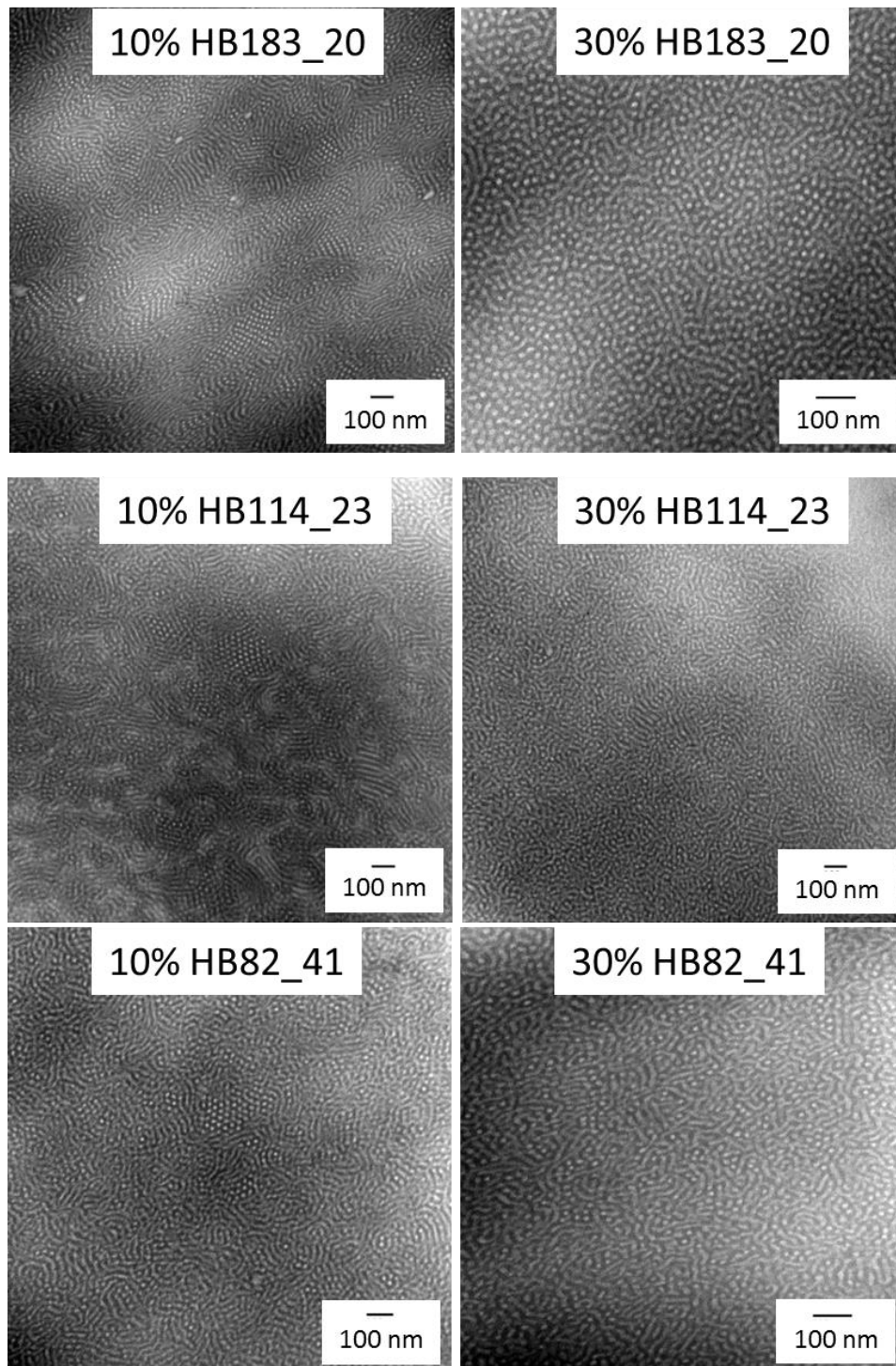
Figure 3.11 TEM micrographs of the binary blends HyperBlock/Kraton™ D-1160. The two types of blends have a content of HyperBlock of 10 and 30 wt. % whose TEM images are reported respectively on the left and right column of the picture. In this figure we compare blends of HyperBlocks with a content of polystyrene of 20 and 40 wt. %.
