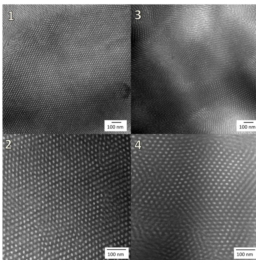
Figure 3.5 TEM micrographs for the sample Kraton™ D-1124P three-arm star (30% PS). 1 and 2 are images for the unannealed film, 3 and 4 are the images for the films annealed at 120°C.
