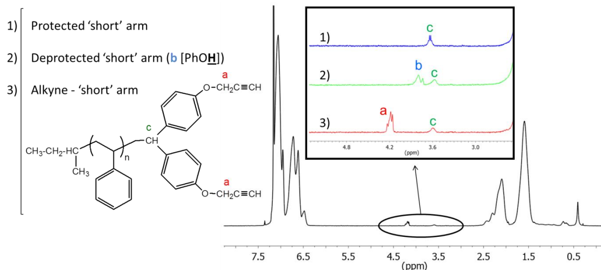
Figure 4.8 ^1\text{H-NMR} spectra of the 'short' arm provided with two alkyne functionalities in \text{C}_6\text{D}_6 (400 MHz). Comparison of the spectra acquired during the transformation of the chain-end functionalities from protected phenol groups to alkyne groups.
