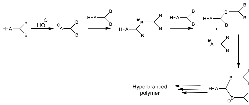
Scheme 1.13 Hyperbranched polymer synthesis by proton-transfer polymerisation.
