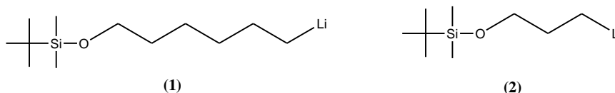
Figure 1.7 Protected initiators 6-( t -butyldimethylsiloxy)hexyllithium (1) and 3-( t -butyldimethylsiloxy)propyllithium (2).
