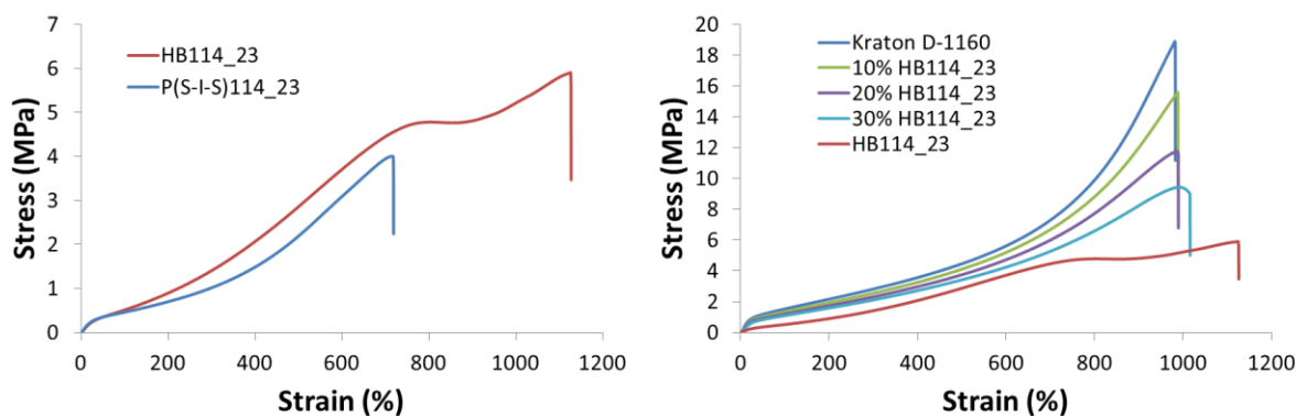
Figure 3.22 Representative tensile stress-strain curves for P(S-I-S)114_23 and HyperBlocks, compared in the graph on the left, and stress-strain curves for Kraton™ D-1160 and blends compared with HB114_23 in the graph on the right.
