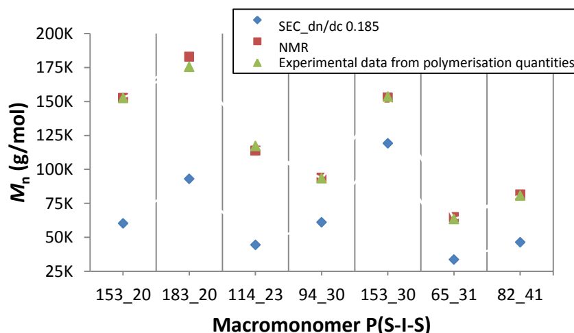
Figure 2.8 Comparison between M_n calculated in three different ways: by SEC with a \text{dn}/\text{dc} of 0.185 of polystyrene (blue line), by ^1\text{H-NMR} spectroscopy (red line) and by considering the amount of monomers added during the polymerisation and the molecular weight obtained by SEC of the first polystyrene block (green line).
