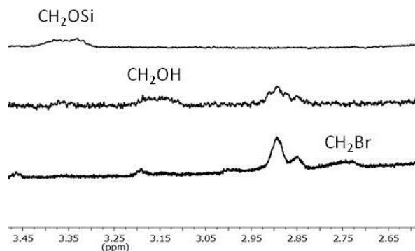
Figure 2.10 Overlay of ^1\text{H-NMR} spectra in \text{C}_6\text{D}_6 (700 MHz and 400 MHz) of protected, deprotected and brominated P(S-I-S)82_41. Shift of the peak of the end group functionality during the transformation from protected alcohol [ \text{CH}_2\text{OSi} ] to primary alcohol [ \text{CH}_2\text{OH} ] and finally to alkyl bromide [ \text{CH}_2\text{Br} ].
