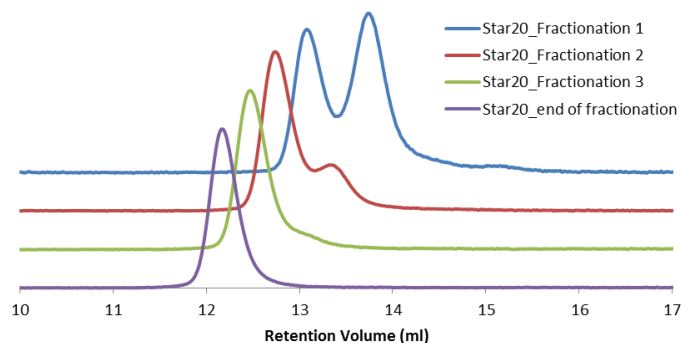
Figure 4.23 SEC chromatograms (RI detector) of the Star20 polymer mixtures from the starting crude material to the final 'pure' star after being processed through three fractionations.
