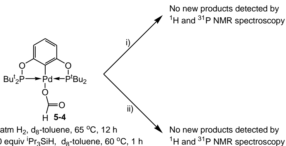
Scheme 5.12: Attempted further reactivity of the complex [Pd(OC(H)O)(\kappa^3\text{-P,C,P-4-1})] ( 5-4 ).
