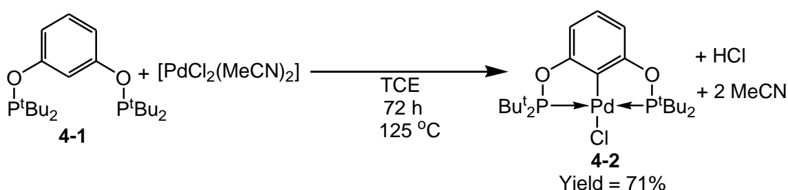
Scheme 4.5: Synthesis of [PdCl(\kappa^3\text{-P,C,P-4-1})] ( 4-2 ).
