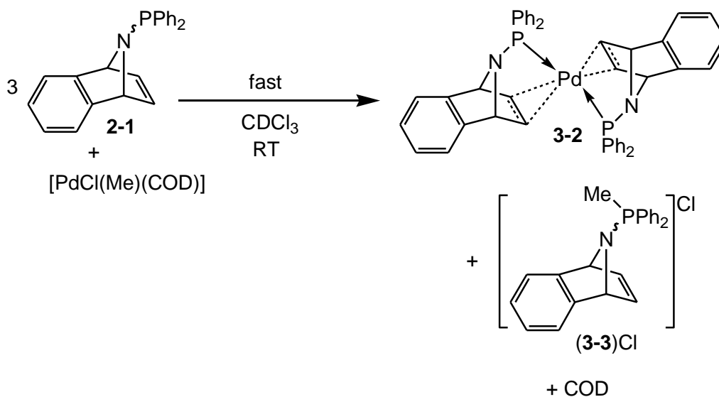
Scheme 3.21: Reaction between three equivalents of 2-1 and [\text{PdCl}(\text{Me})(\text{COD})] .
