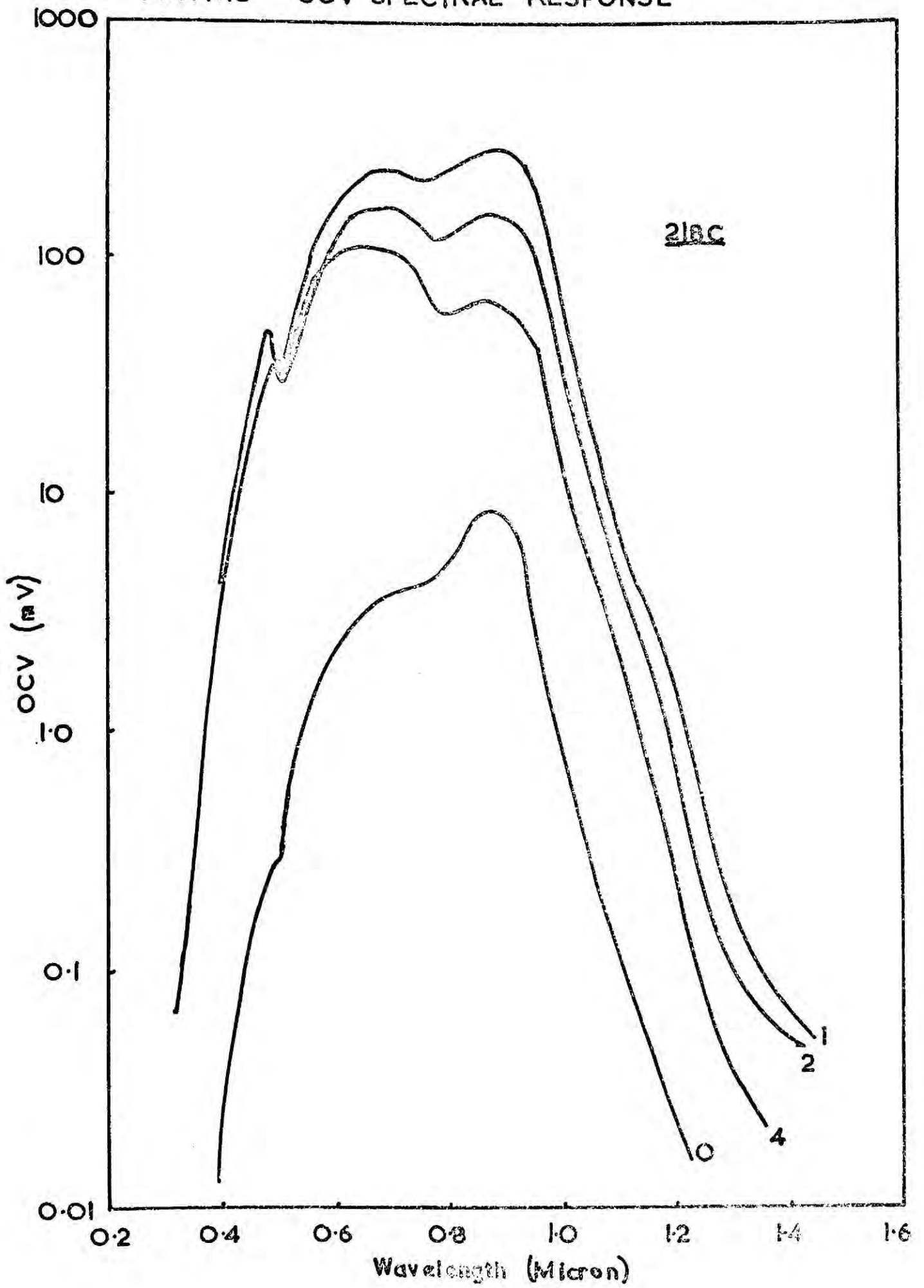
FIG. 7.13 OCV SPECTRAL RESPONSE
