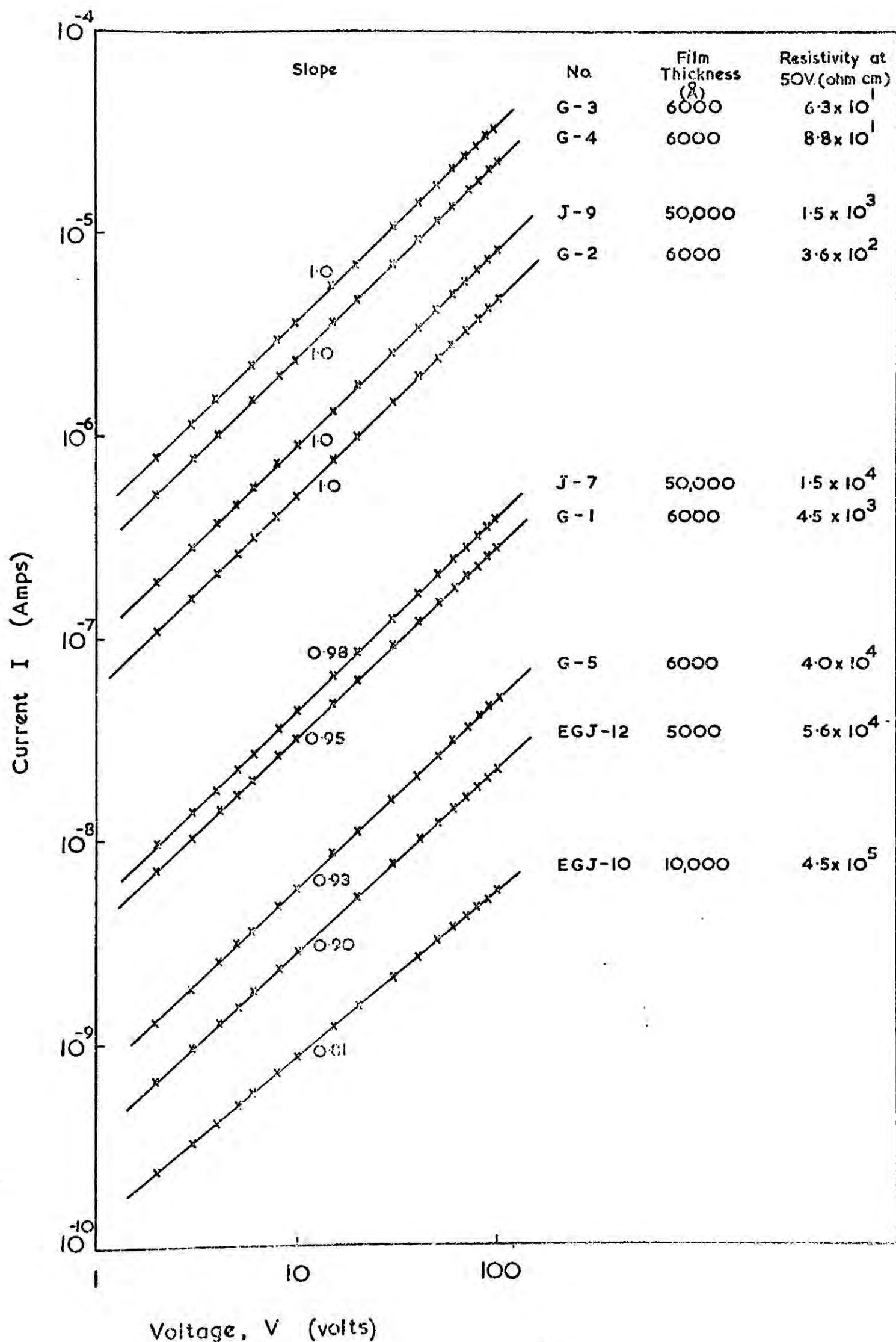
FIG. 6-3 Dark I (V) characteristics of polycrystalline CdS films on glass
