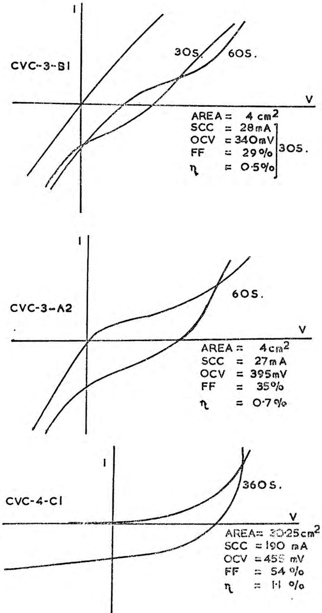
FIG. 7.7 I(V) FOR POOR THIN FILM CELLS
