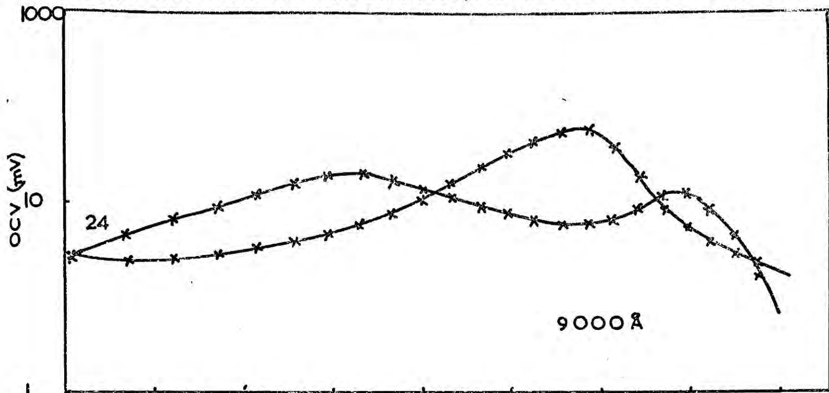
FIG. 7.16 OCV VERSUS TEMPERATURE, MONOCHROMATIC ILLUMINATION
