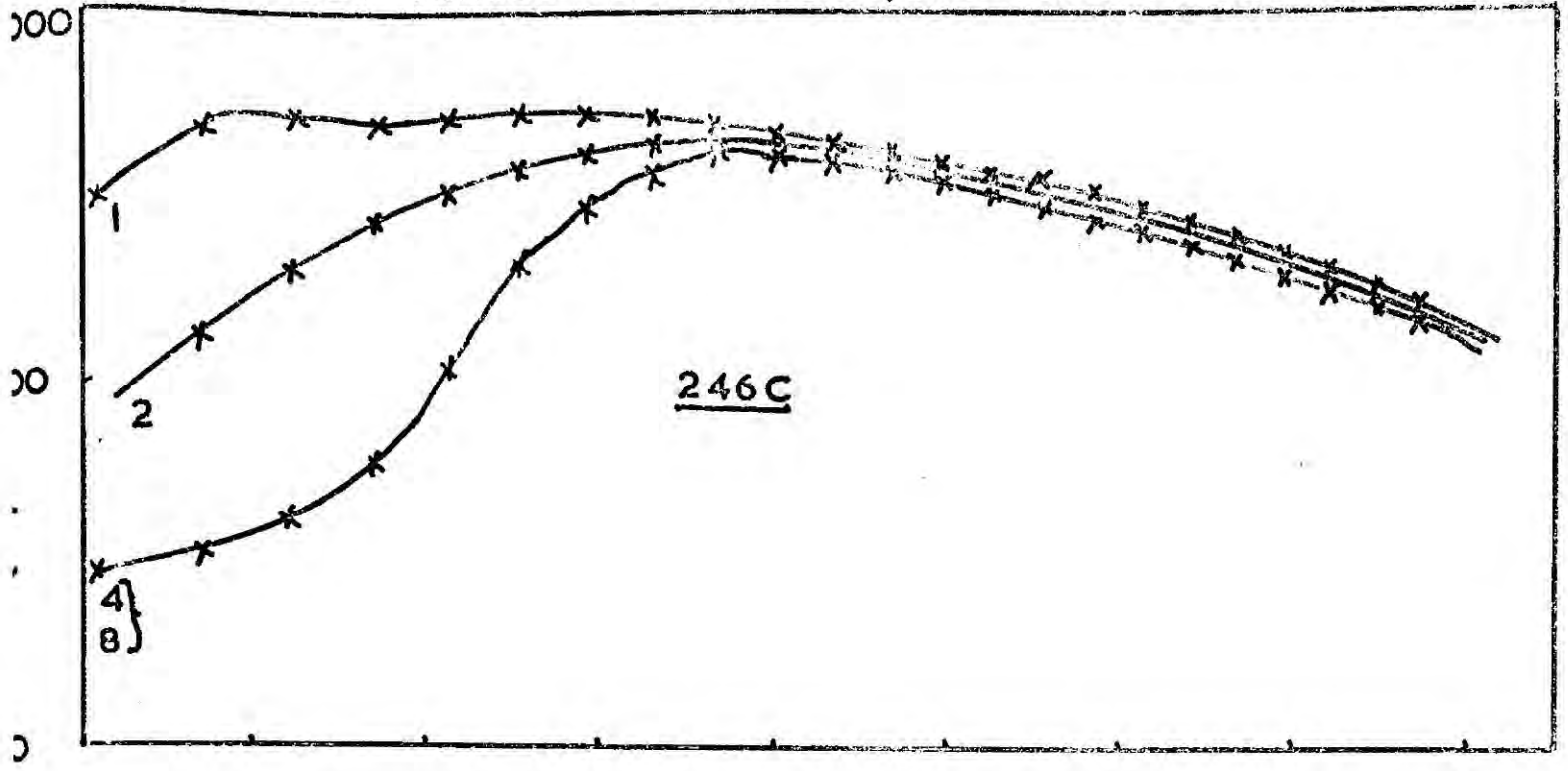
FIG. 7.15 OCV VERSUS TEMPERATURE, 1000 SUNLIGHT ILLUMINATION
