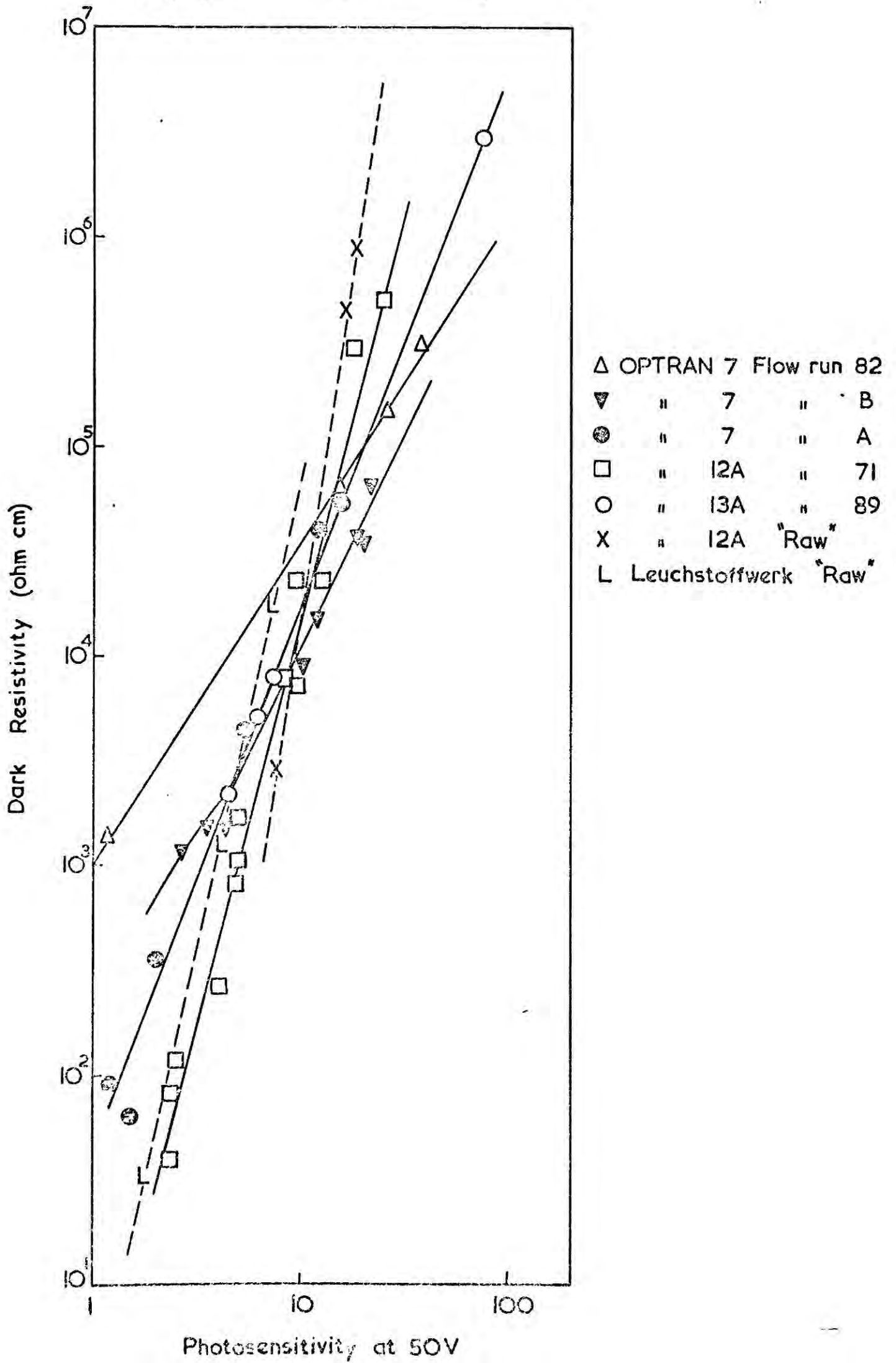
FIG.6-11 Relation between Dark Resistivity and Photosensitivity of polycrystalline CdS films on glass.
