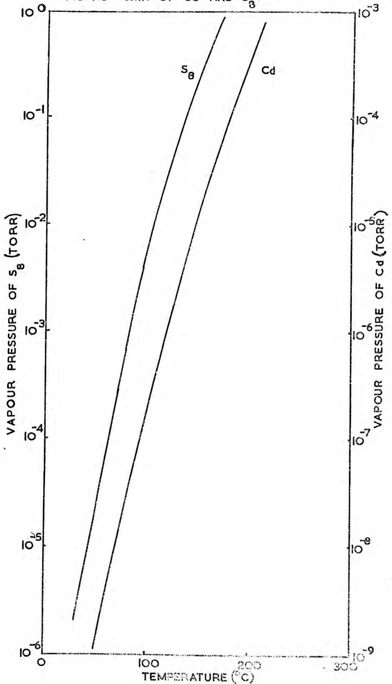
FIG. 9.5 S.V.P. OF Cd AND S 8 .
