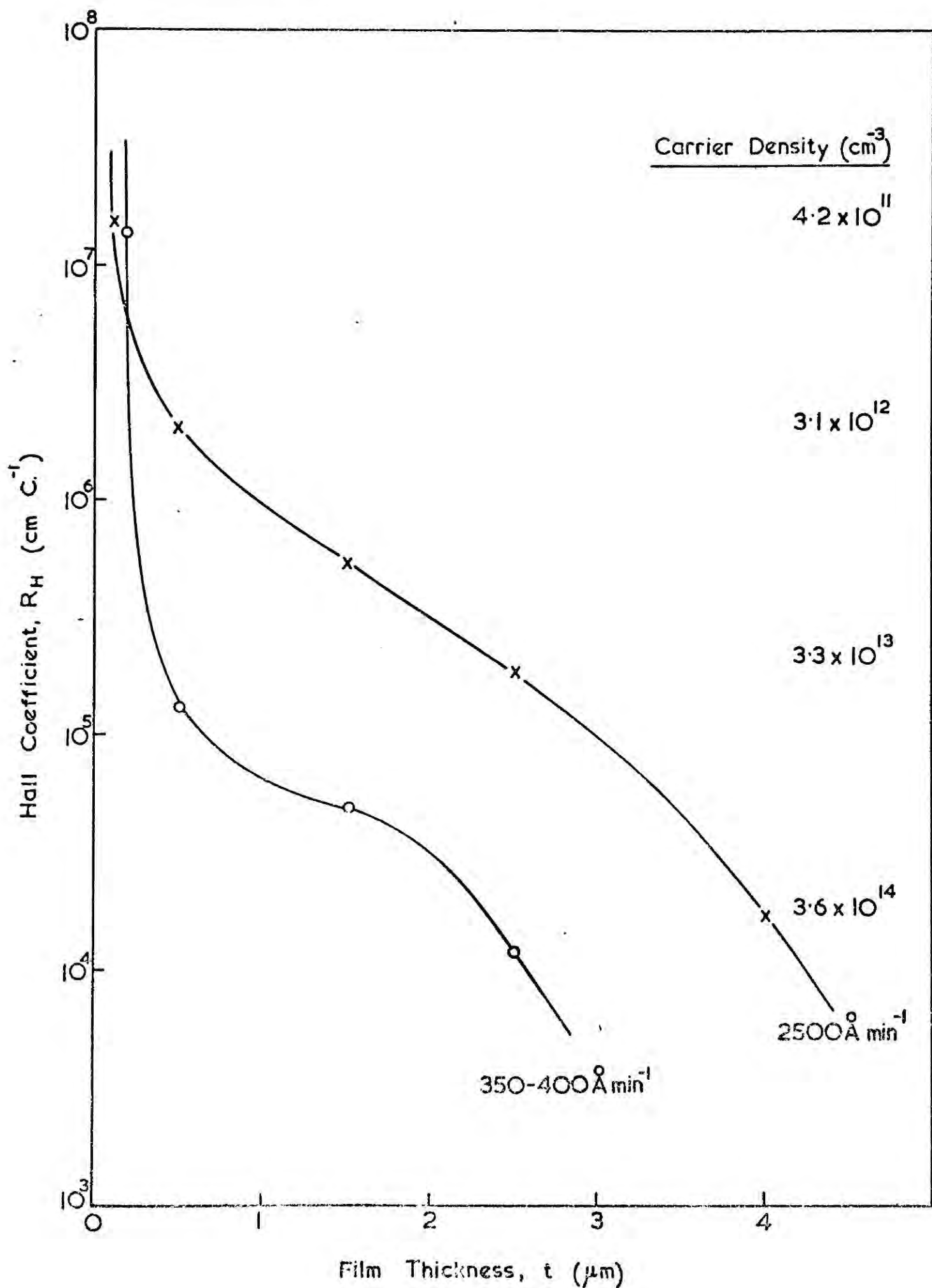
Fig.6.10 Hall coefficient size effect of CdS polycrystalline films on glass.
