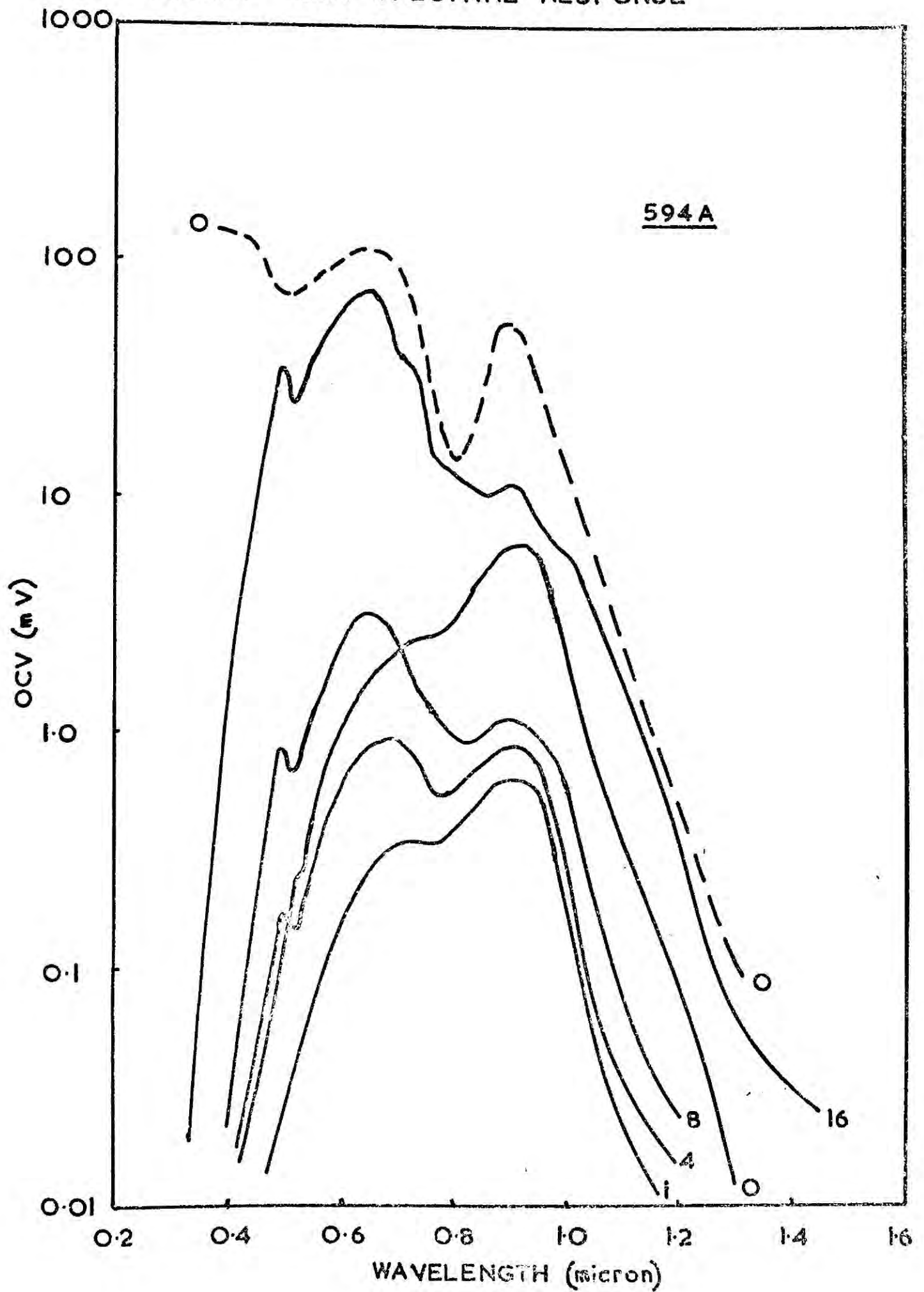
FIG. 7.11 OCV SPECTRAL RESPONSE
