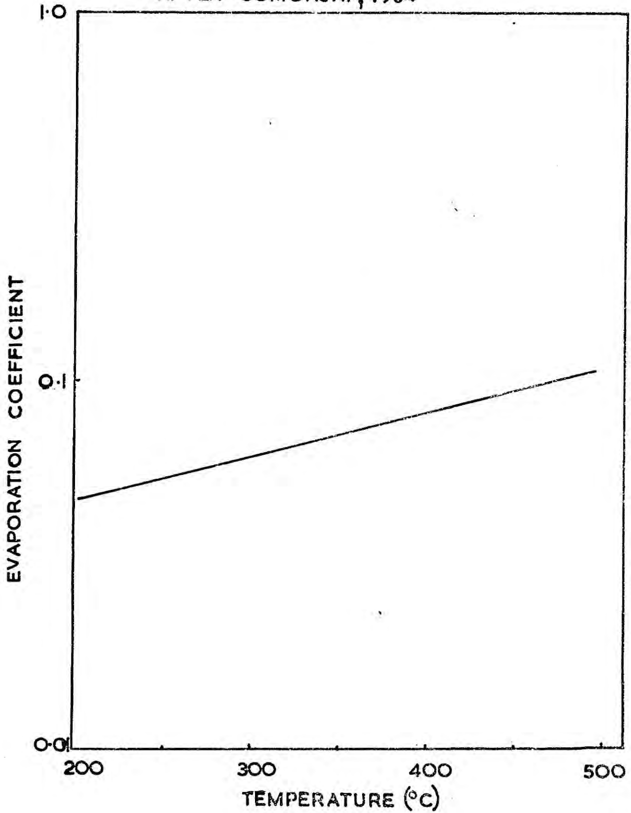
FIG.9.4 EVAPORATION COEFFICIENT OF CdS, AFTER SOMORJAI, 1964
