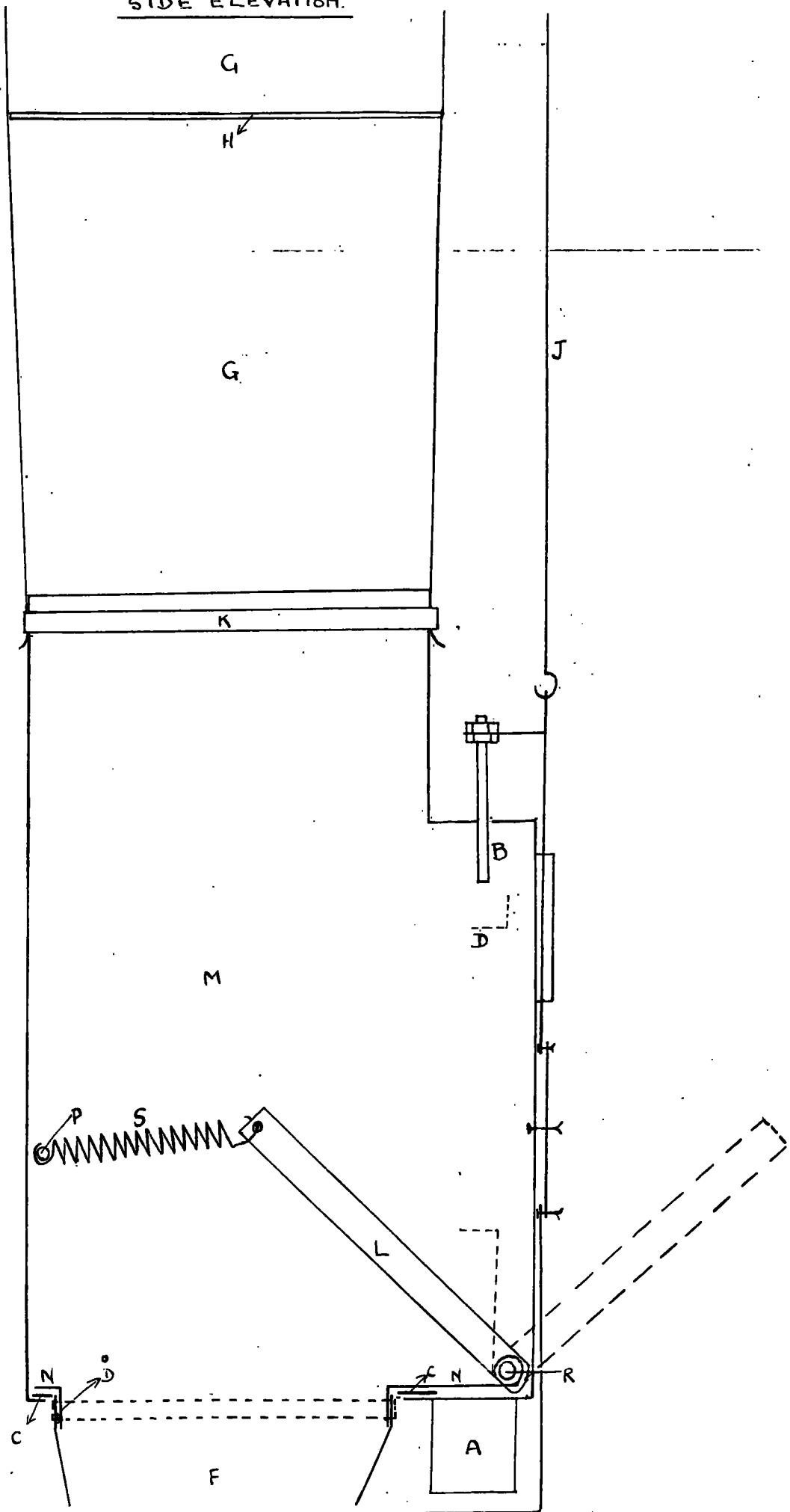
SIDE ELEVATION.
