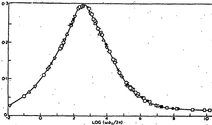
FIG. 2. Master curve for \epsilon'_r versus \log_{10} \omega b \tau / 2\pi T_0 = 273^\circ\text{K} . Mix C
