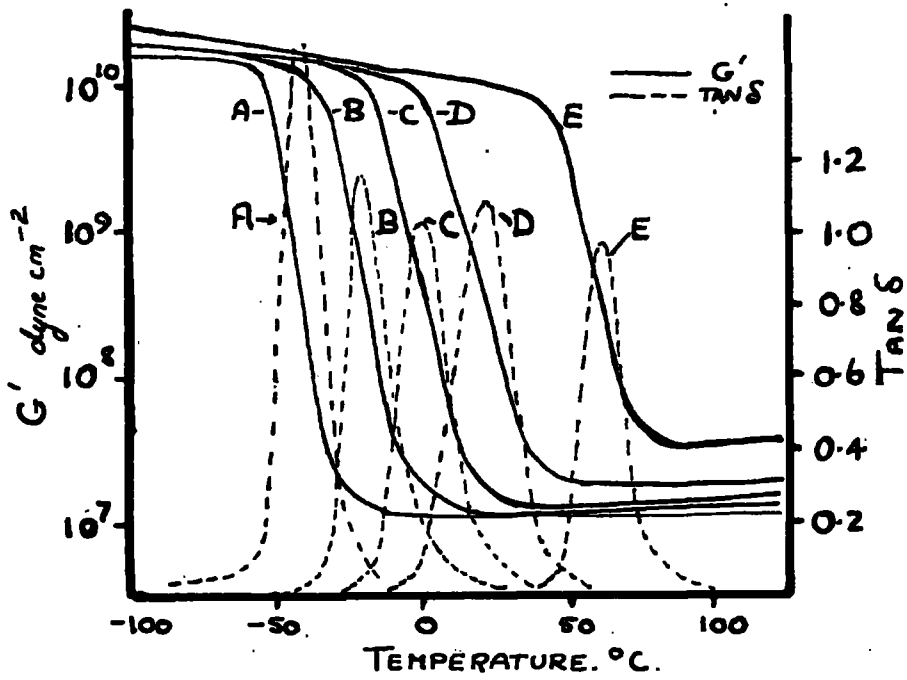
FIG 2.22 Effect of amount of combined sulphur on temperature variation of modulus ( G' ) and \tan \delta . A, 5%; B, 10%; C, 15%; D, 20%; E, 30% sulphur calculated on raw rubber (Data from Schmieder and Wolf, 1953)
