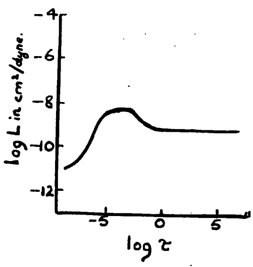
FIG 2-12 Retardation Spectrum plotted logarithmically Lightly vulcanised NR at 25°C
