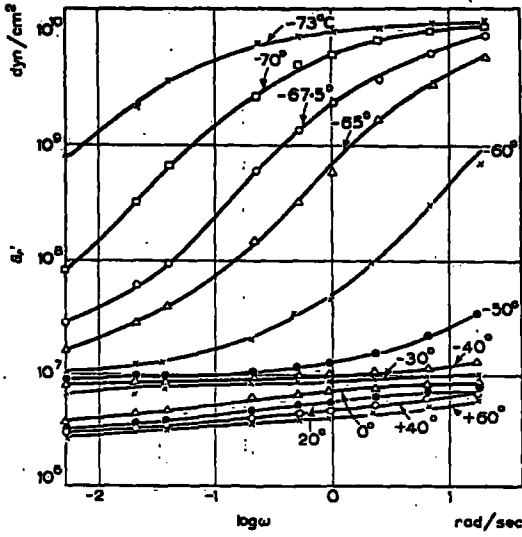
FIG. 1. Reduced modulus G_r' of unvulcanized natural rubber. T_0 = 273^\circ\text{K} .
