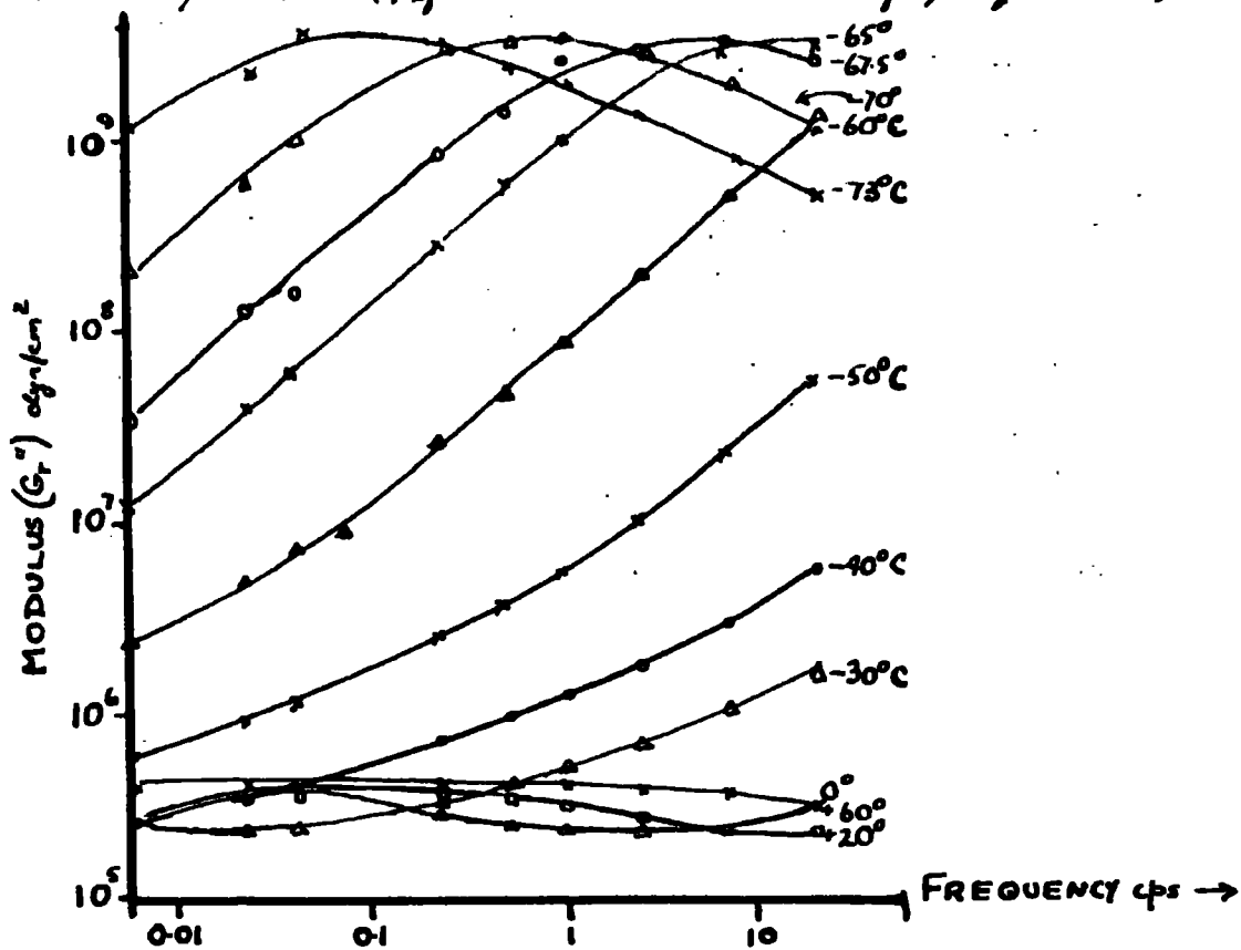
FIG 2-17 a Reduced in-phase modulus ( G_r' ) for unvulcanized natural rubber - frequency curve (Payne, 1925)
