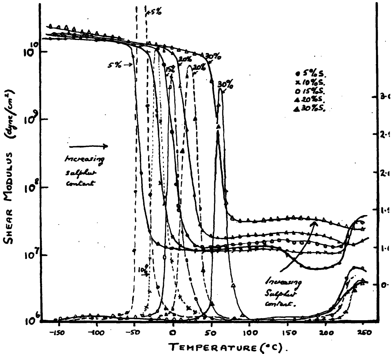
FIG 2.25. Shear modulus and damping decrement - temperature function with increasing amounts of sulphur content (Schrieder and Wolf,
