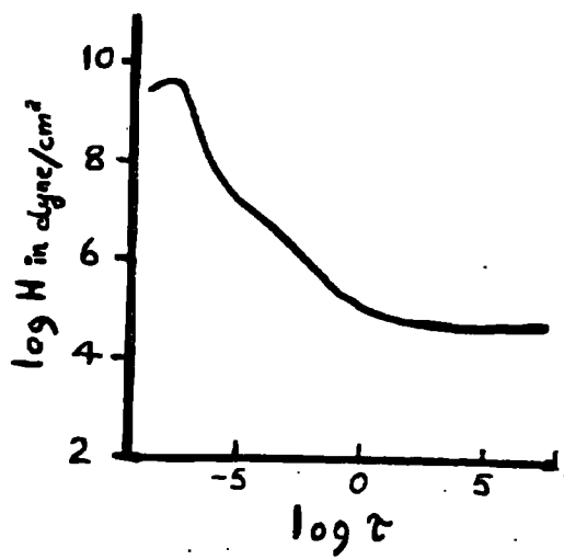
FIG 2-11 Relaxation Spectrum plotted logarithmically. Lightly vulcanised NR at 25°C
