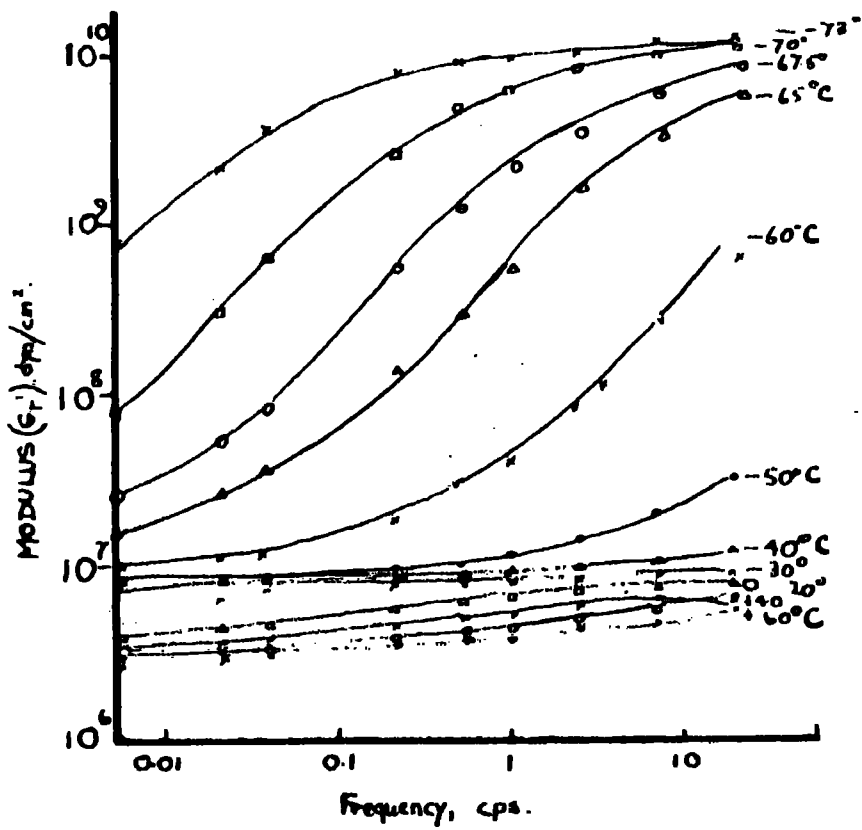
FIG 2-17 a Reduced in-phase modulus ( G_r' ) for unvulcanized natural rubber - frequency curve (Payne, 1925)
