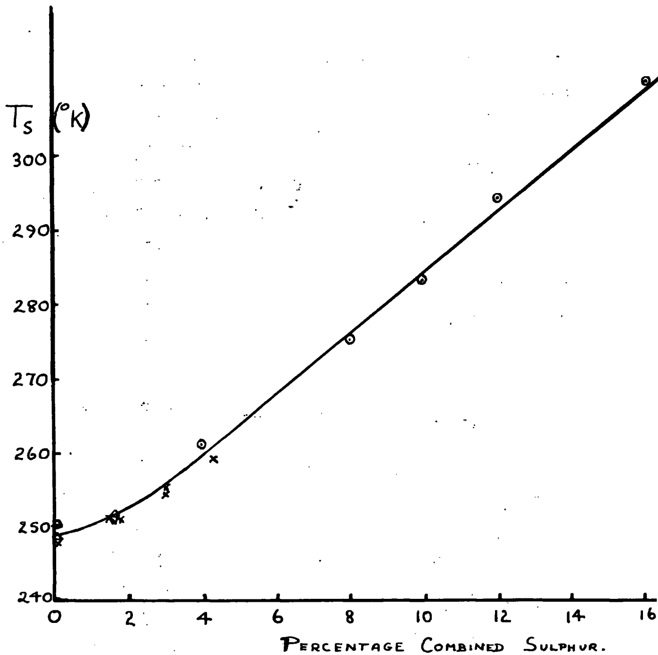
FIG 3.18. Relationship between T_g and combined sulphur content. x, dielectric results (dielectric - Norman and Payne) o dielectric results; derived by Payne (1958) from data of Scott, Curtis and McPherson (1933). Δ; dynamic mechanical results from three papers. Zapas, Sleyfer and de Witt (1955), Fletcher and Gent (1957), Payne (1958), ∇ dynamic mechanical results Payne (1958).
