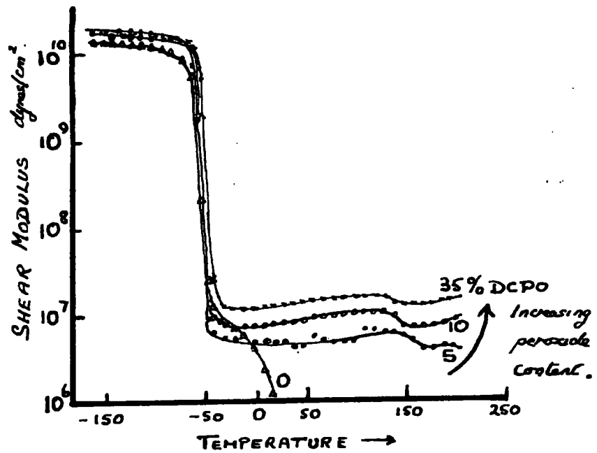
FIG 2-26. Shear modulus, G , of dicumyl peroxide cured natural rubber as a function of temperature. (Heimze, Schrieber, Schell and W. 1961).
