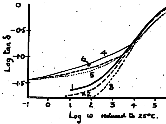
Fig 2-35. Loss tangents of the six vulcanizates, plotted logarithmically against radian frequency reduced to 25°. (Stollon and Ferry).
