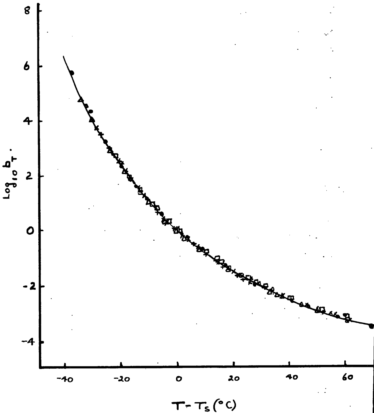
FIG 3-10, \text{Log } b_T values. \bullet Unvulcanized. \Delta A2. \square A4 \times A6, + B3, — \log b_T = -8.86(T - T_s) / (101.6 + T) Payne (1958a).
