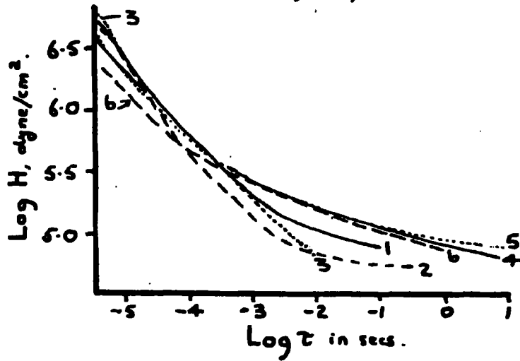
FIG 2.33. Relaxation spectra of six vulcanisates, mean of calculations from J' and J'' , reduced to 25^{\circ}\text{C} . (Stratton and Ferry). See Table 2.3 for details of the vulcanisates 1, 2 and 3 sulphur vulcanisates. 4, 5 and 6 refer to rubbers not cross linked by sulphur.
