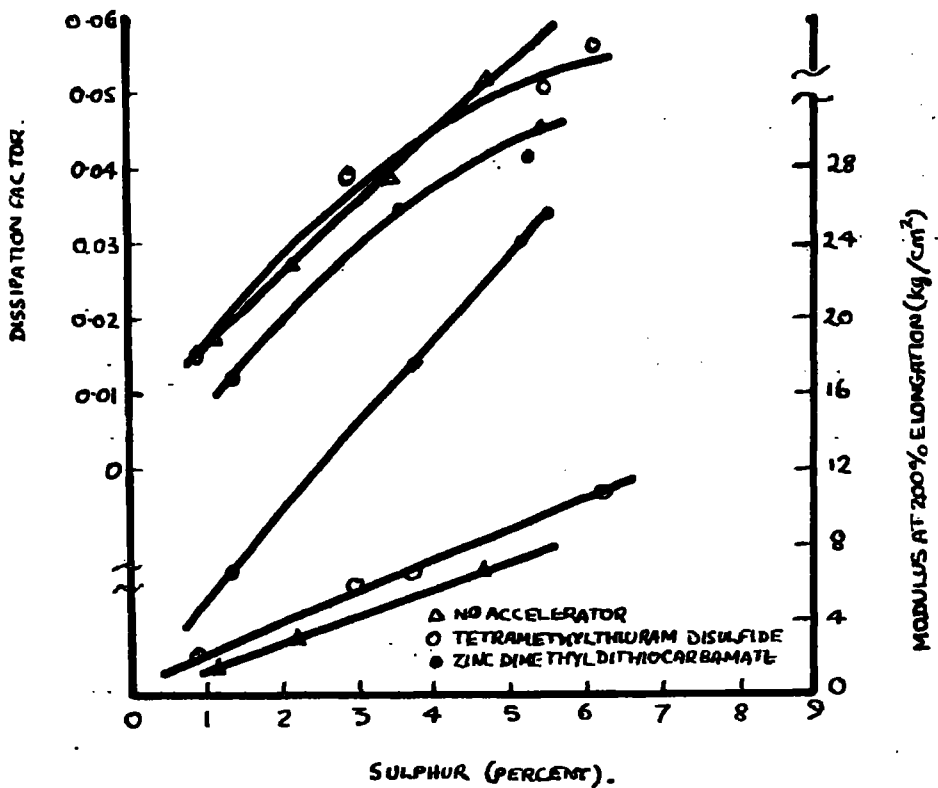
FIG 3-5. Variation of dissipation factor and modulus of soft rubber vulcanisates with per cent of combined sulphur, showing the effect of zinc. (Schabramach 1957).
