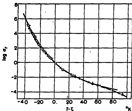
FIG. 11. (T - T_g) versus (\text{Log}_{10} a_T) The solid line shown is the empirical curve described by Eq. (12).
