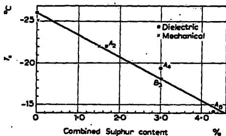
FIG. 10. T_g values as a function of combined sulphur content in natural rubber. The T_g values have been obtained from dielectric and mechanical measurements on unvulcanized and vulcanized natural rubbers.
