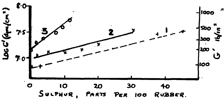
FIG 2.23 Effect of combined sulphur on in-phase modulus ( G' ). Curve 1: natural rubber (data from Table 2.1); 2: natural rubber (Schmieder and Wolf, 1953); 3: butadiene-styrene rubber (Payne 1959).
