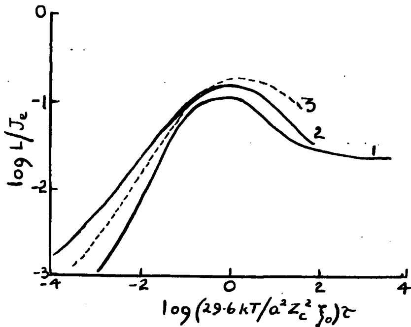
Fig 2.36. Retardation spectra of cross-linked systems, near their maxima, reduced to corresponding states by equations 2.50 and 2.5. Curve 1: natural rubber, 2; polyurethane rubber, 3; 40% polyvinyl chloride in dimethyl thianthrene. (Ferry, 1961).
