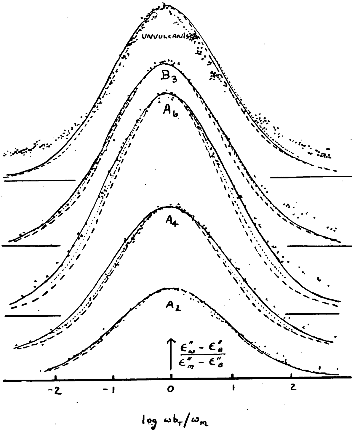
FIG 3-15: Comparison of experimental results with analytic functions (2). ——— Wagner and Yagel - - - - Kirkwood and Fuoss (1). ..... Kirkwood and Fuoss (2).
