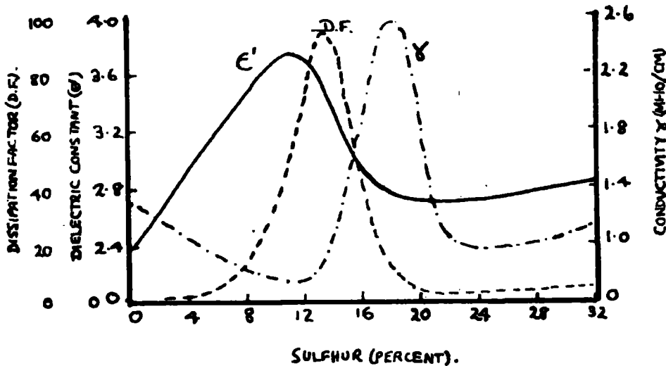
FIG 3-2. Variation of dielectric constant, dissipation factor, and conductivity of rubber-sulphur vulcanisates with sulphur content. Measurements at 1000 cps 25°C. (Scott, MacPherson and Curtis 1923. MacPherson 1963)
