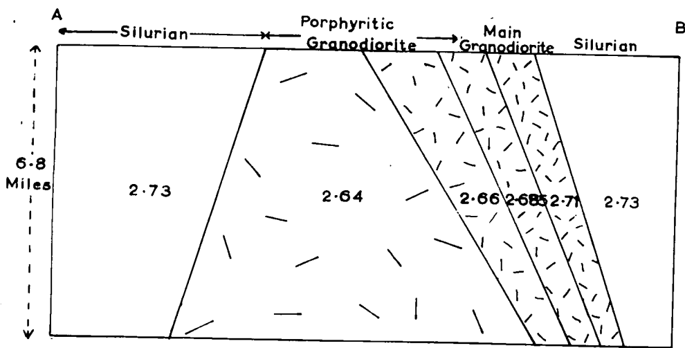
Fig.6.4 Comparison of the anomaly due to the two dimensional model shown above with the observed anomaly over the granite (The dimensions of the model are based upon fig. 2, page 322 of Bott & Masson-Smith (1960))
