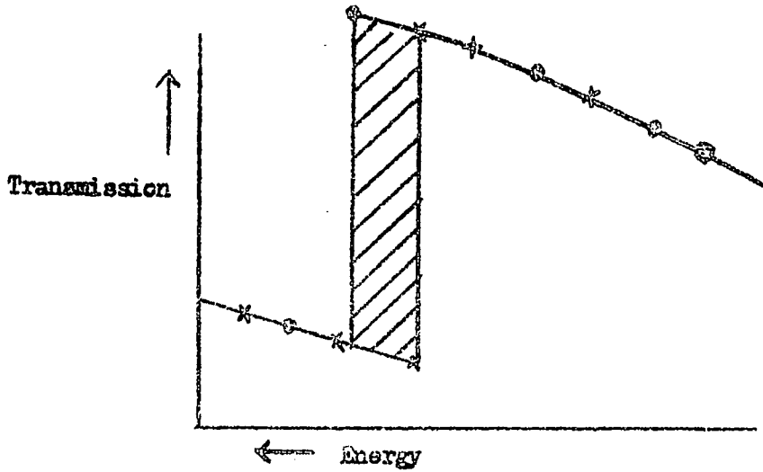
Fig. 1-5 Transmission of filters when they are made balanced The shaded portion represents the intensities of the selected radiations
