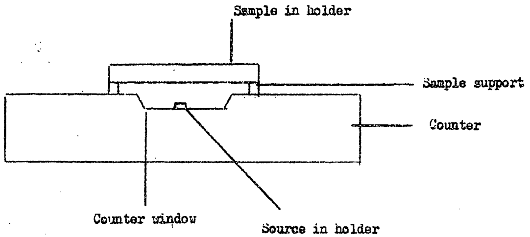
Fig. 1-3 Geometrical arrangement
