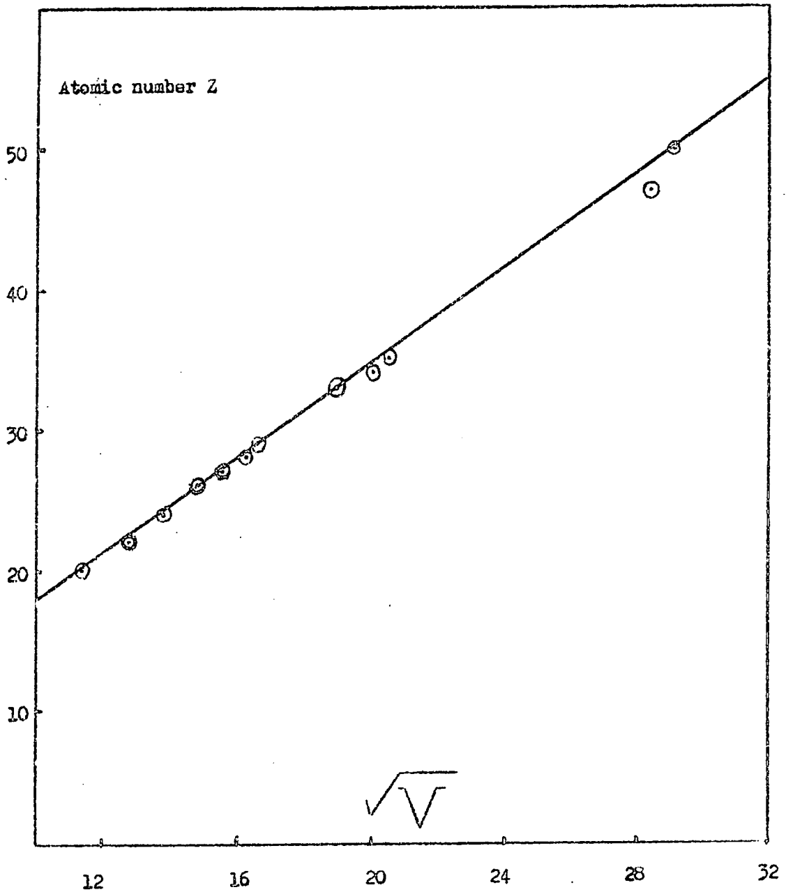
Fig. 3-8 Atomic number Z against square root of mean amplitude of pulses produced by K \lambda -rays (after correction for attenuation)
