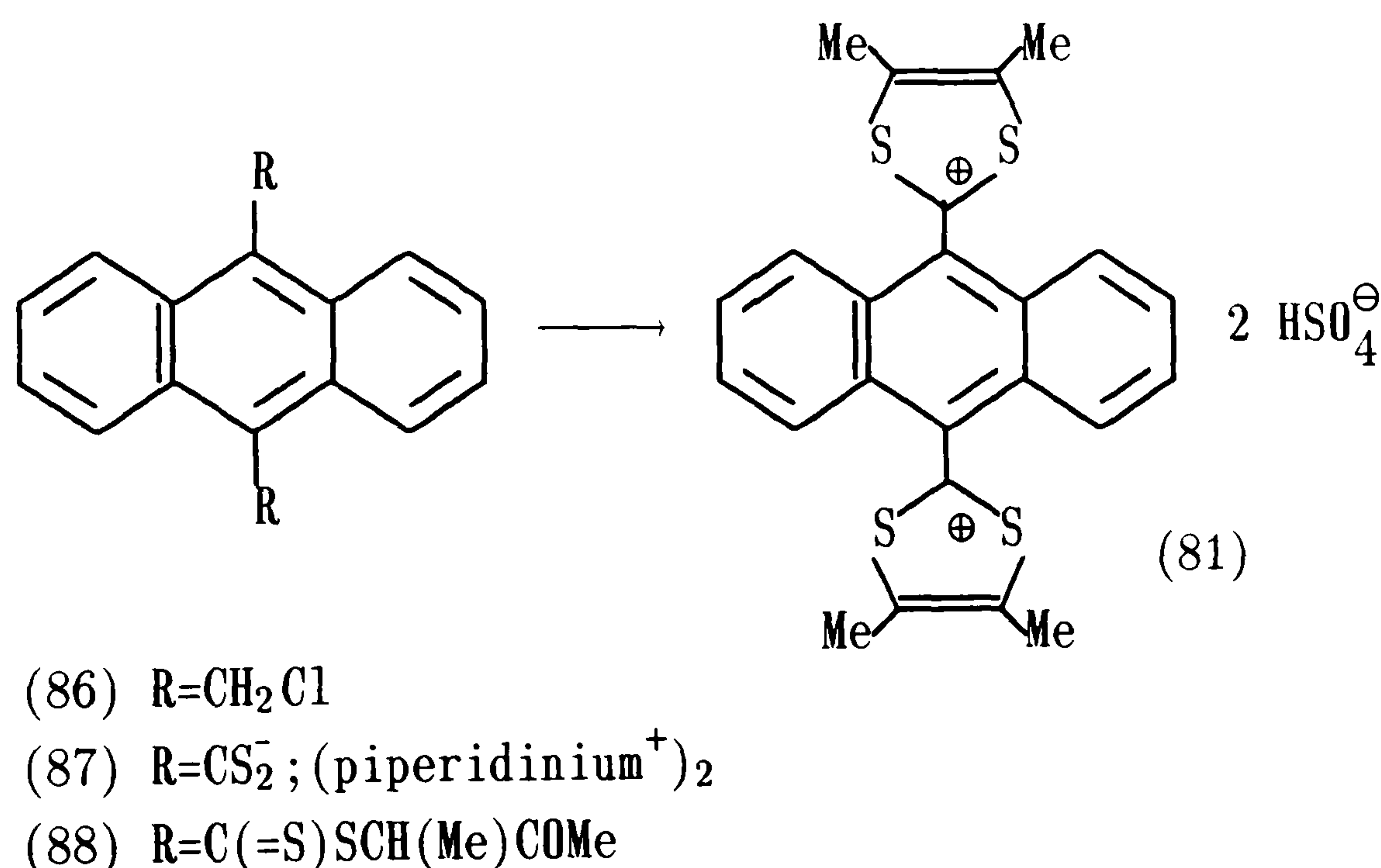
Scheme 2.8: Reagents: As for Scheme 2.7; overall yield = 42%
