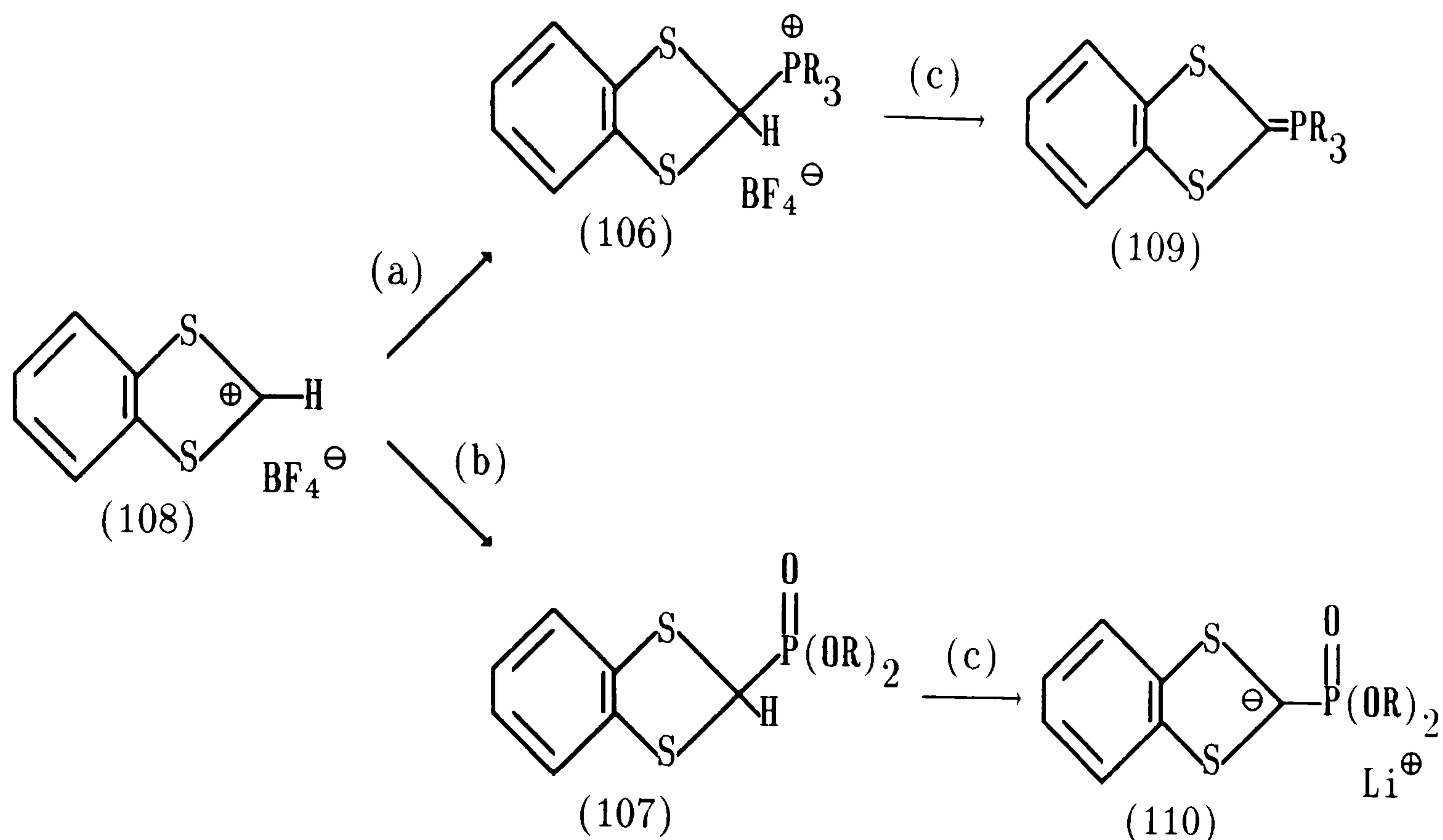
Scheme 2.12: Reagents: (a) \text{PR}_3 ; (b) \text{P(OR)}_3 , \text{NaI} ; (c) n\text{-BuLi} .
