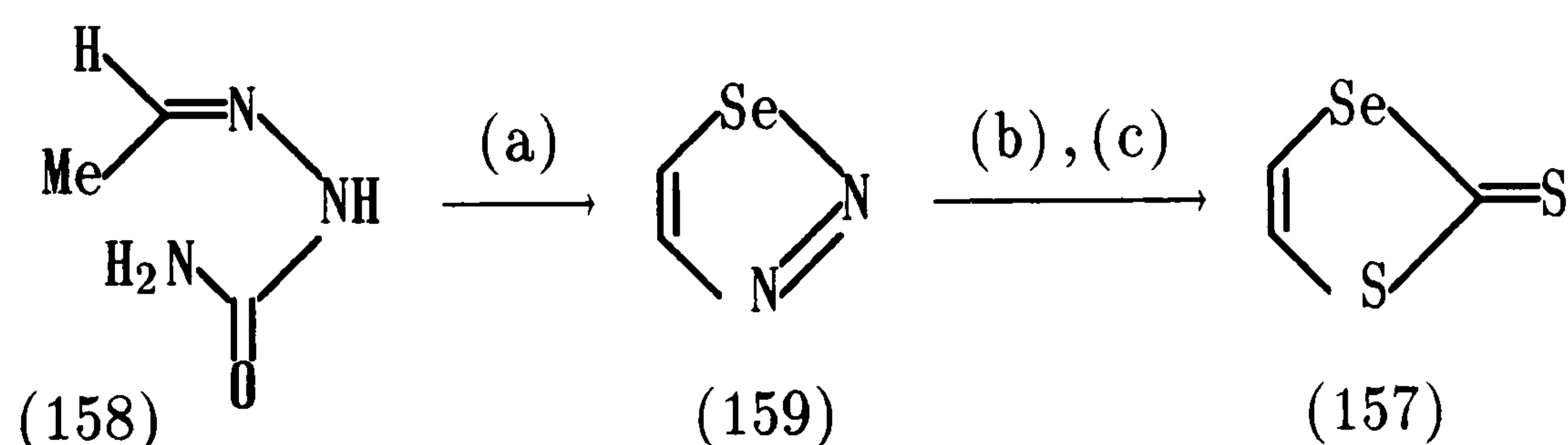
Scheme 3.2: Reagents: (a) SeO 2 ; (b) t -BuOH/DMF/CS 2 ; (c) HCl.
