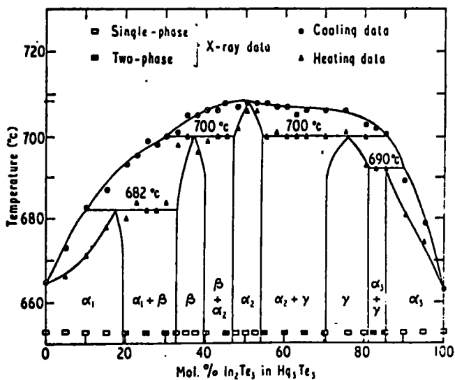
Phase diagram of the Hg_3Te_3-In_2Te_3 alloy system.
