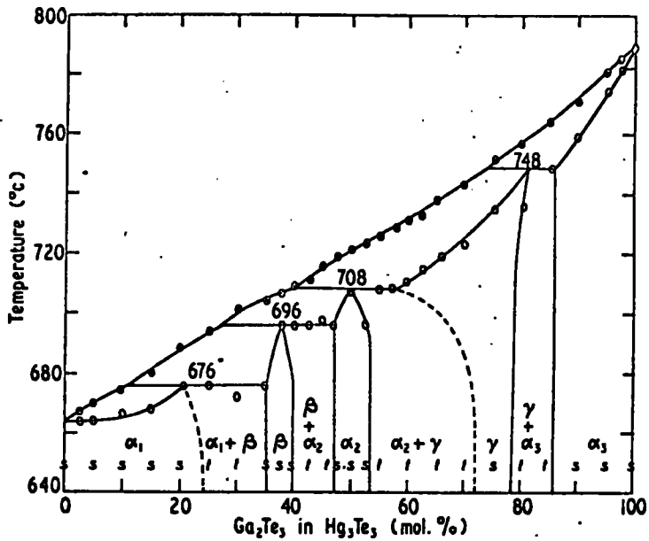
Equilibrium diagram of Hg_3Te_3-Ga_2Te_3
