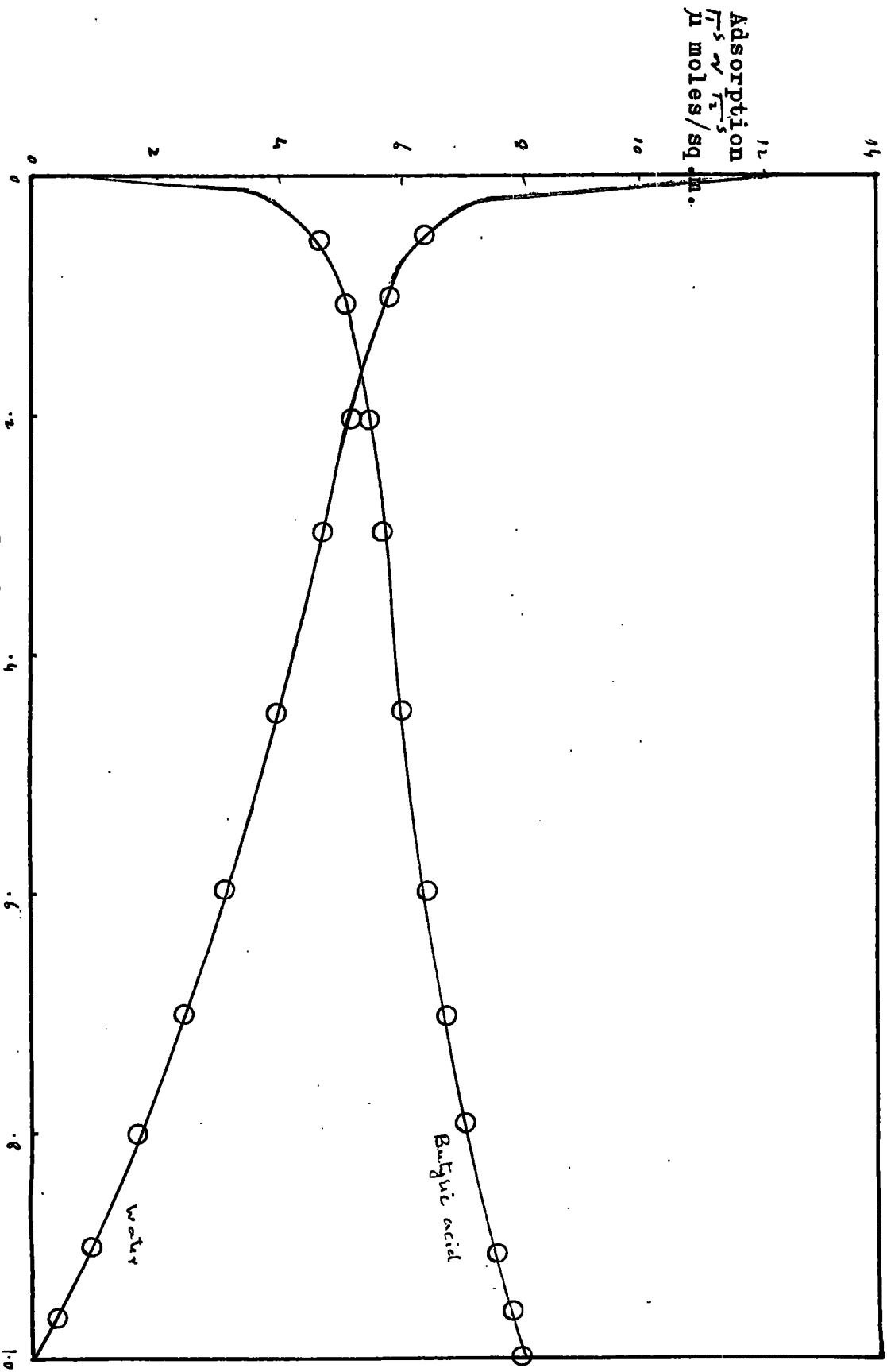
Fig. 57- Individual isotherms for adsorption of butyric acid and water at 30 C with the major axes of both molecules perpendicular to the surface.
